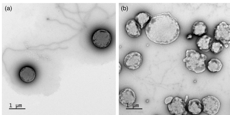
Fig. 1. (a, b) Negative stain transmission electron microscopy of strain M1 T . Microscope images of the cellular periphery of strain M1 T cells imaged at different magnifications.
