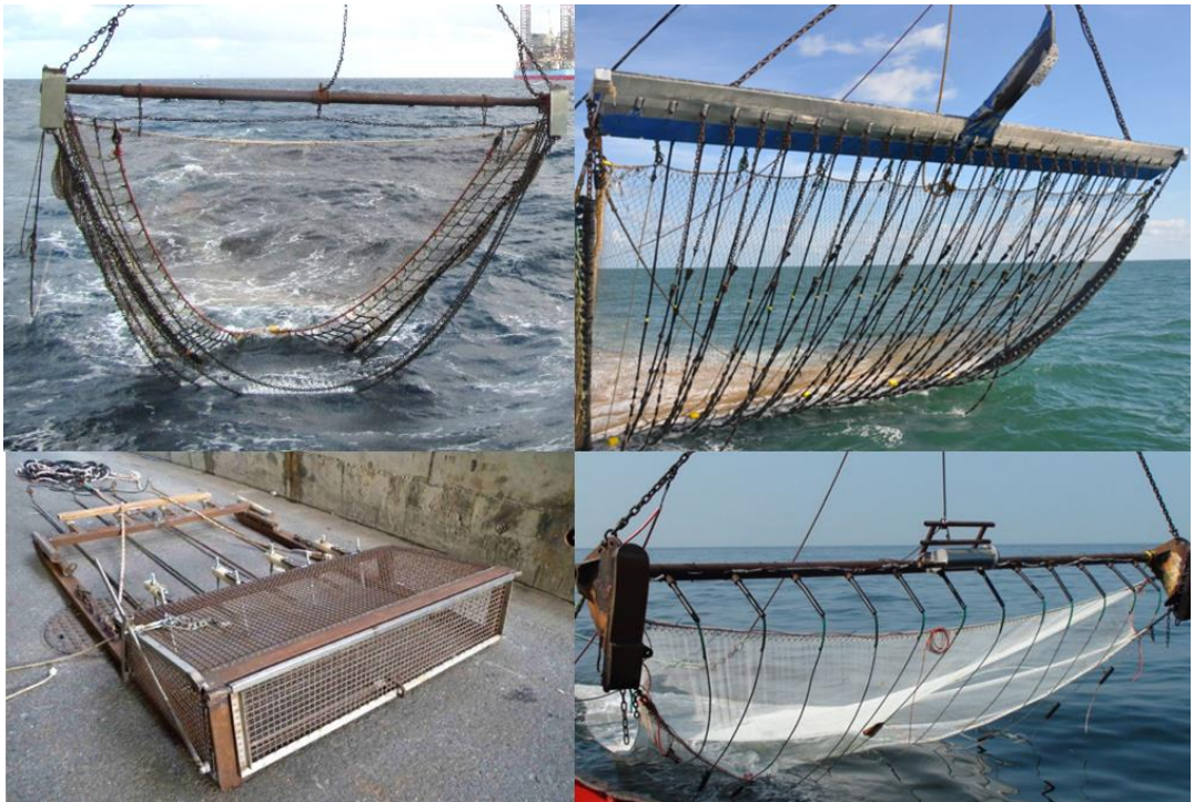
Figure 2. Comparison between a traditional tickler chain rigged beam trawl (top left) and an electric PulseWing trawl (top right) which are both used to fish for North Sea dover sole ( Solea solea ). Electrodes and gear used to stimulate and catch razor clams, Ensis spp. (bottom left) and a ‘Hovercran’ electric trawler used to catch brown shrimp, Crangon crangon (bottom right).
