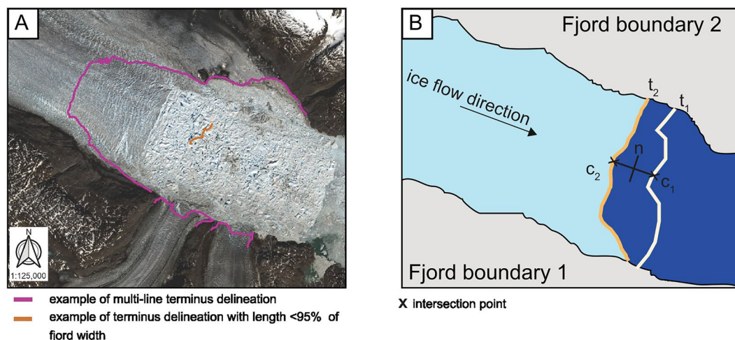
Fig. 3 Terminus delineation filtering. (A) Examples of terminus delineations with more than one line segment (pink) and with a length shorter than 95% of the fjord width (orange), which are excluded from the dataset. (B) Schematic showing how advance and retreat are determined. The normal ( n ) to the line connecting the intersection points ( c_1 and c_2 ) of successive terminus delineations ( t_1 and t_2 ) is used to determine advance and retreat of the glacier. In the sketch shown here, c_2 is up-fjord of the normal n , therefore the glacier has retreated. This classification of advance/retreat is solely used for filtering purposes.
