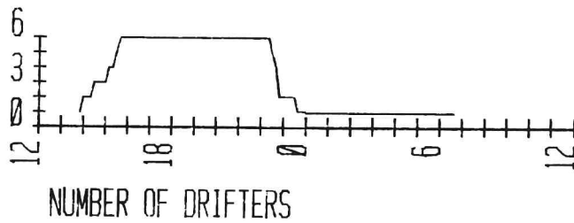
Fig. 5. 19 and 20 May 1980. Number of drifters.
