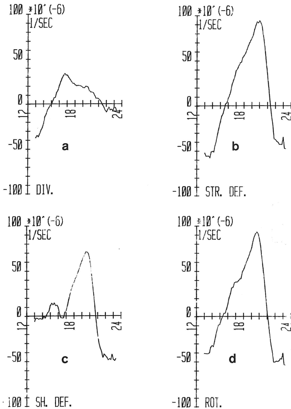
Fig. 88. 19 and 20 may 1980. Current meters 2, 3 and 4. a) Divergence. b) Stretching deformation. c) Shearing deformation. d) Vorticity.
