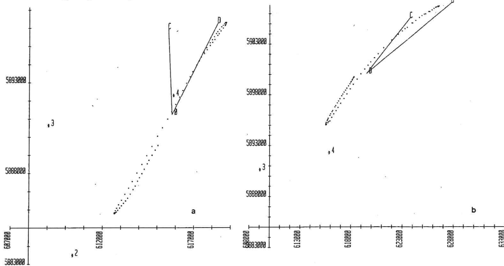
Fig. 102. Current meters interpolation vector C, calculated at the real drifter path, and Lagrangian vector D, plotted at the centroid of a part of the drifter trajectory. a) 16 and 17 june 1980. Current meters 2, 3 and 4. Drifter 0. From 16 june, 14.20 h till 17 june, 02.50 h, 750 minutes. b) 23 and 24 june 1980. Current meters 3, 4 and 5. Drifter 0. From 23 june, 18.50 h till 24 june, 07.20 h, 750 minutes.
