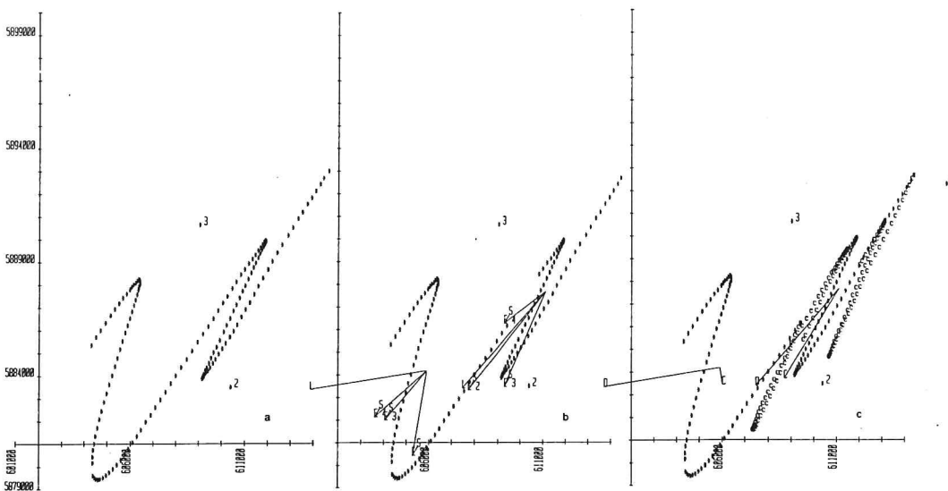
Fig. 44. 21 and 22 may 1980. Drifter 5.
