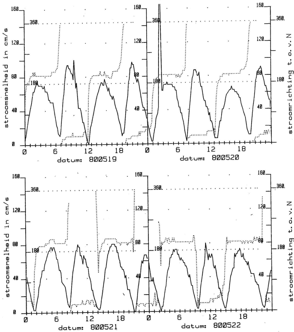
Fig. 80. 19, 20, 21 and 22 may 1980. Current meter 2. Current speed (solid curve) and direction (dashed curve).
