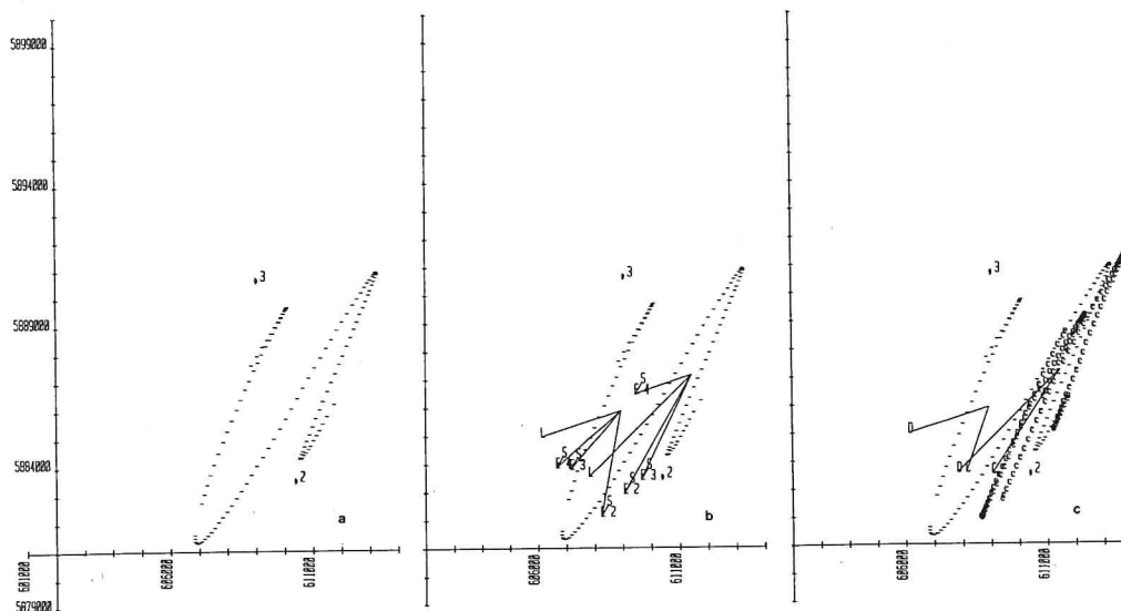
Fig. 42. 21 and 22 may 1980. Drifter 3.
