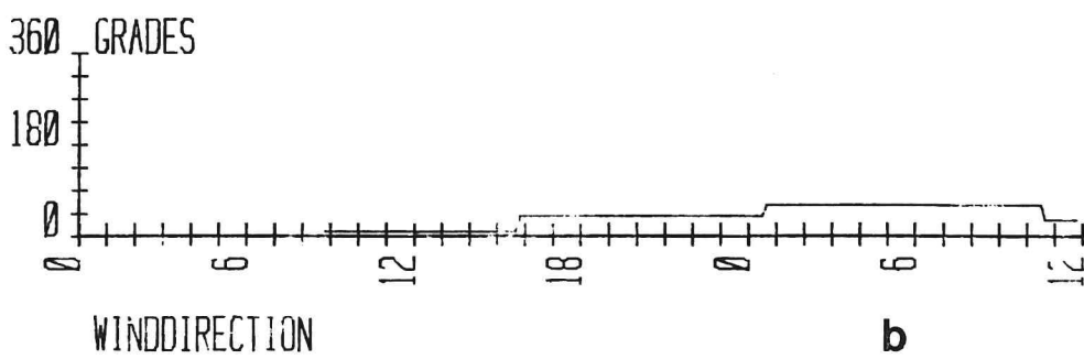
Fig. 21. 20 and 21 may 1980. a) Wind velocity. b) Wind direction.
