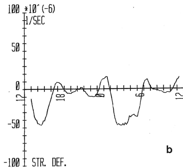
Fig. 95. 23 and 24 June 1980. Current meters 3, 4 and 5. a) Divergence. b) Stretching deformation.
