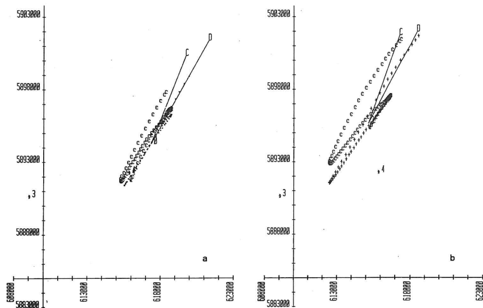
Fig. 97. 16 and 17 june 1980. Drifters 0 and 2.
