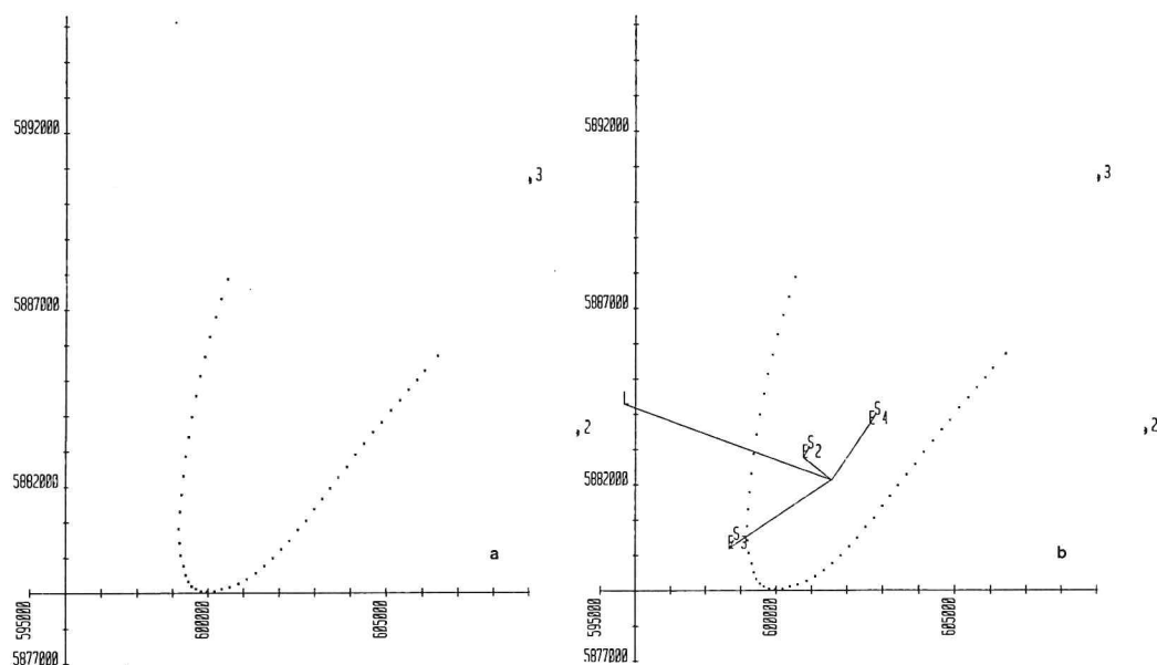
Fig. 9. 19 and 20 may 1980. Drifter 0.
