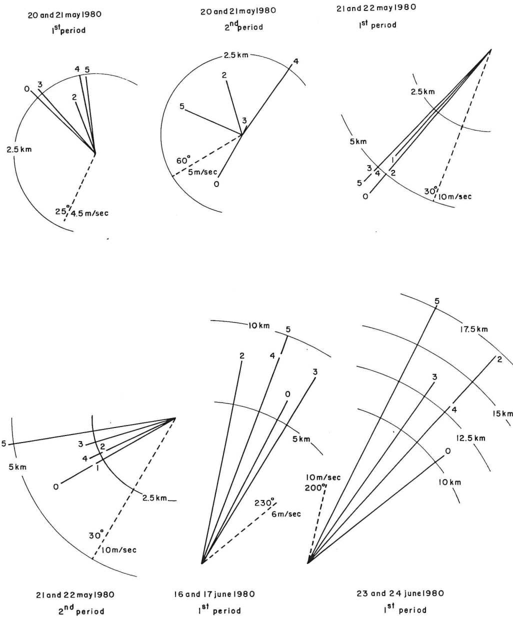
Fig. 103. Residual velocity and wind characteristics.
