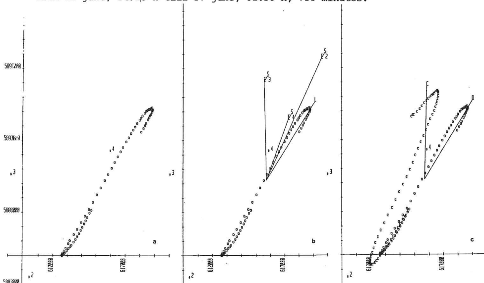
Fig. 55. 16 and 17 June 1980. Drifter 1.
