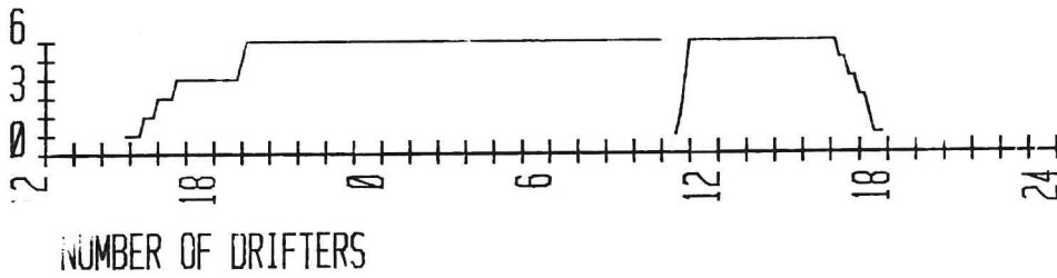
Fig. 35. 21 and 22 may 1980. Number of drifters.
