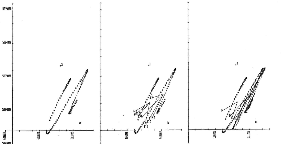
Fig. 40. 21 and 22 may 1980. Drifter 1.
