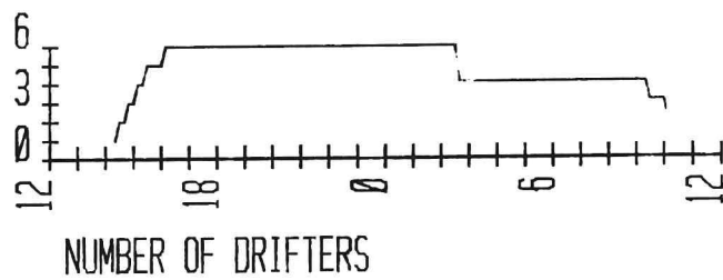
Fig. 50. 16 and 17 june 1980. Number of drifters.
