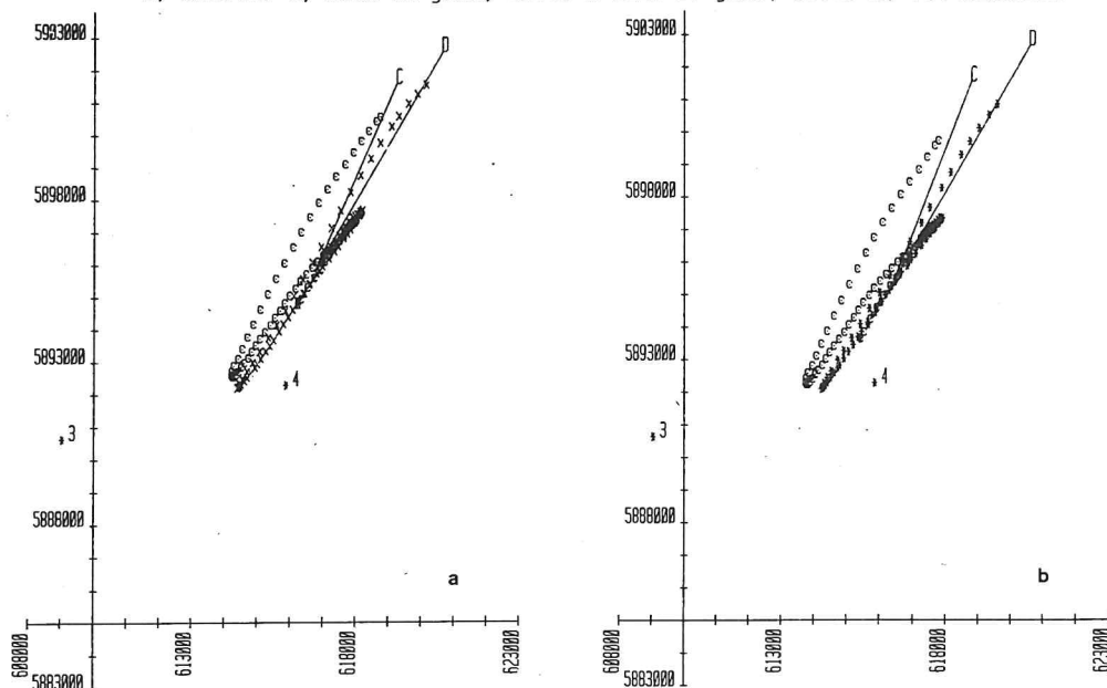
Fig. 98. 16 and 17 june 1980. Drifters 4 and 5.
