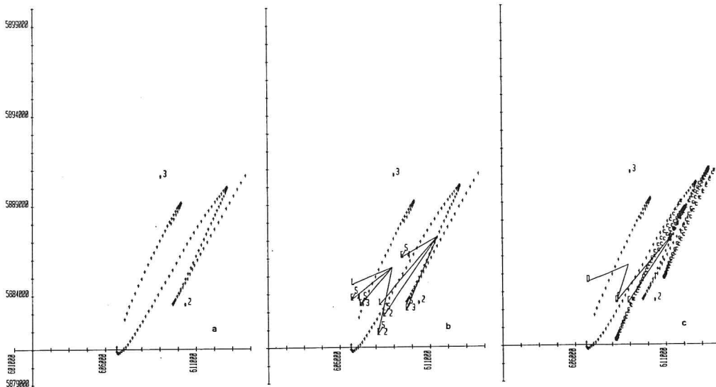
Fig. 41. 21 and 22 may 1980. Drifter 2.
