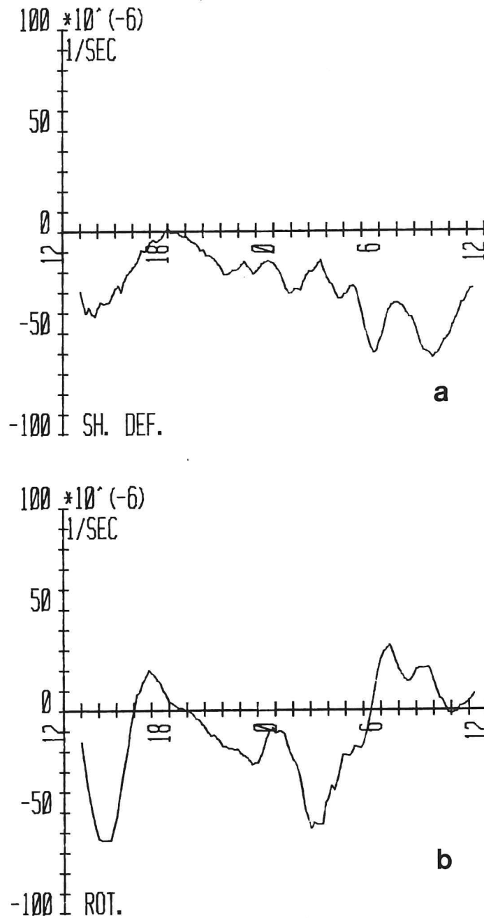
Fig. 96. 23 and 24 June 1980. Current meters 3, 4 and 5. a) Shearing deformation. b) Vorticity.
