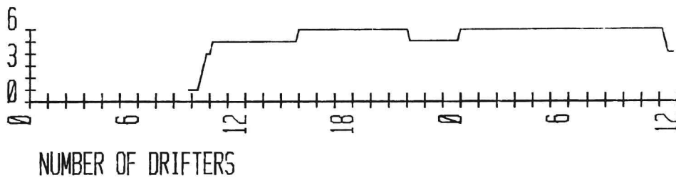
Fig. 20. 20 and 21 May 1980. Number of drifters.
