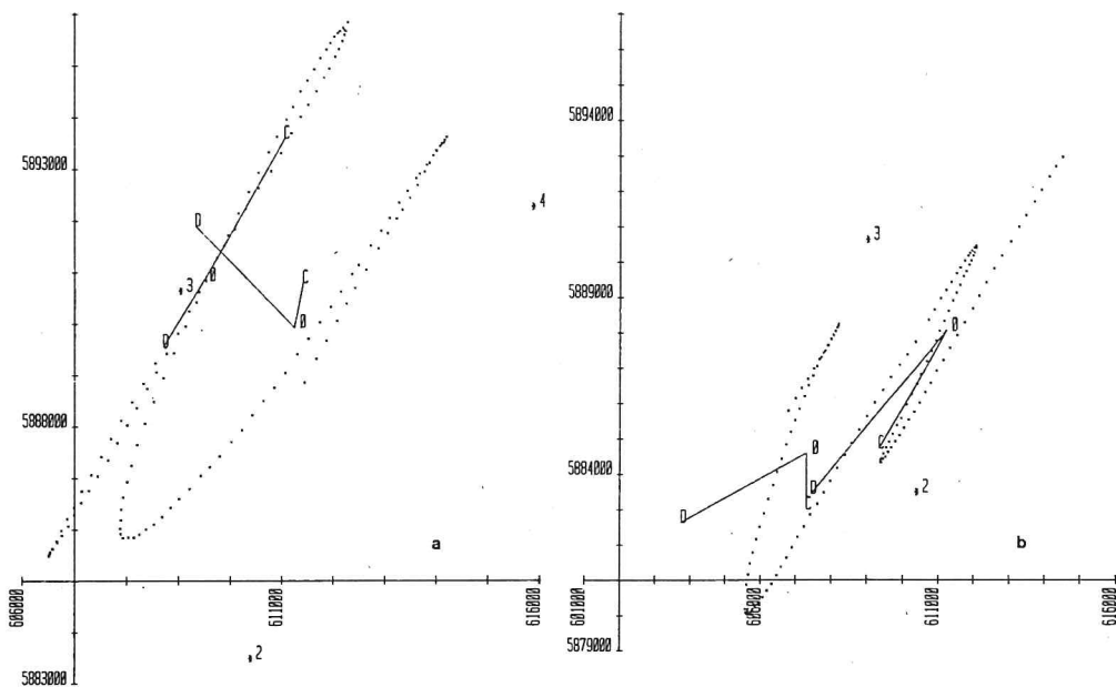
Fig. 101. Current meters interpolation vector C, calculated at the real drifter path, and Lagrangian vector D, plotted at the centroids of two parts of the drifter trajectory. a) 20 and 21 may 1980. Current meters 2, 3 and 4. Drifter 0. First part, 20 may, from 10.10 h till 22.40 h. Second part, from 20 may, 22.40 h till 21 may, 11.10 h. Both parts 750 minutes. b) 21 and 22 may 1980. Current meters 2, 3 and 4. Drifter 0. First part, from 21 may, 16.00 h till 22 may, 04.30 h. Second part, part, 22 may, from 04.50 h till 17.20 h. Both parts 750 minutes.
