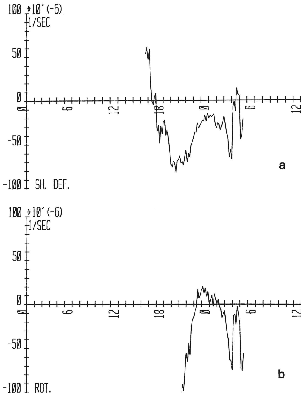
Fig. 79. 23 and 24 june 1980. Drifters. a) Shearing deformation. b) Vorticity.
