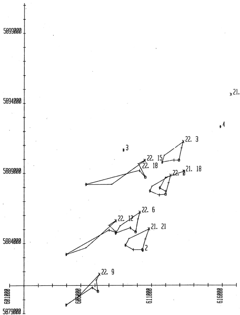
Fig. 38. 21 and 22 may 1980. Shape of the cluster of drifters, every 3 hours.
