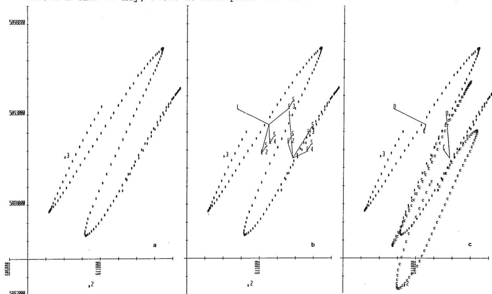
a) Drifter trajectory, from 20 may, 09.40 h till 21 may, 13.00 h. b) Eulerian and Stokes vectors, E and S, of current meters 2, 3 and 4 and Lagrangian vector L. c) Current meters 2, 3 and 4 interpolation vector C and Lagrangian vector D. All vectors are plotted at the centroids of two parts of the drifter trajectory. First part, 20 may, from 10.10 h till 22.40 h. Second part, from 20 may, 22.40 h till 21 may, 11.10 h. Both parts 750 minutes.
