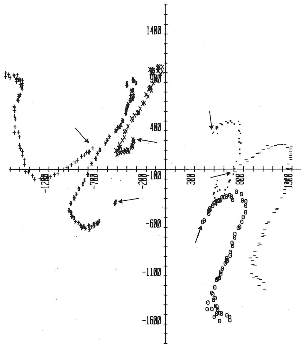
Fig. 60. 16 and 17 june 1980. Displacement of each drifter (m) relative to the centroid of 6 drifters. From 16 june, 16.10 h till 17 june, 02.30 h.
