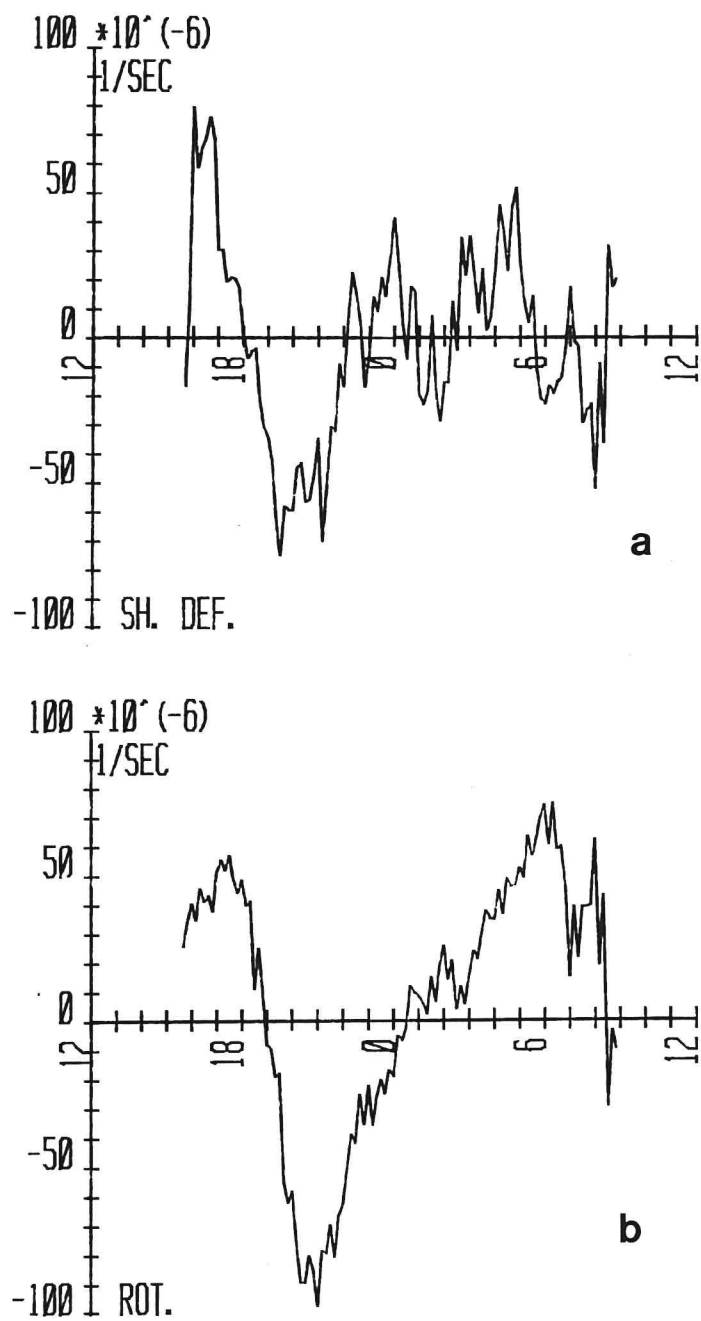
Fig. 64. 16 and 17 June 1980. Drifters. a) Shearing deformation. b) Vorticity.
