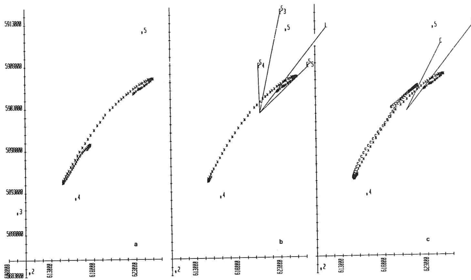
Fig. 73. 23 and 24 June 1980. Drifter 4.
