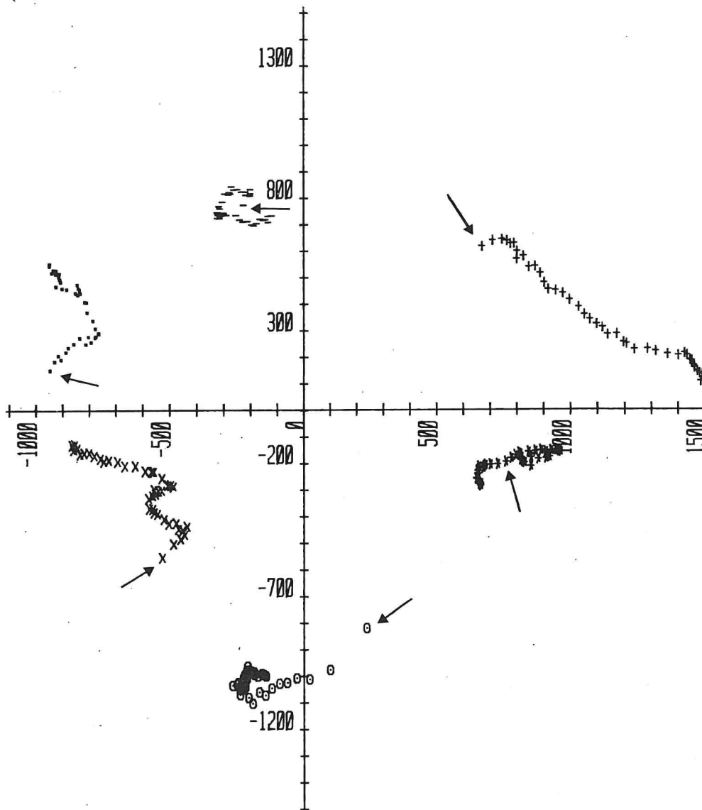
Fig. 15. 19 and 20 May 1980. Displacement of each drifter (m) relative to the centroid of a cluster of 6 drifters. 19 May, from 15.40 h till 22.20 h. → : starting point.
