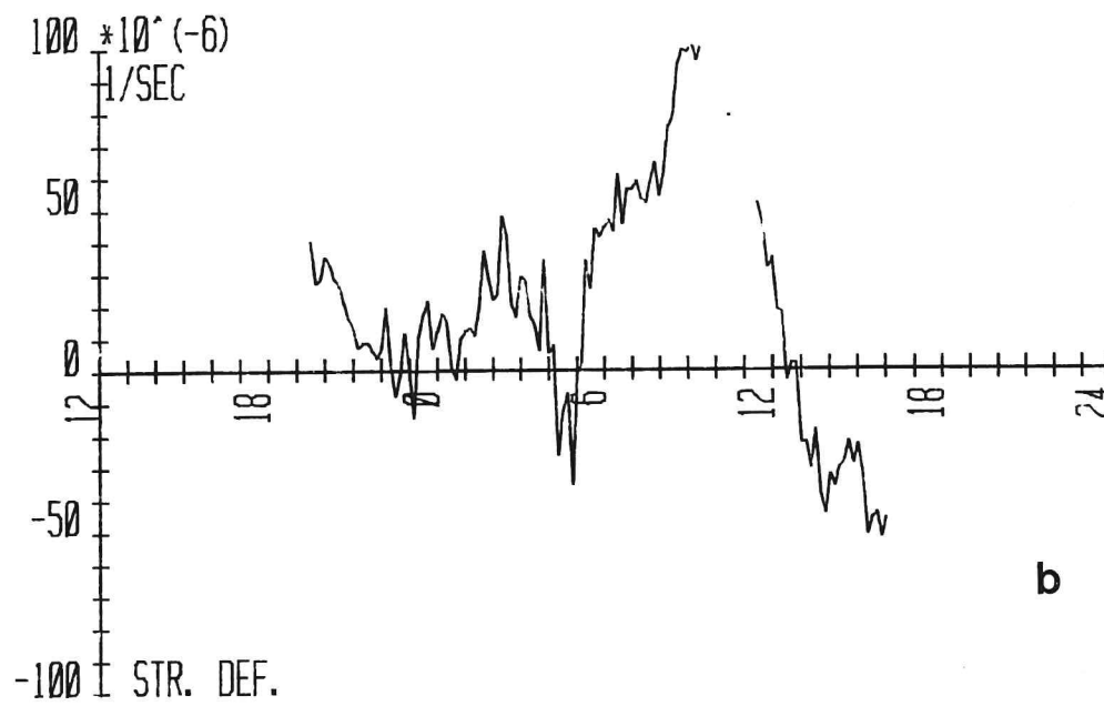
Fig. 48. 21 and 22 may 1980. Drifters. a) Divergence. b) Stretching deformation.
