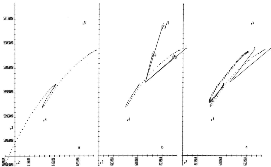
Fig. 69. 23 and 24 June 1980. Drifter 0.
