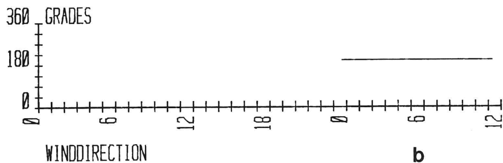
Fig. 66. 23 and 24 june 1980. a) Wind velocity. b) Wind direction.
