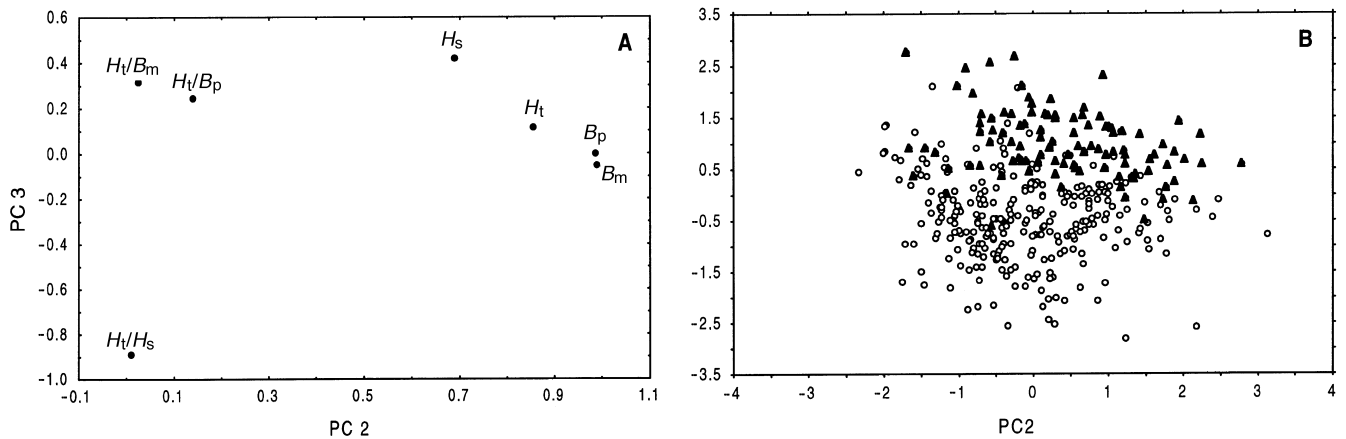
Figure 4. Patterns of shape variation with respect to PC2 and PC3. A. Loadings of each measurement on the two shape components. B. Factor loadings for individuals of Trochelia berniciensis . Loadings plotted against PC2 and PC3 explained 91.53% of the variance. Triangles indicate individuals collected at >940 m.
