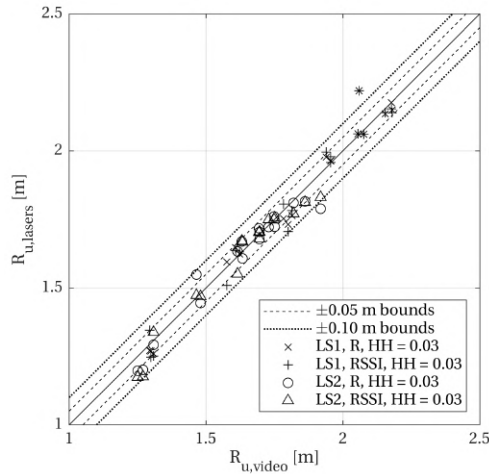
Figure 6.9: Run-up heights from both laser scanners, based on both measured distance ( R ) and laser reflectance ( RSSI ) versus run-up heights from videos, for a test with obliquely incident waves. Distance between laser lines 1.3 m.
