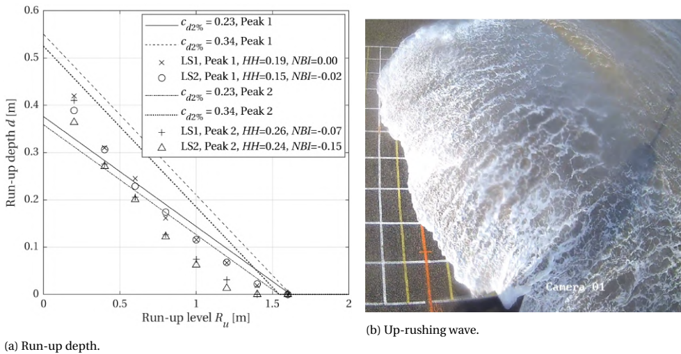
Figure 7.11: Left: Run-up depth at several locations along the dike slope exceeded by 2% of the waves, based on both laser scanners and for both storm peaks. Data compared to linear relation of Van der Meer (2011) for two different values of c_{d2\%} . HH and NBI indicator values given for c_{d2\%} = 0.23 . Right: Snapshot of large up-rushing wave, showing foam and entrained air.
