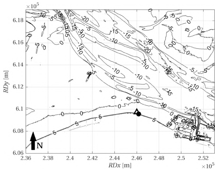
Figure 7.4: Bathymetry of the area of interest, shown as depth contours [m+NAP], with the deep main tidal channel and shallow flats in front of the dike. Laser scanner system (circle) and measurement pole (triangle) locations indicated.
