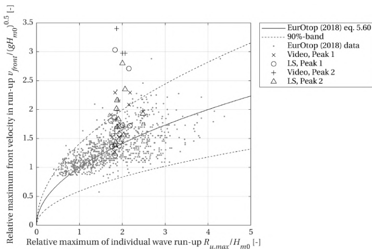
Figure 7.12: Relative maximum front velocity versus relative run-up on the slope. Results based on video analysis (2D velocities) and laser scanners (velocity component in the up-slope direction), compared to Equation 7.8. Figure based on EurOtop (2018), including the FlowDike data (Lorke et al., 2011).
