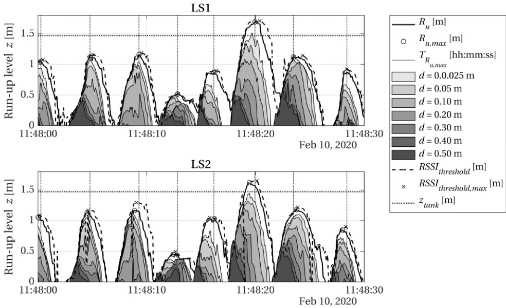
Figure 7.8: Measured run-up heights R_u [m] based on measured distances R (solid lines) and laser reflectance RSSI (dashed lines), as well as measured run-up depths d [m] (contours) for both laser scanners (LS1 and LS2), during a 30 second window. Maximum run-up heights R_{u,max} [m] per wave based on both R (circles) and RSSI (crosses) indicated. Height level of the overtopping tank z_{tank} [m] indicated by the dotted line. Moments of maximum run-up height T_{R_{u,max}} [hh:mm:ss] at LS1 indicated by the dash-dot lines. Note the delay between the signals, where the waves often reached LS2 first with the present wave direction.
