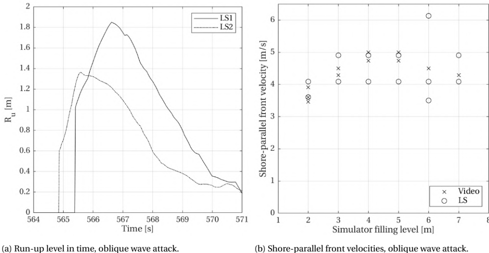
Figure 6.10: Left: Snapshot of run-up level in time for both laser scanners during oblique wave attack. The time lag and different maximum run-up levels are visible. Right: Maximum shore-parallel front velocities determined from laser scanner data (circles) versus video data (crosses). Laser velocities based on the time lags between the laser scanner signals. Distance between laser lines 2.5 m.
