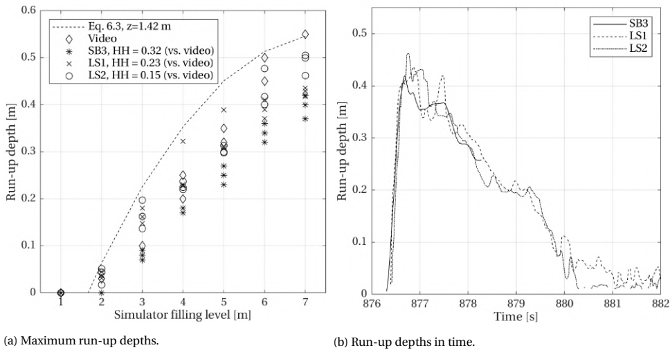
Figure 6.6: Left: Run-up depths as measured with both laser scanners (LS1 and LS2), the third surf board (SB3) and as estimated from videos at z = 1.42 m, compared with the relation of Van der Meer (2011) (Equation 6.3). Right: Run-up depths in time at the same location for a single wave, for both laser scanners and the third surf board.
