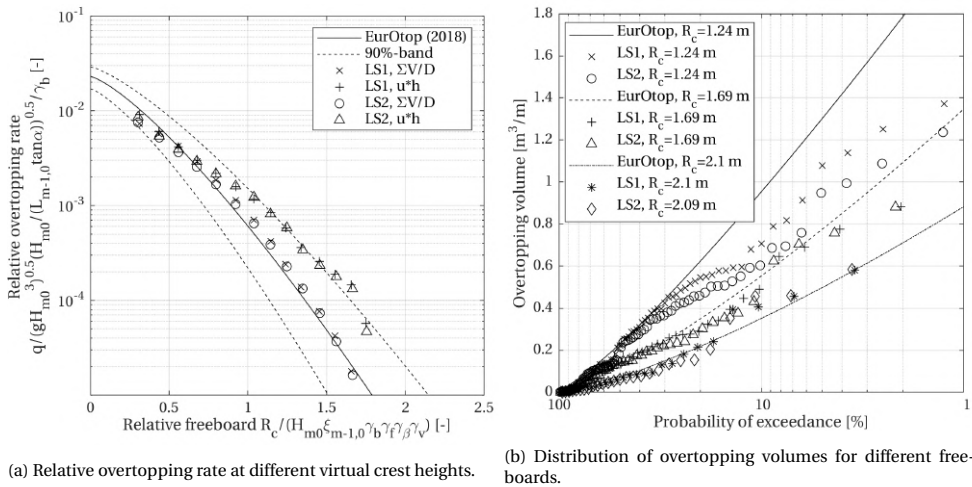
Figure 6.8: Left: Relative overtopping rate at different virtual crest heights based on maximum volumes (crosses, circles) or run-up depth multiplied with front velocity (pluses, triangles) for a test with 100 random perpendicularly incident waves, compared to EurOtop (2018) equations (solid and dashed lines). Right: Distribution of overtopping volumes for three different crest freeboards, compared to EurOtop (2018) . R_c [m] is the crest freeboard, \xi_{m-1,0} [-] the breaker parameter, the different \gamma parameters are influence factors, see EurOtop (2018) .
