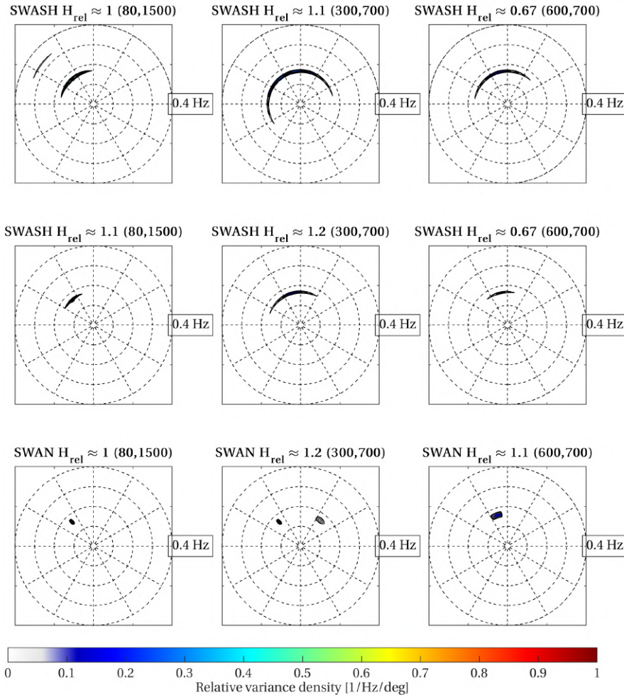
Figure 4.6: 2D spectra at three locations for regular waves travelling from shallower to deeper water with \theta = 48^\circ ( 318^\circ\text{N} ). Top row: SWASH with non-linear waves ( H_s = 1 m). Middle row: SWASH with linear waves ( H_s = 0.1 m). Bottom row: SWAN with non-linear waves ( H_s = 1 m). Variance density of each model normalised and colour-scaled with the maximum variance density at the offshore (80,1500) location.
