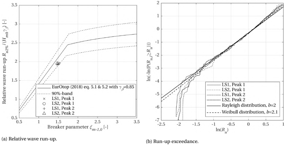
Figure 7.10: Left: Relative wave run-up versus breaker parameter. Figure based on EurOtop (2018). Note the added influence of the oblique wave attack on the vertical axis compared to EurOtop (2018). Data for both laser scanners based on measured distances, and for both storm peaks. Right: Run-up exceedance plots for both laser scanners and both storm peaks, plotted on Weibull scale. A straight line gives a Weibull distribution, a straight line with a slope of 1:2 gives a Rayleigh distribution.
