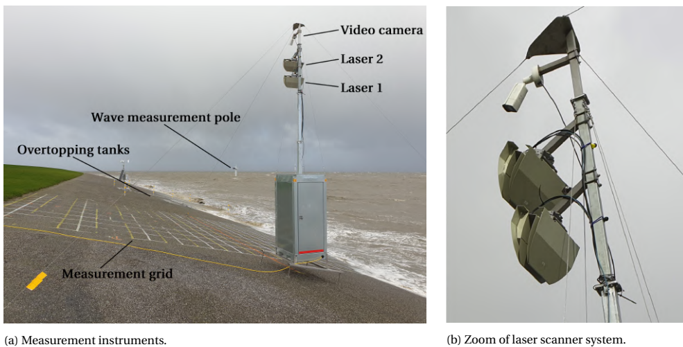
Figure 7.2: Left: New laser scanner system on the dike in the Eems-Dollard estuary, next to the overtopping tanks, during storm Ciara. The Rijkswaterstaat (wave) measurement pole can be seen in the distance. Rijkswaterstaat is the Directorate-General for Public Works and Water Management in the Netherlands. Right: From the bottom to the top, Laser scanner 1, laser scanner 2, video camera.
