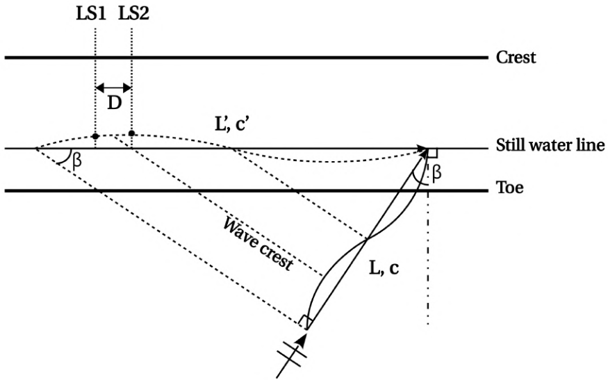
Figure 6.12: Angle of incidence analysis definitions, with an obliquely incident sinusoidal wave (wave direction indicated by the arrow) propagating towards the dike (toe and crest indicated with thick solid lines), with a phase velocity c and a wavelength L . This wave causes a projected wave to travel along the dike, with a velocity c' and a length L' (dashed lines). \beta is the angle of incidence. Laser scanner scan lines indicated by the dotted lines (LS1 and LS2), with a distance D between them.
