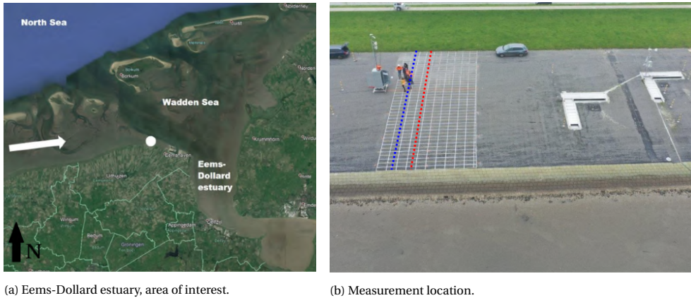
Figure 7.1: Left: The Eems-Dollard estuary in the Netherlands, area of interest of the field measurement project. Laser scanner system location indicated with the white dot. Wind direction during storm Ciara indicated with the arrow. Satellite image: ©2021 GeoBasis-DE/BKG, ©2021 Google. Data: SIO, NOAA, U.S. Navy, NGA, GEBCO. Right: Drone overview of measurement location, with the laser scanner pole (left), the approximate laser scan line locations (blue and red dashed lines), the painted grid on the slope, and two of the overtopping tanks (right).
