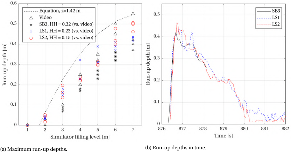
Figure 5.5: Left: Run-up depths at z = 1.42 m for test 1 as measured with both laser scanners, a surf board and from visual estimations, compared with equation from Van der Meer (2011). Right: Run-up depth in time at the same location for a filling level of 7 m and for both laser scanners and the surf board.
