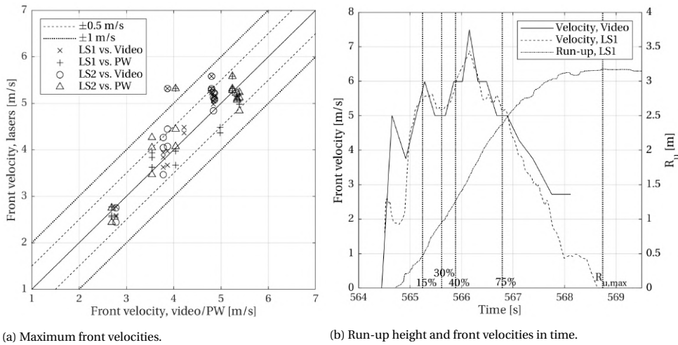
Figure 6.7: Left: Front velocities determined from laser scanner data versus paddle wheel (PW) and video data. Velocities based on front travelling from one paddle wheel to the next. Right: Run-up (dash-dot) and front velocity (dashed) time signals of laser scanner 1 and front velocity time signal (solid line) from video analysis for a single wave. The dotted vertical lines indicate percentages of the maximum run-up level.
