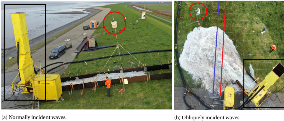
Figure 5.1: Left: Laser scanner system (red circle) and run-up simulator (black rectangle) during tests with normally incident waves. Right: Top view during obliquely incident waves. Scan lines indicated by blue and red lines.
