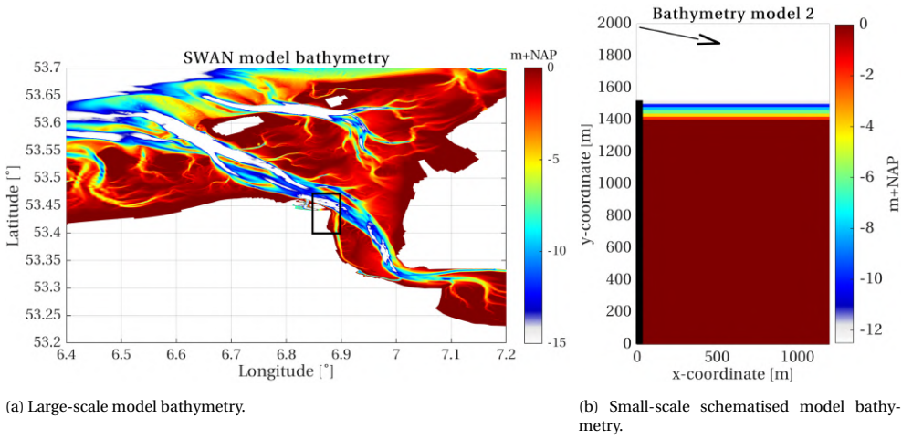
Figure 3.4: Left: SWAN model bathymetry as used for the quantification of propagation effects and the comparison of the two SWAN versions, with the area around the Eemshaven indicated by the rectangle. Right: Bathymetry of the schematised model of the area around the Eemshaven, including the shallow area in front of the dike and a 1:10 slope. The western boundary ( y = 0 m until y = 1500 m) is closed off, representing the dike (thick black line). Mean wave direction indicated with the arrow.
