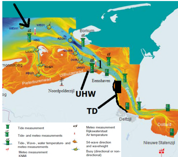
Figure 3.2: Eems-Dollard estuary, with the deep main tidal channel (number 1), the secondary channel the Bocht van Watum (number 2), the dike section of interest (black line), the two locations of interest for setting up the first measurements, Uithuizerwad (UHW) and the Twin Dikes (TD), and the wind direction during extreme conditions (arrow). Blue is deeper, orange is shallower.
