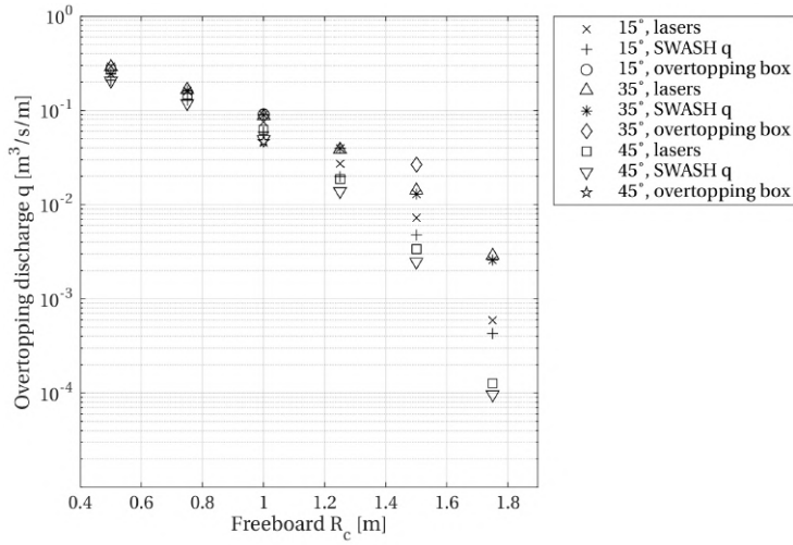
Figure 6.15: Overtopping discharge for several virtual crest levels as determined from the virtual laser scanner data for three SWASH simulations. Tests 10 to 12, with angles of incidence of 15° (crosses), 35° (triangles) and 45° (squares). SWASH discharge parameter q (pluses, asterisks, down-pointing triangles) and virtual overtopping box data (circles, diamonds, pentagrams) plotted as well. Simulations with a 1:4 slope, a JONSWAP spectrum with H_s = 1 m and T_p = 4 s.
