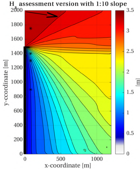
Figure 3.10: Significant wave height H_s during design conditions for the case with a 1:10 slope, using the safety assessment version. Gradients in the wave height occur, resembling diffraction patterns, without inclusion of diffraction in the model. Spectral output locations (asterisks) and mean wave direction (arrow) shown as well.
