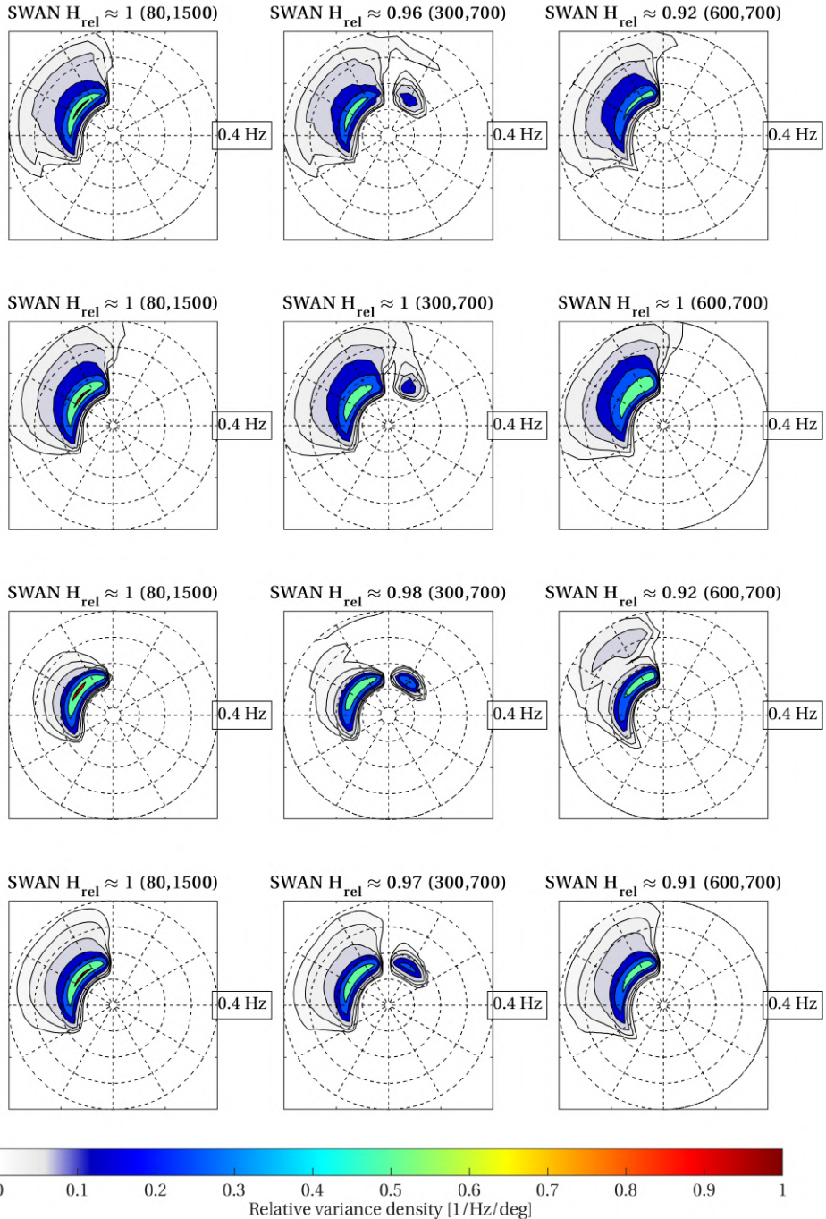
Figure 4.11: 2D spectra at three locations for irregular, broad-spread waves travelling from shallower to deeper water with an angle of incidence of 48^\circ ( 318^\circ\text{N} ) and a 35\text{ m/s} wind coming from 318^\circ\text{N} imposed. Top row: SWAN with default settings. Second row: SWAN with WBI settings. Third row: SWAN with ST6 settings. Bottom row: SWAN with recommended settings, with 20\text{ m} grid cells and the diffraction approximation enabled. Variance density of each model normalised and colour-coded with the maximum variance density at the offshore (80,1500) location.
