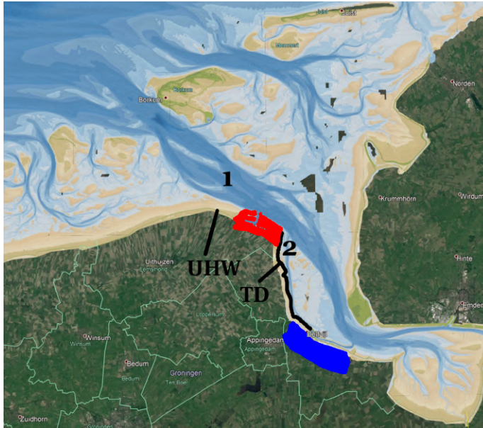
Figure 1.2: Eems-Dollard estuary, with the port Eemshaven (red area), the town Delfzijl (blue area), the deep main tidal channel (number 1), the secondary channel the Bocht van Watum (number 2), the dike section of interest (black line) and the two locations of interest for the field measurements, Uithuizerwad (UHW) and the Twin Dikes (TD). Bathymetrical data from Rijkswaterstaat six-yearly bathymetrical surveys, blue is deeper, yellow is shallower.
