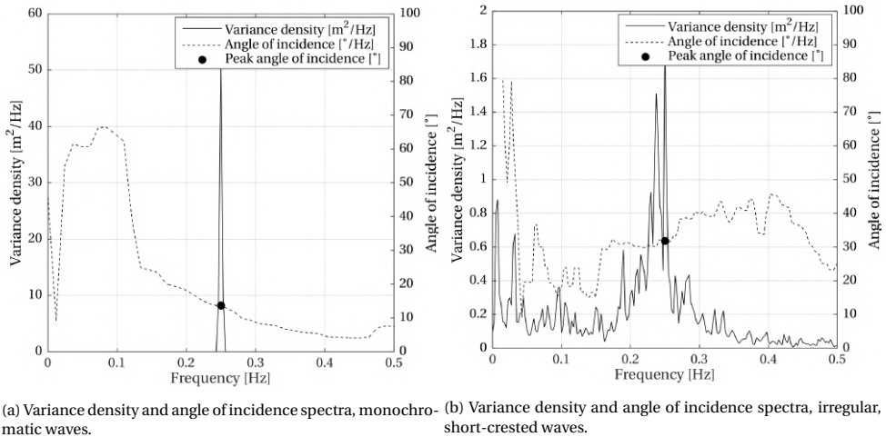
Figure 6.13: Variance density spectra (solid lines) based on virtual laser line run-up data and angle of incidence spectra (Equation 6.9, dashed lines) for two cases. Left: Angle of incidence of 15°, water depth of 10 m, a vertical wall and monochromatic waves. Right: Angle of incidence of 35°, water depth of 2.5 m, 1:4 dike slope and irregular, short-crested waves. The angle of incidence spectra give the angle of incidence for each mode in the spectrum of the measured run-up. The angle of incidence \beta was defined according to Figure 6.12. Peak angles of incidence indicated by the circles.
