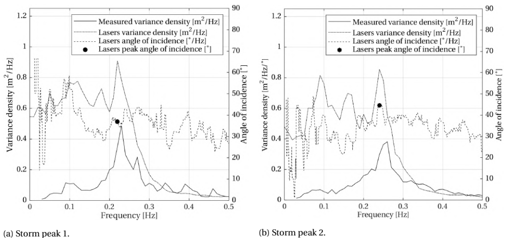
Figure 7.15: Wave variance density spectra based on radar measurements (solid lines), variance density spectra based on laser scanner run-up signals (dash-dot lines) and 'angle of incidence spectra' (dashed lines) for both storm peaks, giving the angle of incidence for each mode in the spectrum. The dots indicate the peak angles of incidence.
