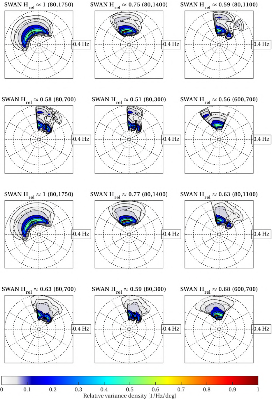
Figure 4.18: 2D SWAN spectra at several locations. First two rows: SWAN with recommended settings, without wind imposed. Bottom two rows: SWAN with recommended settings, with wind. Variance density normalised and colour-scaled with the maximum variance density at the offshore (80,1750) location.
