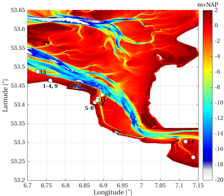
Figure 1.5: Eems-Dollard estuary with measurement instruments as of the end of 2020. See Table 1.1 for the definitions of the numbers and further details on the instruments. Bathymetrical data from Rijkswaterstaat six-yearly bathymetrical surveys.
