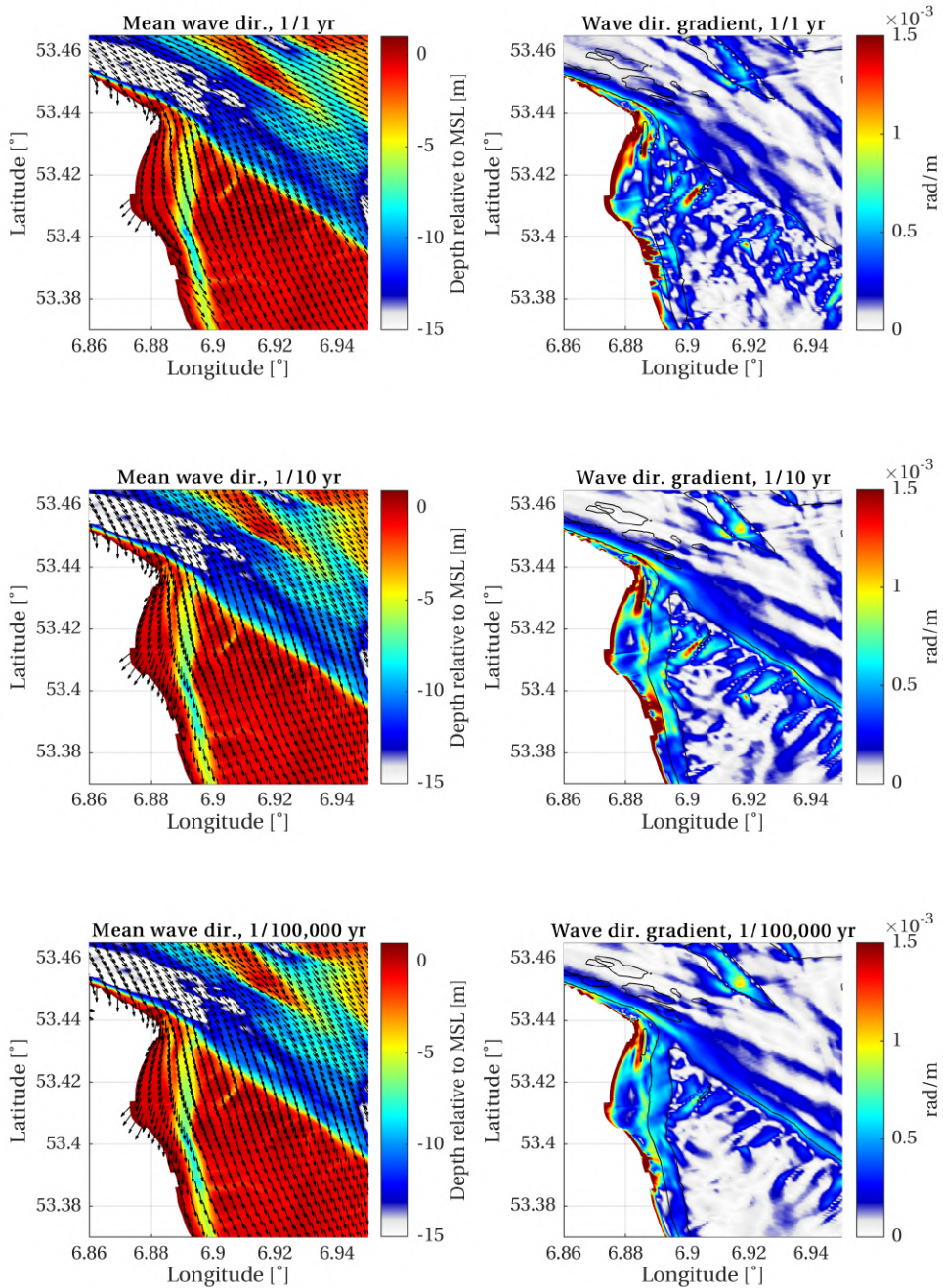
Figure 3.5: Results for return periods of 1 year, 10 years and 100,000 years. Left: SWAN model bathymetry and mean wave direction vectors. Right: Absolute gradient in mean wave direction. Bottom contours drawn at -3 m, -15 m and -25 m.
