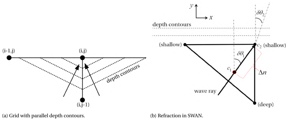
Figure B.1: Left: Geographic grid with parallel depth contours, after Booij (1998). Right: SWAN refraction situation sketch. Definitions of variables given in the main text. Figure after Zijlema (2020).
