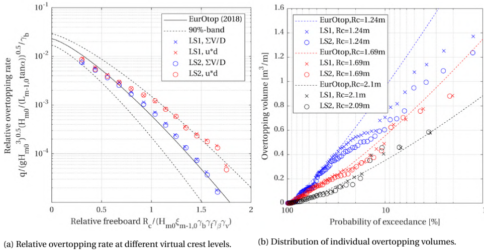
Figure 5.7: Left: Relative overtopping rate for several virtual crest levels for test 1a and based on maximum volumes or run-up depth multiplied with front velocity, compared to EurOtop (2018) equations. Right: Distribution of individual overtopping volumes, compared to EurOtop (2018) . R_c [m] is the crest freeboard, \xi_{m-1,0} [-] is the breaker parameter, the different \gamma parameters [-] are influence factors, see EurOtop (2018) .
