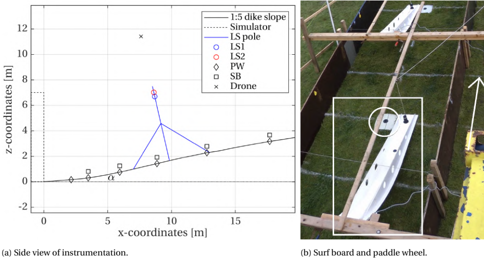
Figure 6.2: Left: Side view of system set-up and instrumentation. x -coordinates horizontal, z -coordinates vertical, y -coordinates perpendicular to the figure. \alpha [ ^\circ ] is the slope angle. LS pole is the laser scanner pole, LS1 the lower laser scanner, LS2 the upper laser scanner. PW are the 6 paddle wheels; SB the five surf boards. Right: Example of surf board (white rectangle) and paddle wheel (white circle). Up-slope direction indicated by the arrow.
