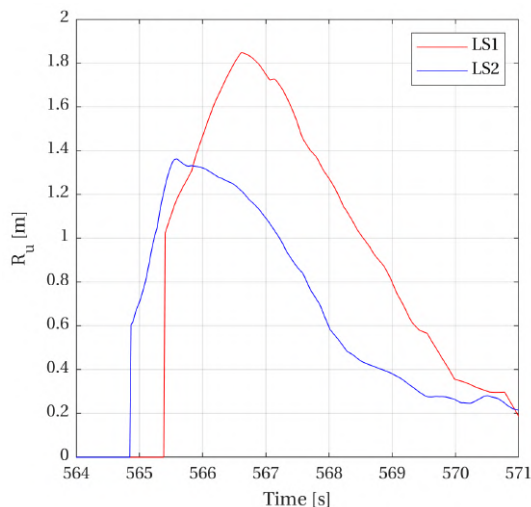
Figure 5.8: Snapshot of run-up level in time for both laser scanners during oblique wave attack. The time lag and different maximum run-up levels are visible.
