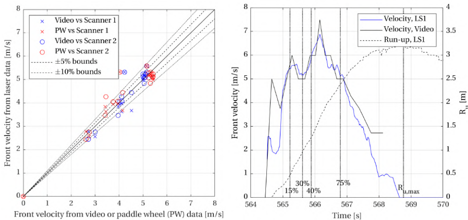
(a) Maximum front velocities.
