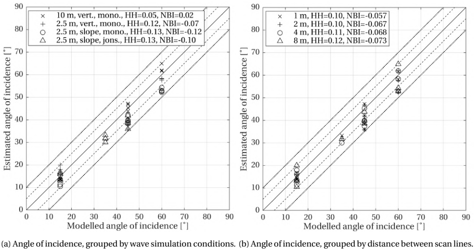
Figure 6.14: Wave angle of incidence data for all SWASH simulations, comparing peak angles of incidence as modelled by SWASH with peak angles of incidence derived from virtual laser scanner data (see Figure 6.13). Left: Data grouped according to simulation conditions (water depth 10 m or 2.5 m, vertical wall or 1:4 slope, monochromatic or irregular waves). Right: Data grouped according to distance between the scan lines (1 m, 2 m, 4 m or 8 m). HH and NBI values, and \pm 5^\circ and \pm 10^\circ error bounds (dashed and dotted lines) given as well.
