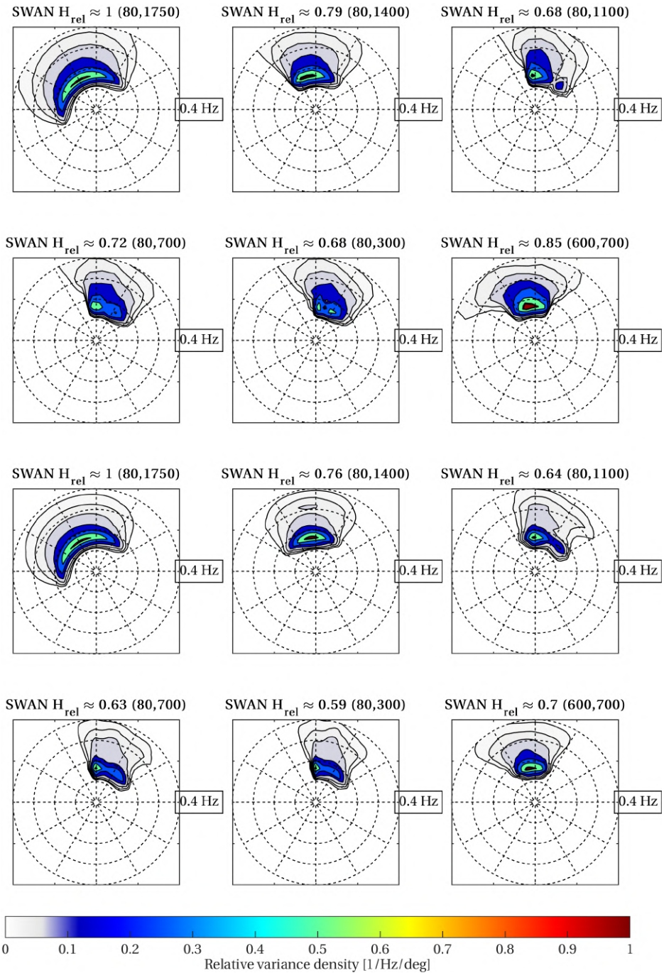
Figure 4.19: 2D SWAN spectra at several locations. First two rows: SWAN with WBI settings, with wind imposed. Bottom two rows: SWAN with recommended settings, diffraction approximation, 20 m grid cells and with wind. Variance density normalised and colour-scaled with the maximum variance density at the offshore (80,1750) location.
