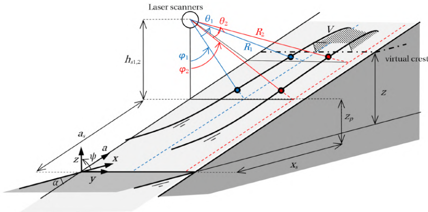
Figure 7.7: Schematised updated set-up with two laser scanners. Scan lines (red and blue dashed lines), scanned points on water surface (red and blue dots) are indicated. x (horizontal), y (perpendicular), z (vertical) and a -coordinate (along the slope) system is also indicated. R_{1,2} [m] are the scanned distances, \theta_{1,2} [°] are the scan angles, \phi_{1,2} [°] the slant angles, x_s [m] are the x -coordinates of the laser scanners, a_s [m] the a -coordinates of the laser scanners, z_p [m] is the z -coordinate of the laser scanner pole, h_{s1,2} [m] are the heights of the laser scanners above the slope, \alpha [°] is the slope angle. V [m 3 ] is a virtual overtopping volume, \psi [°] is the correction angle resulting from the rotation matrix, rotating the x - and z -coordinates in the x, z -plane.
