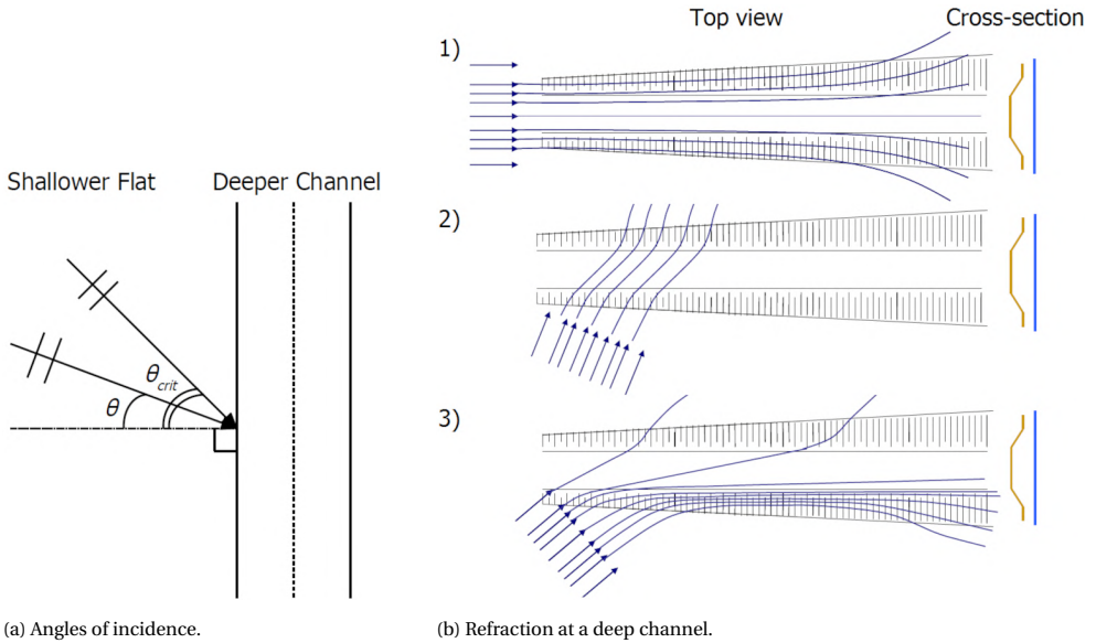
Figure 4.2: Left: Definition of incident angle \theta [°] and critical angle \theta_{crit} [°], relative to the normal to the depth contours, based on Snell's law. The dashed line is the channel axis. Right: Waves propagating in three different directions over a channel. Longitudinally (1), at an angle smaller than the critical angle (2) and at the critical angle (3). Figure after Guzman Mardones (2011) ; Zwamborn and Grieve (1974) .
