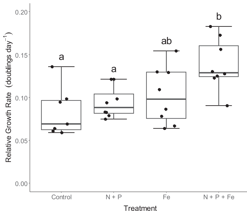
Fig. 1. Relative growth rate (RGR) of Sargassum fluitans III under different nutrient enrichment treatments. Boxplot shows quartiles, median, and significant differences. Letters indicate significantly different groups after application of a post-hoc Tukey test ( p < 0.05 ).
