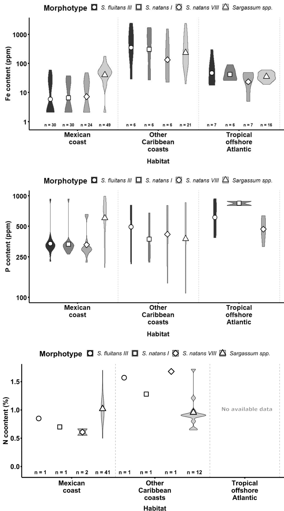
Fig. 3. Violin plots summarizing sargassum Fe, P and N content, grouped per zone and species. Sargassum spp. is a mix of species and morphotypes. Data from 20 publications for Fe, 9 for P, 7 for N, and own data from Mexico (this study, and 30 points from a cruise around Cozumel) and Bonaire (2 bays). Locations, morphotypes and repeated measurements differing at least 1 month are defined as separate entries.
