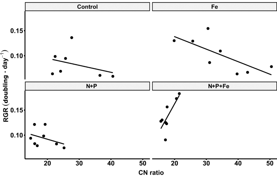
Fig. 2. Relationship between tissue C:N ratio and Relative Growth Rate (RGR) of Sargassum fluitans III under four nutrient regimes.
