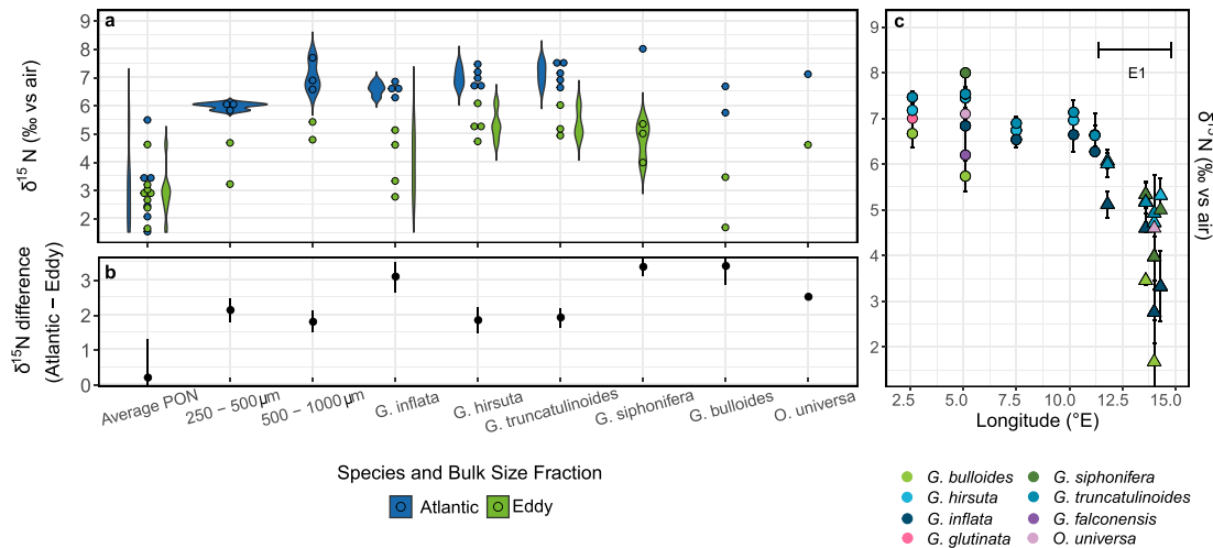
Figure 7. (a) Violin plot showing the concentration-weighted average \delta^{15}\text{N} of mixed-layer particulate organic N, bulk zooplankton (250–500 and 500–1,000 \mu\text{m} size classes), and foraminifer tissue (i.e., FT- \delta^{15}\text{N} ) for six species collected in the 0–200 m net tows in 2017. Circles represent the average FT- \delta^{15}\text{N} measured in triplicate for each species at a single station, with the blue circles indicating Atlantic stations and the green circles showing the Agulhas eddy (E1) data. The shapes behind or alongside the circles show the spread of the data; (b) The difference in mean FT- \delta^{15}\text{N} between Atlantic and E1 foraminifera for each particulate pool or foraminifer species; (c) Species-specific average FT- \delta^{15}\text{N} at each station sampled along the transect, with circles and triangles representing Atlantic and eddy stations, respectively.
