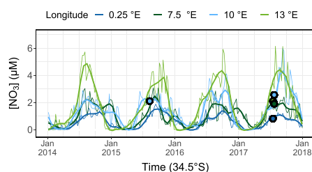
Figure 3. Surface (0.5 m) nitrate concentrations from the CMEMS product at four locations along the SAMBA transect (34.5°S; 0.25°E (dark blue), 7.5°E (dark green), 10°E (light blue), 13°E (light green)) between January 2014 and January 2018. The thin lines show monthly reanalysis data and the thick lines show smoothed data (moving average = 2 weeks) ( http://marine.copernicus.eu/documents/QUID/CMEMS-GLO-QUID-001-028.pdf ). Colored circles indicate the surface nitrate concentrations measured at the corresponding locations during the 2015 and 2017 cruises.
