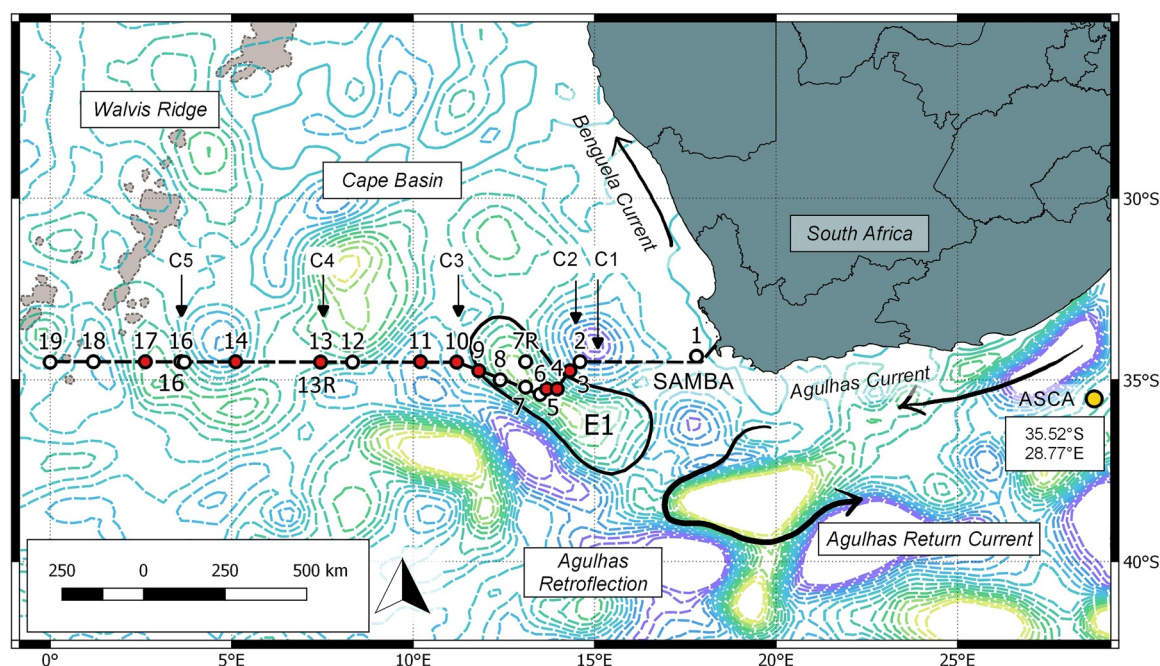
Figure 1. Cruise track followed by the R/V S.A. Agulhas II in July 2017 along the SAMBA line (dashed black transect). Contour lines show sea-surface height anomaly (SSHA) relative to the geoid (SSALTO/DUACS product distributed by AVISO via the Copernicus Marine Environment Monitoring Service (Lea et al., 2018; http://marine.copernicus.eu , 24 July 2017)), with positive and negative anomalies shown by the light green and purple dashed lines, respectively. The outer edge of Agulhas eddy E1, as defined in Section 2.4, is indicated by the thick black contour. Along the transect, the white circles represent stations sampled for nitrate concentration, nitrate isotopes, and particulate organic nitrogen, while red circles show stations where foraminifera and bulk zooplankton were additionally collected using net tows. The positions of stations sampled in 2015 along the same 34.5°S transect (Campbell, 2016; Marconi et al., 2017) are indicated by arrows and labeled C1–C5, noting that the background SSHA does not apply to these stations. The position of a station located in the Agulhas Current region in the southwest Indian Ocean (in the vicinity of the ASCA line) that was sampled in July 2016 is indicated by the yellow circle.
