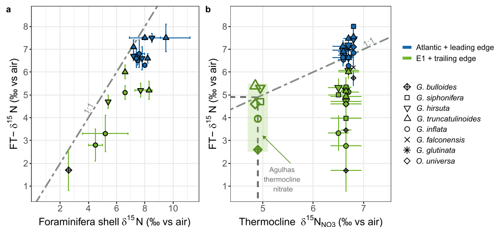
Figure 8. (a) Cross-plot of FT- \delta^{15}\text{N} vs. foraminifera shell-bound \delta^{15}\text{N} from the same net tows; (b) Comparison of FT- \delta^{15}\text{N} and thermocline \delta^{15}\text{N}_{\text{NO}_3} (approximated by the \delta^{15}\text{N}_{\text{NO}_3} of SASMW measured across the transect). Blue symbols show nitrate and foraminifer measurements from the Atlantic stations and the leading edge of Agulhas eddy E1 while green symbols show data from within E1 and include the trailing edge station (see Section 2.4 for details). Error bars show \pm 1 standard deviation of triplicate measurements of the same foraminifer species at each station (y-axis) and duplicate nitrate isotope measurements from the same station and depth (x-axis). In panel b, open symbols in the shaded green box indicate where the average eddy FT- \delta^{15}\text{N} for each foraminifer species would be positioned if plotted versus the mean Agulhas thermocline \delta^{15}\text{N}_{\text{NO}_3} ( 4.9\text{‰} ); calculated for all thermocline data available for the Agulhas System Climate Array line (Marshall et al., 2023) rather than from just the representative Agulhas profile shown in Figure 4b. The dashed gray line in both panels indicates a 1:1 line.
