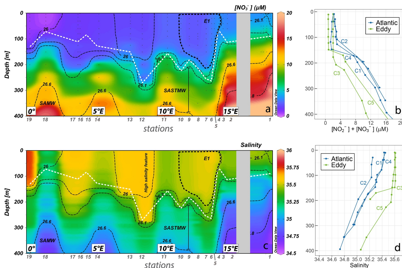
Figure 2. Section plots from the 2017 cruise showing (a) nitrate concentration and (c) salinity overlaid with isopycnals ( \text{kg m}^{-3} ; dotted black contour lines). Subantarctic Mode Water (SAMW) and South Atlantic Subtropical Mode Water (SASTMW) are defined by density (Donners et al., 2005). The approximate mixed layer depth is indicated by the dashed white line. Sampling station numbers are labeled on the bottom x-axis, and the location of Agulhas eddy E1 is shown by the dashed black polygon (labeled E1). Panels (b) and (d) show the vertical profiles of nitrate and salinity for the SAMBA stations sampled in 2015, with the colors indicating whether those stations were located in background Atlantic- (blue) or Agulhas eddy (green) waters at the time of sampling.
