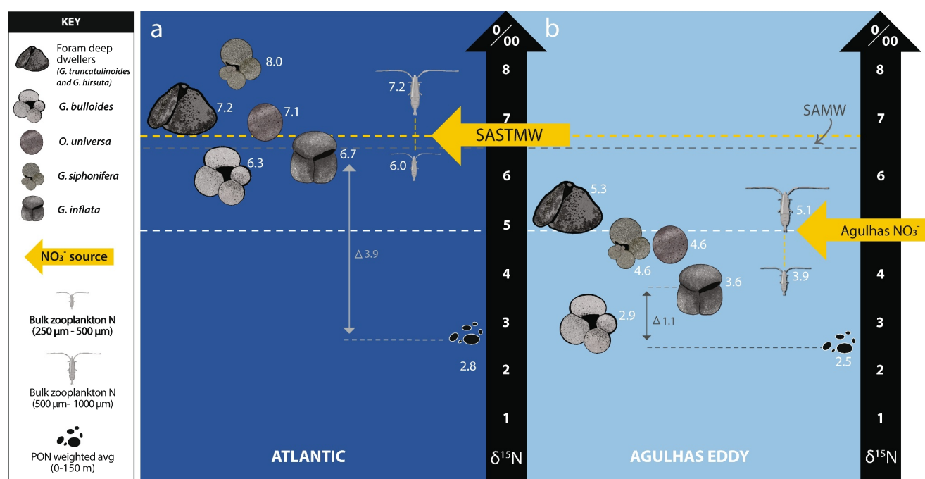
Figure 9. Schematic of the proposed nitrogen isotope dynamics in (a) the background Atlantic and (b) an Agulhas eddy sampled in the Cape Basin in 2017, with \delta^{15}\text{N} shown by the vertical black arrows. The horizontal yellow arrows and dashed lines indicate South Atlantic Subtropical Mode Water (SASTMW, \delta^{15}\text{N}_{\text{NO}_3} of 6.9‰), which is the water mass (and nitrate supply) located directly below the mixed layer across the Cape Basin. The arrows in panel (b) show the mean \delta^{15}\text{N}_{\text{NO}_3} of Agulhas Current thermocline nitrate ( \delta^{15}\text{N}_{\text{NO}_3} of 4.9‰) and Subantarctic Mode Water (SAMW, \delta^{15}\text{N}_{\text{NO}_3} of 6.7‰) (Marshall et al., 2023), which underlies the thermocline and is the ultimate source of nitrate to both the Cape Basin and Agulhas region. Suspended particulate organic N (PON) \delta^{15}\text{N} , bulk zooplankton \delta^{15}\text{N} (for the 250–500 \mu\text{m} and 500–1,000 \mu\text{m} size classes), and FT- \delta^{15}\text{N} are shown using symbols and images of the various species (see legend). The numbers next to the organisms indicate their biomass \delta^{15}\text{N} , in units of ‰. The thin vertical arrows show the calculated difference ( \Delta ) in \delta^{15}\text{N} between an example foraminifer species ( G. inflata ; chosen due to its high abundance across the transect and its mid-range trophic position) and the suspended PON.
