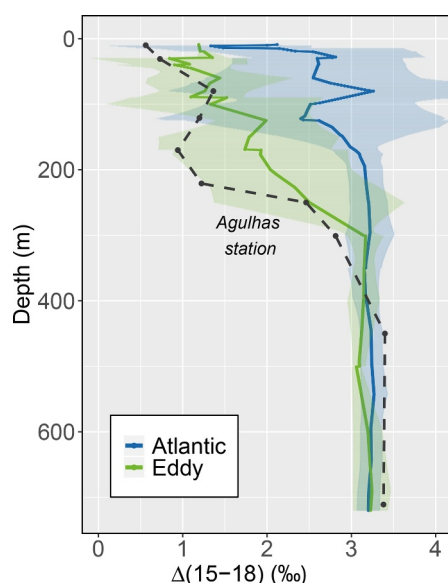
Figure 5. Average nitrate \Delta(15-18) , i.e., (\delta^{15}\text{N}_{\text{NO}_3} - \delta^{18}\text{O}_{\text{NO}_3}) , at the Atlantic and eddy stations, gridded at 1 m intervals. Shaded areas indicate \pm 1 standard deviation of the combined 2015 and 2017 data set. The black dashed line shows the nitrate \Delta(15-18) for the Agulhas Current station included in Figure 4 (Marshall et al., 2023).
