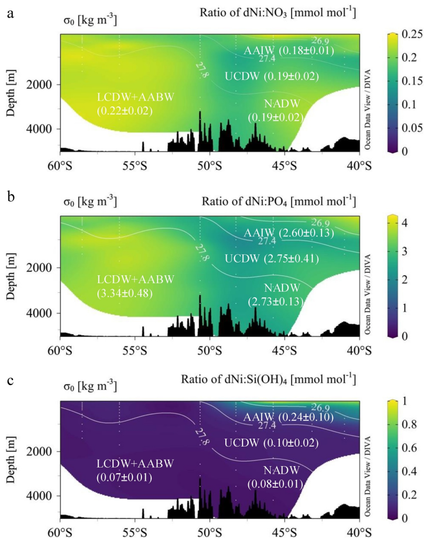
Figure 6. Sections of key subsurface water masses in the Southern Ocean showing ratios (mean \pm sd) of dNi to (a) NO 3 , (b) PO 4 , and (c) Si(OH) 4 . Isolines represent potential densities ( \sigma_0 ) aimed at delineating water mass depths. Water mass abbreviations as per Figure 2. Figure constructed with Ocean Data View (Schlitzer, 2023).
