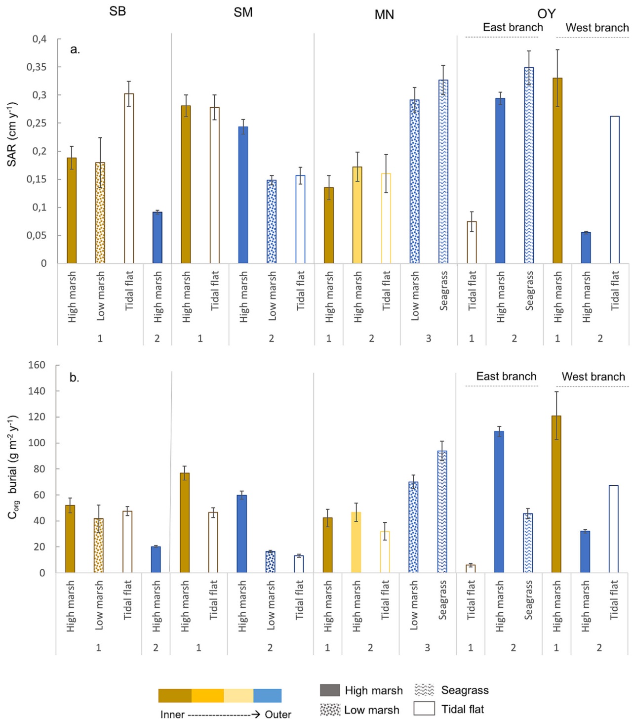
Fig. 6. Mean \pm SE a) sediment accretion rate (SAR cm y -1 ) and b) C org burial rate (g m -2 y -1 ) since 1960 estimated per habitat (n = 1 core) within each section per estuary (SB: Santander Bay; SM: Santoña Marshes; MN: Mondego estuary; OY: Oyambre). Number above the bars indicates the sampling area within each estuary. Color gradient indicates relative position along the estuary (from inner to outer sections) while bar fill patterns represent different habitats.
