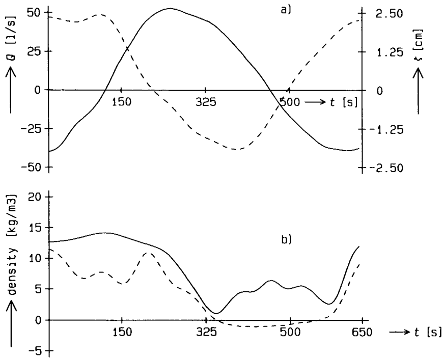
Figure 3.31 Time-histories of the discharge, the water level, and the density in the river in front of the harbour: a) —, discharge and ---, water level elevation; b) —, density at 0.047 m above the bottom; ---, density at 0.14 m above the bottom (1000 kg/m 3 is subtracted from the density).
