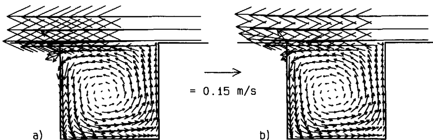
Figure 4.19 Computed flow patterns at t = 375 s, \nu_t^1 = \nu_t^2 = 5.0\text{E-}4 \text{ m}^2/\text{s} : a) 0.0935 m, and b) 0.044 m above the bottom, respectively.
