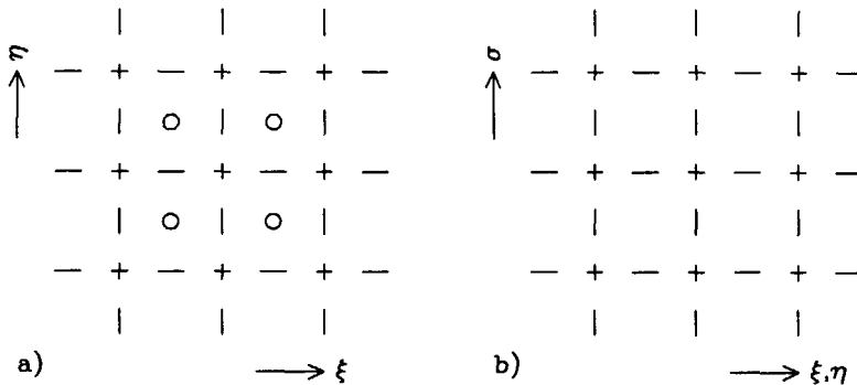
Figure 4.3 Computational grid of TRISULA: a) + = \zeta and c , - = u , | = v , and \circ = d ; b) + = c , - = u or v , and | = \omega .
