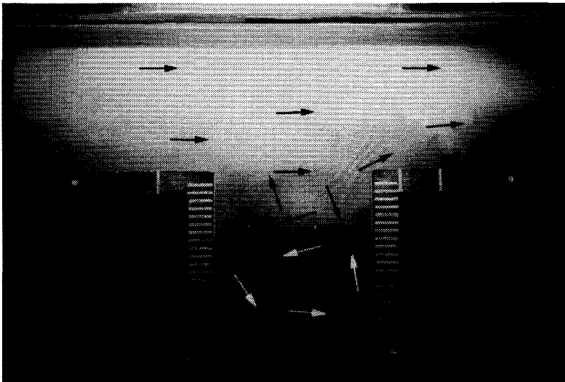
Photo 2 Exchange of dyed water from harbour 1 and limpid river-water at t \approx 50 s (experiment 1B).
