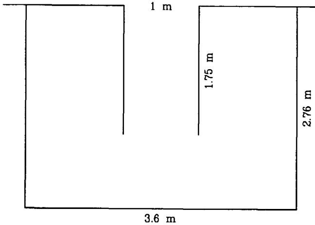
Figure 3.18 Top view of model harbour 6.
