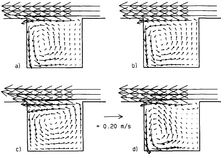
Figure 4.5 Influence of the eddy viscosity on the depth-averaged flow patterns in the harbour at t = 325 s: a) \nu_t = 5.0\text{E-}4 \text{ m}^2/\text{s} , b) \nu_t = 1.0\text{E-}3 \text{ m}^2/\text{s} , c) \nu_t = 5.0\text{E-}3 \text{ m}^2/\text{s} , and d) \nu_t = 0.11u_*h + 1.0\text{E-}5 \text{ m}^2/\text{s} .
