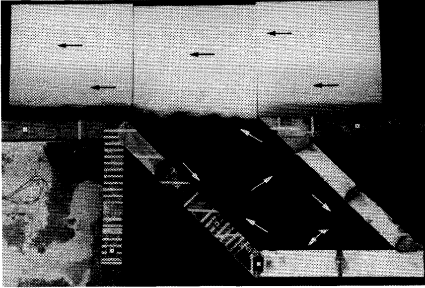
Photo 7 Exchange of dyed water from harbour 4 and limp river-water at maximum current ( t = 375 s).
