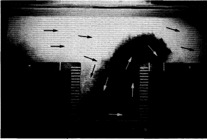
Photo 1 Exchange of dyed water from harbour 1 and limpid river-water shortly after slack water ( t \approx 10 s, experiment 1B).
