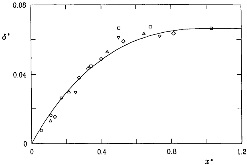
Figure 2.4 Width of the mixing layer. Results of five tests: ○, h/c_f = 8.67 m; Δ, h/c_f = 4.59 m; ▽, h/c_f = 4.00 m; ◇, h/c_f = 3.72 m; □, h/c_f = 2.89 m. — = equation 2.5. (From Chu & Babarutsi, 1988.)
