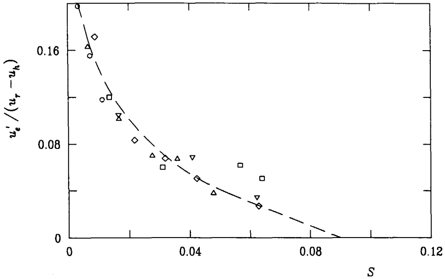
Figure 2.3 Variation of the transverse component of turbulence with bed-friction number. Results of five tests: \circ , h/c_f = 8.67 m; \Delta , h/c_f = 4.59 m; \nabla , h/c_f = 4.00 m; \diamond , h/c_f = 3.72 m; \square , h/c_f = 2.89 m. (From Chu & Babarutsi, 1988.)
