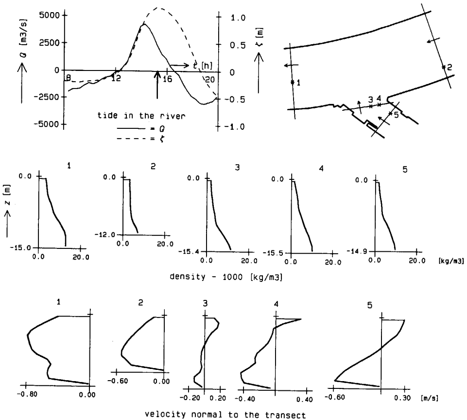
Figure 5.6 Vertical distributions of density and velocity in the 1 st Petroleum Harbour at high tide ( t = 15\text{h}15 ).
