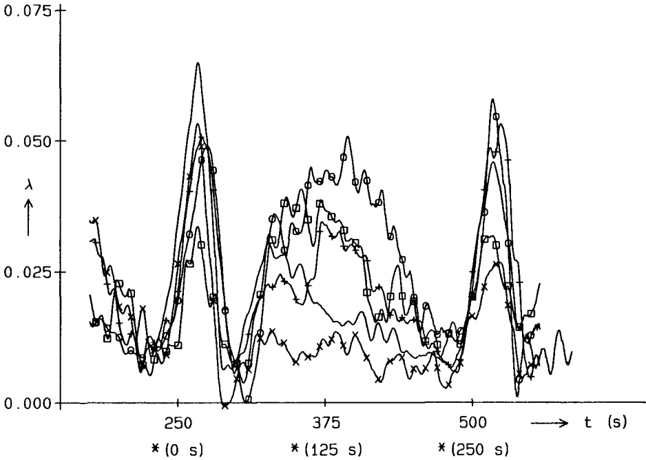
Figure 3.16 Normalized heat transport through the entrance: —, harbour 1; —+—, harbour 2; —□—, harbour 3; —○—, harbour 4 (time indicated by *); and —x—, harbour 4.
