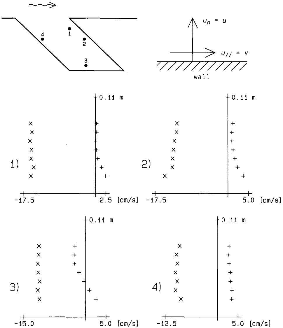
Figure 3.13 Velocity distributions in the water column in harbour 4: + = u velocity component and x = v velocity component.
