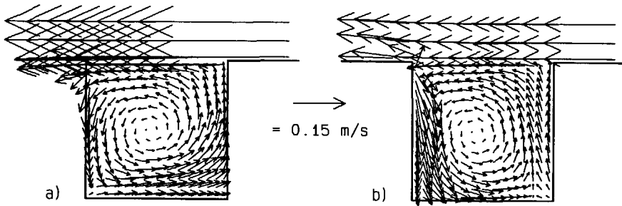
Figure 4.20 Computed flow patterns at t = 405 s, \nu_t^h = 5.0\text{E-}4 m 2 /s and \nu_t^v = 1.0\text{E-}4 m 2 /s: a) 0.0935 m, and b) 0.044 m above the bottom, respectively.
