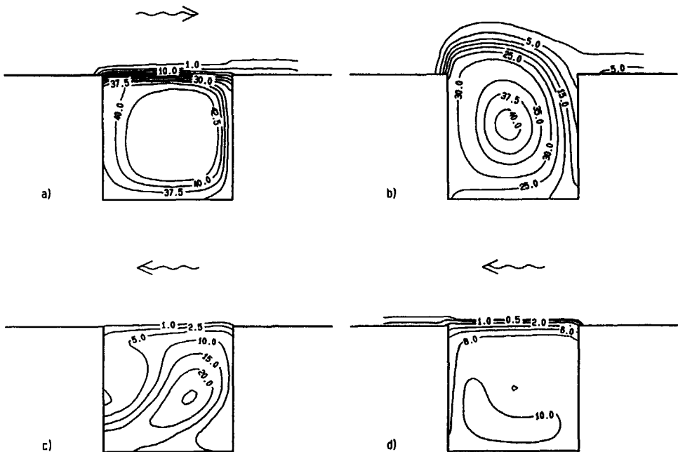
Figure 4.9 Isolines of concentration in \text{g}/\text{m}^3 ( D_t = 5.0\text{E-}3 \text{ m}^2/\text{s} ): a) t = 175 \text{ s} , b) t = 250 \text{ s} (slack water), c) t = 300 \text{ s} , and d) t = 375 \text{ s} (maximum current).
