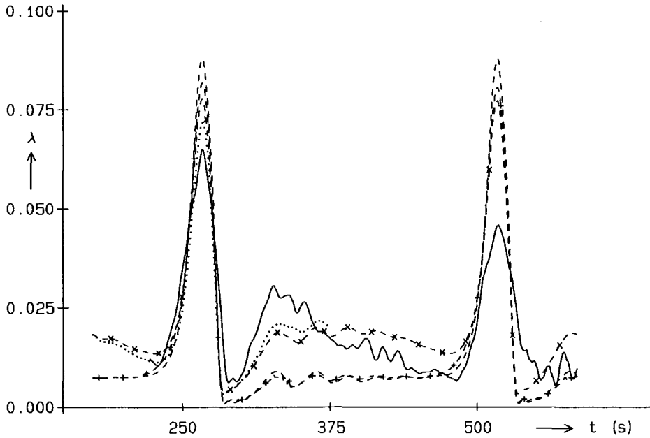
Figure 4.11 Normalized transport through the entrance: measured, —; computed, — — — = isotropic dispersion ( D_t = 5.0E-3 \text{ m}^2/\text{s} ), - - - - = anisotropic dispersion ( \gamma = 0.15 ), -x-x- = anisotropic dispersion ( \gamma = 1.0 ), and . . . . = anisotropic dispersion ( \gamma = 1.0 and \Delta x = 0.025 \text{ m} ).
