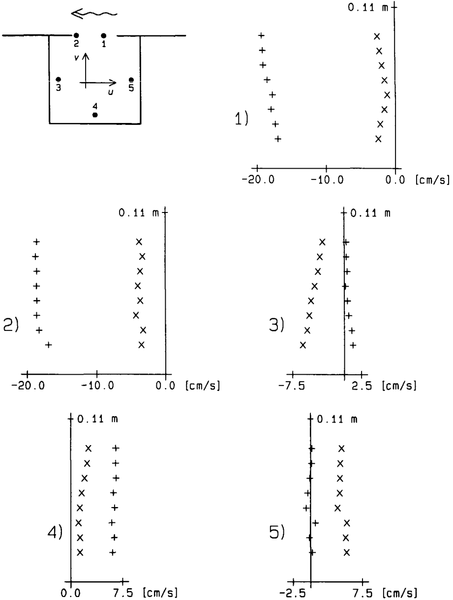
Figure 3.12 Velocity distributions in the water column in harbour 3: + = u velocity component and x = v velocity component.
