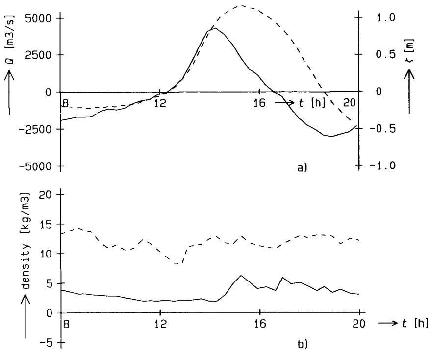
Fig. 5.2 Time histories of discharge, water level elevation, and density in the river in front of the harbour: a) —, discharge and - - -, water level elevation with respect to NAP; b) —, density at 6 m below the free surface and - - -, density at 12 m below the free surface.
