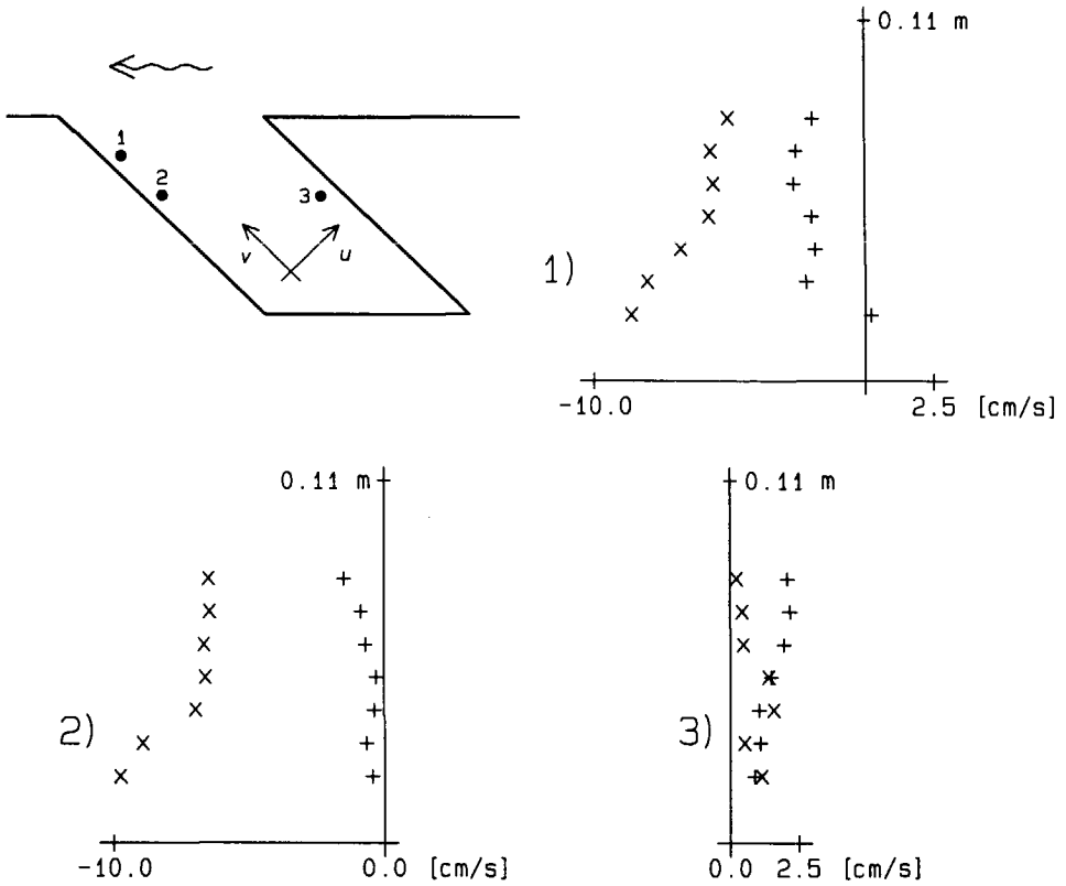
Figure 3.14 Velocity distributions in the water column in harbour 4: + = u velocity component and \times = v velocity component.
