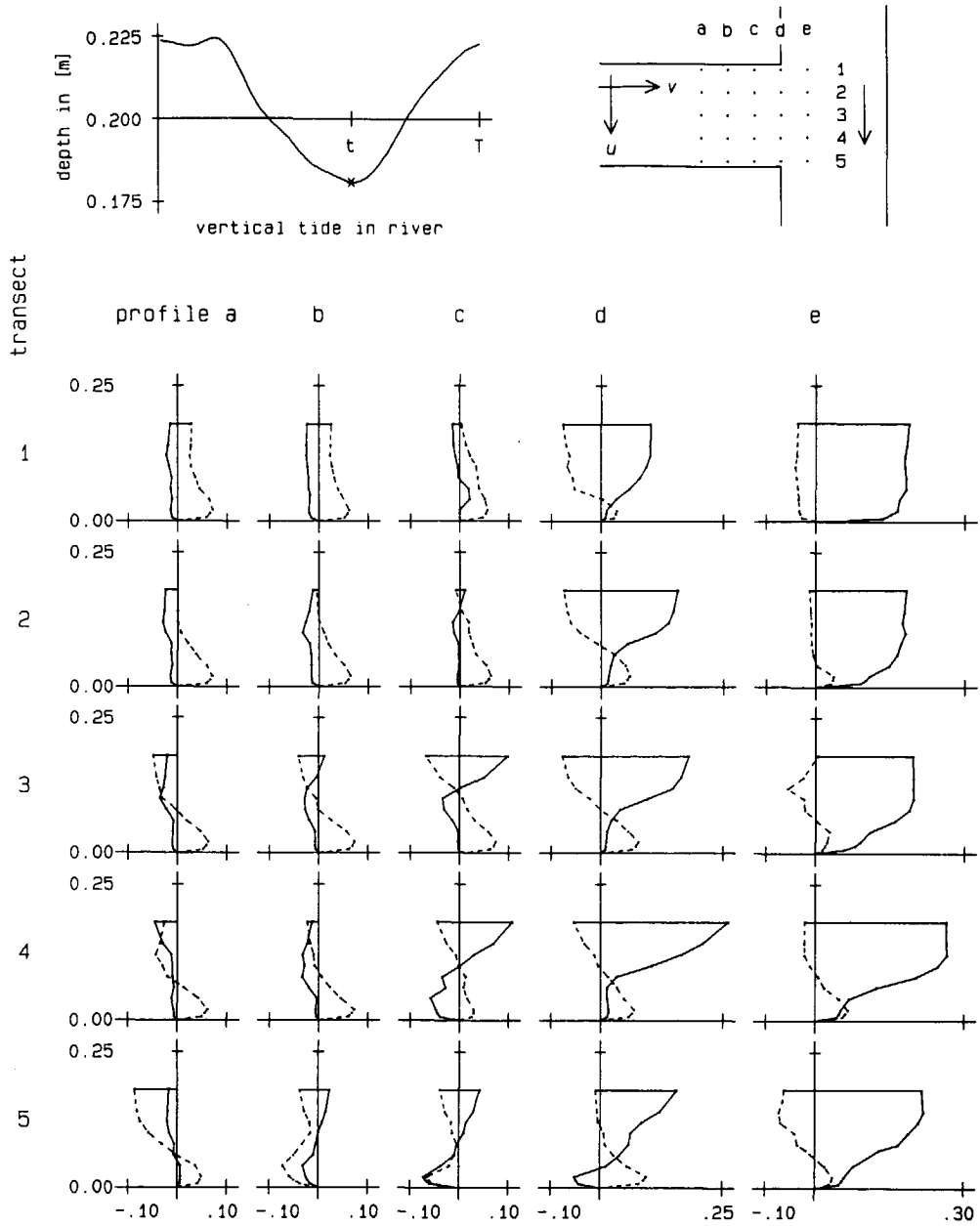
Figure 3.38 Velocity distributions in the water column in harbour 6 at low tide ( t = 390 s): —, u in m/s; and - - -, v in m/s.
