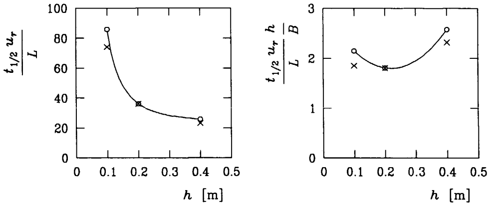
Figure 2.10 Variation of dimensionless half-life parameters with depth. \circ — = calculation of McGuirk & Rodi (1979), and \times = experiments of Nestmann (1977).
