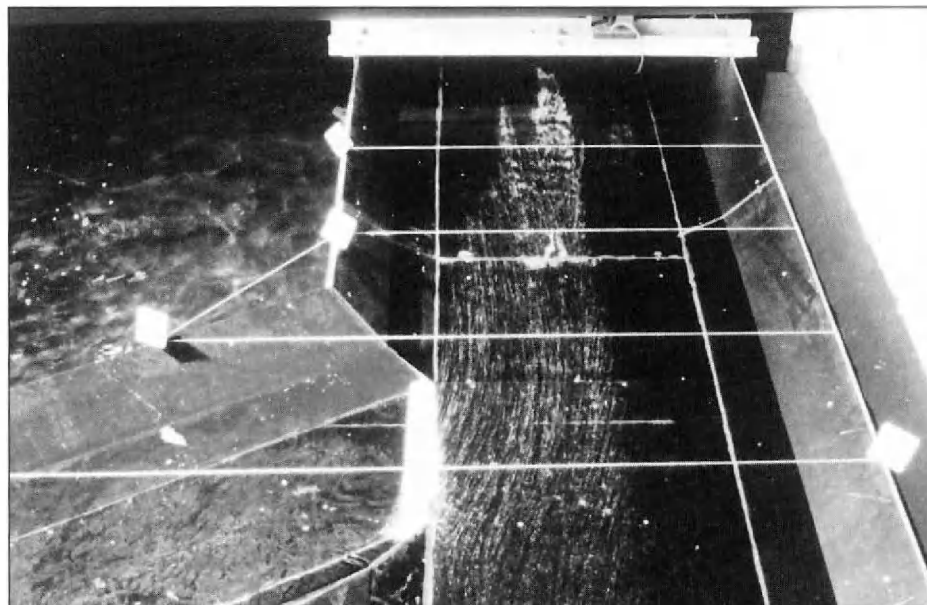
Foto 3. Modellering bodemtransport in "slimme" zandvang.
