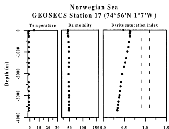
Fig. 5. Temperature, barium molality and barite saturation index vs. depth for GEOSECS station 17 in the Norwegian Sea.
