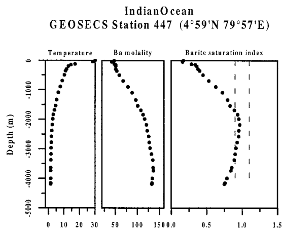
Fig. 10. Temperature, barium molality and barite saturation index vs. depth for GEOSECS station 447 south of Ceylon. There is a return to undersaturation near the seafloor.
