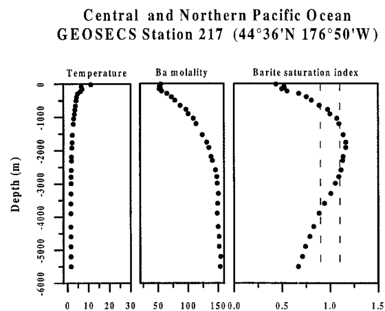
Fig. 6. Temperature, barium molality and barite saturation index vs. depth for GEOSECS station 217. This station is taken as representative of the Pacific Ocean from 45°S to 50°N as the same barite saturation state has been found at GEOSECS stations 204, 212, 217, 215, 219, 224, 226, 227, 241, 263, 296, 331, 337 and 343.
