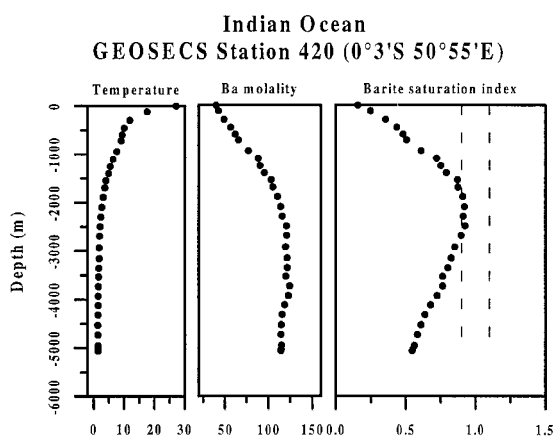
Fig. 8. Temperature, barium molality and barite saturation index vs. depth for GEOSECS station 420 in the Indian Ocean. The results for GEOSECS stations 418 and 424 are the same. The same pattern has been found for station 293 in the Southern Pacific, but also at station.
