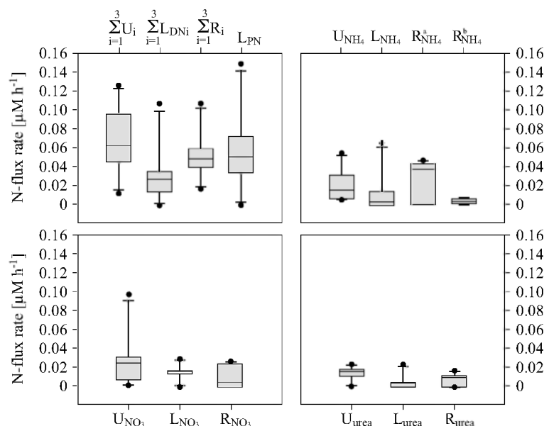
Fig. 6. Box and whisker plots of N-flux rates for 1998 from the Elskens model approach. The values correspond to the minimum estimates of the model. U_{NH_4} , U_{NO_3} and U_{urea} – corresponding nutrient uptake rates; L_{NH_4} , L_{NO_3} and L_{urea} – corresponding nutrient loss rates; L_{PN} – loss rate of PN; R_{NO_3} and R_{urea} – corresponding nutrient regeneration rates; R_{NH_4}^a – ammonium regeneration estimated by Lancelot & Billen's model; R_{NH_4}^b – ammonium regeneration estimated by Elskens' model; \sum_{i=1}^3 U_i , \sum_{i=1}^3 L_{DNi} and \sum_{i=1}^3 R_i – sum of uptake, loss and regeneration rates of the three nutrients
