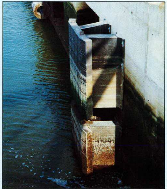
A series of fenders was supplied by Sumitomo Rubber Industries Ltd. of Japan through their Brussels office for the new sea lock. This lock was built by a joint venture of SBBM Enterprises and SOGETRA to provide access for ships of up to 125,000 d.w.t. to the new docks in the inner harbour. Photo shows Pi-type 1250 H x 2750 L fender.
