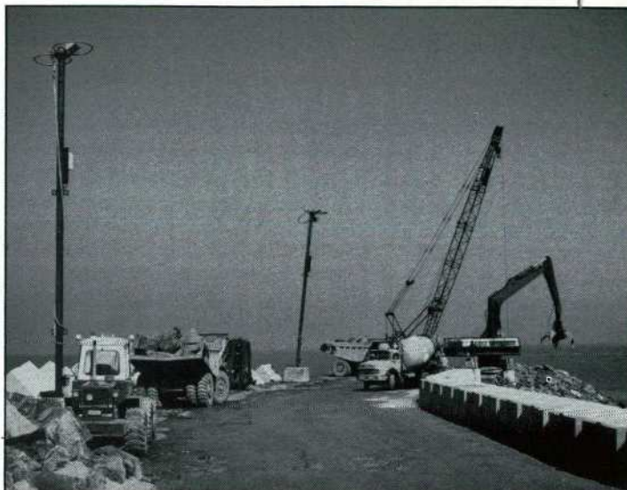
Construction of the two main breakwaters in the North Sea was one of the major challenges faced by the Zeebouuw-Zeezand consortium.
