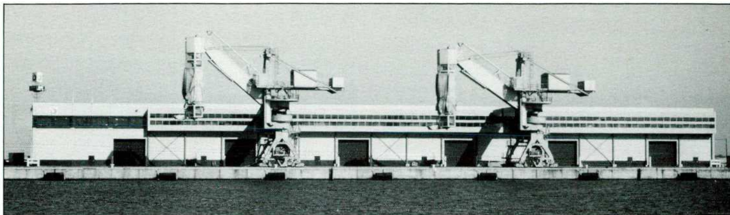
Equipment provision at the new Belgian New Fruit Wharf facility includes these two PWH continuous ship unloaders, each rated at up to 3,800 boxes/hr.
