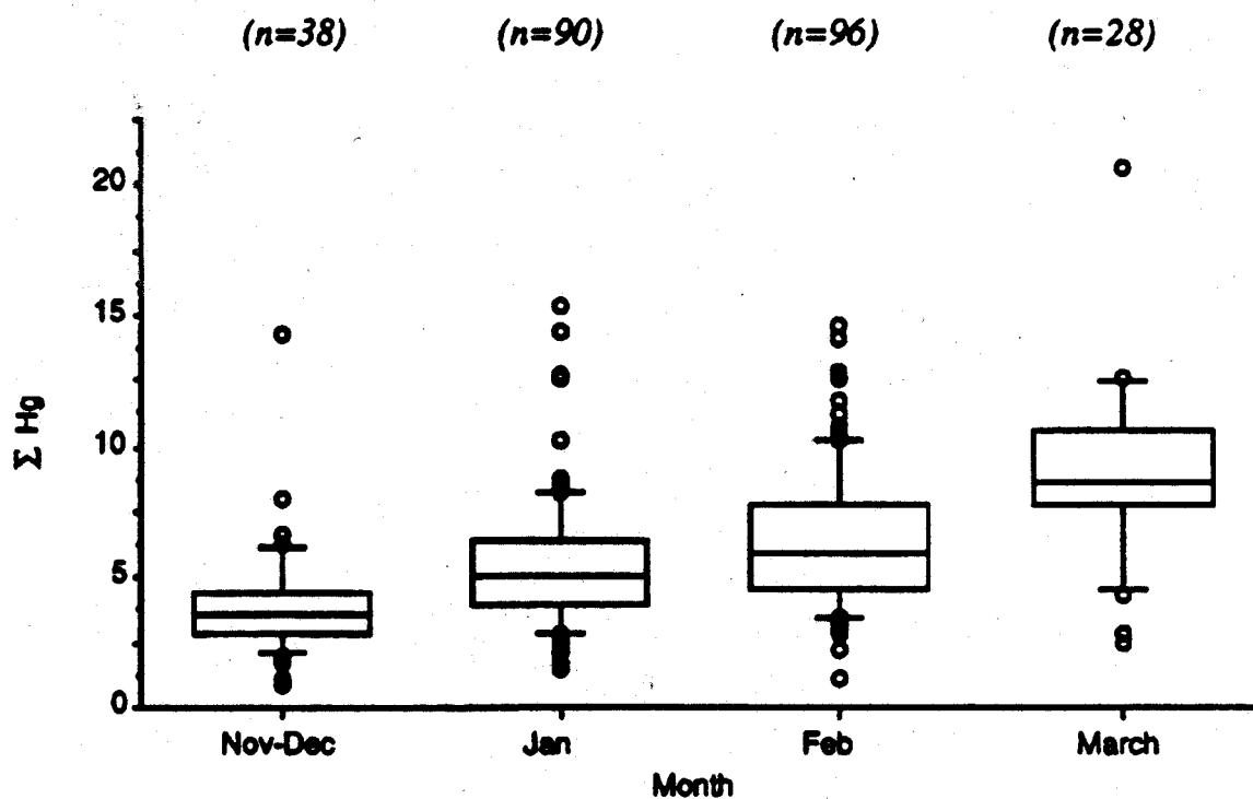
Figure 3.9. Mercury in common guillemot liver samples as a function of collection date ( \mu\text{g g}^{-1} \text{ dw} ; Joiris et al. , 1998)
