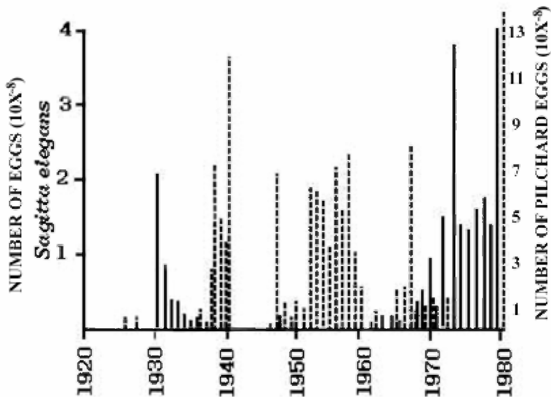
Figure 17 Provides data from Southward (1974a,b), and Southward, Butler and Pennycuik (1975) that show a bipolar (Russell Cycle) shift in English Channel fauna starting about 1938, that reversed in the late 1960s.
