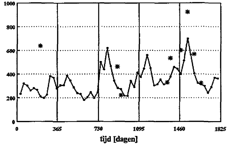
PCB153 slibkwaliteit waterkolom compartment 2 [ug/kgOC]
