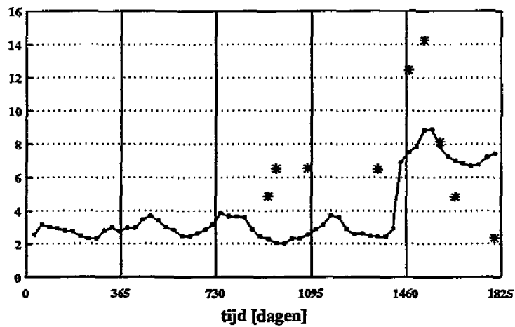
Fla slibkwaliteit waterkolom compartment 4 [mg/kgOC]
