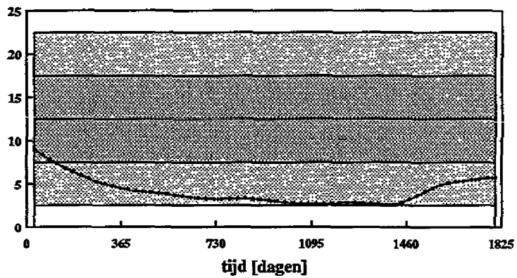
Fla slibkwaliteit waterbodem compartment 4 [mg/kgOC]
