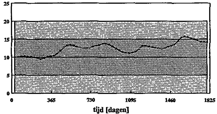
Fla slibkwaliteit waterbodem compartment 2 [mg/kgOC]
