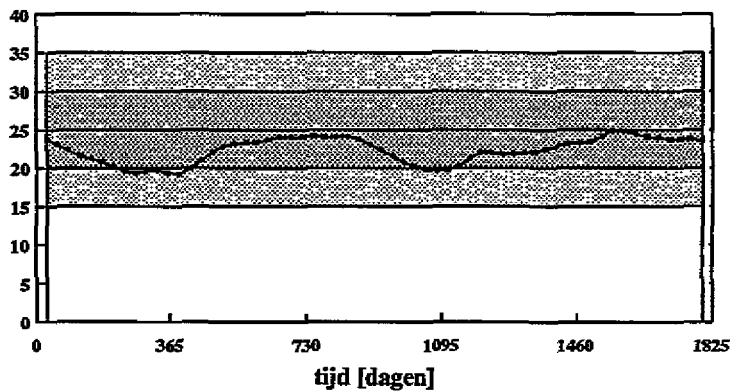
Fla slibkwaliteit waterbodem compartment 1 [mg/kgOC]
