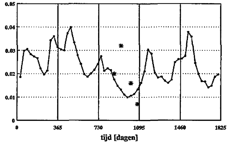
c-HCH totaalconc. waterkolom compartment 3 [µg/l]
