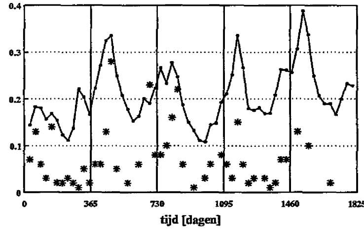
Fla totaalconc. waterkolom compartment 2 [mg/l]
