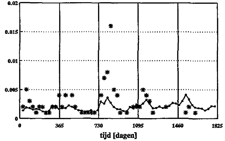
PCB153 totaalconc. waterkolom compartment 2 [ug/l]
