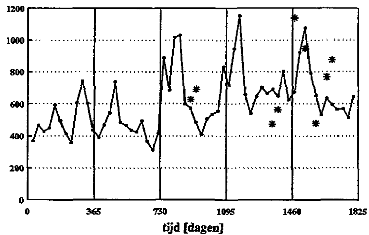
PCB153 slibkwaliteit waterkolom compartment 1 [ug/kgOC]
