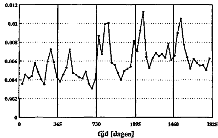
PCB153 totaalconc. waterkolom compartment 1 [ug/l]
