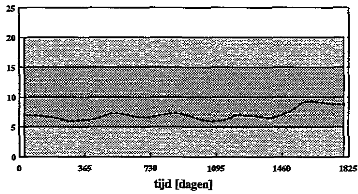
Fla slibkwaliteit waterbodem compartiment 3 [mg/kgOC]
