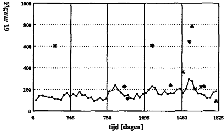
PCB153 slibkwaliteit waterkolom compartment 3 [µg/kgOC]
