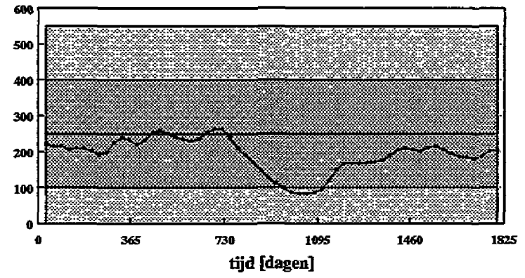
c-HCH slibkwaliteit waterbodem compartiment 1 [ug/kgOC]
