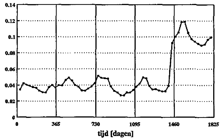
Fla totaalconc. waterkolom compartment 4 [mg/l]
