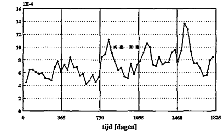
PCB153 totaalconc. waterkolom compartment 3 [µg/l]
