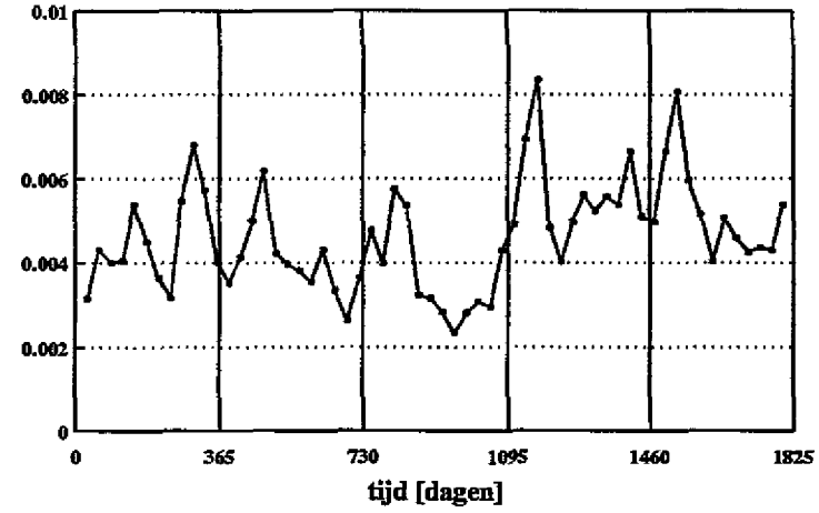
PCB52 totaalconc. waterkolom compartment 1 [ng/l]
