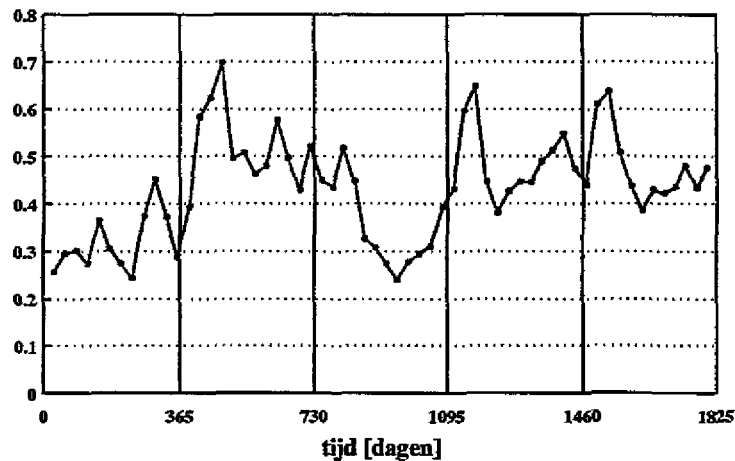
Fla totaalconc. waterkolom compartment 1 [mg/l]
