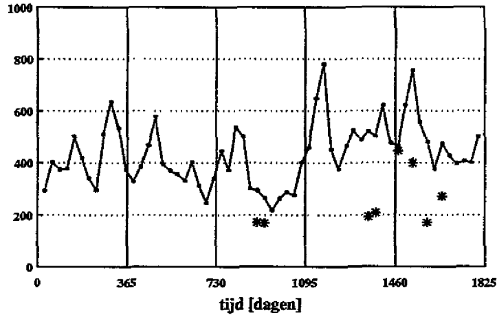
PCB52 slibkwaliteit waterkolom compartment 1 [ug/kgOC]
