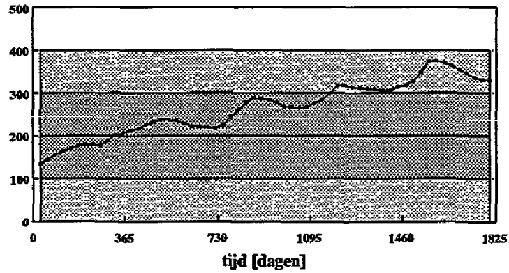
PCB153 slibkwaliteit waterbodem compartment 2 [ug/kgOC]
