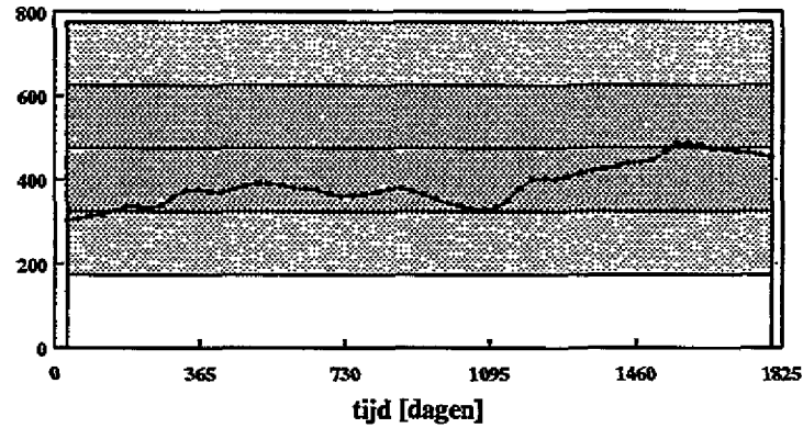
PCB52 slibkwaliteit waterbodem compartment 1 [ug/kgOC]
