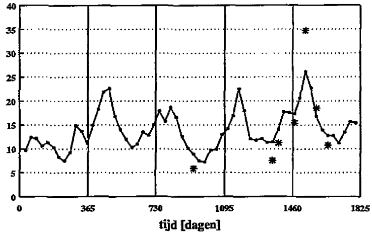
Fla slibkwaliteit waterkolom compartment 2 [mg/kgOC]
