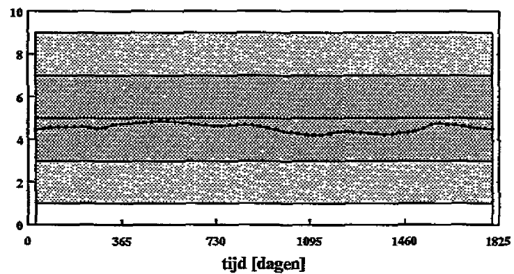
BaP slibkwaliteit waterbodem compartiment 3 [mg/kgOC]
