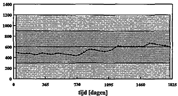
PCB153 slibkwaliteit waterbodem compartment 1 [ng/kgOC]
