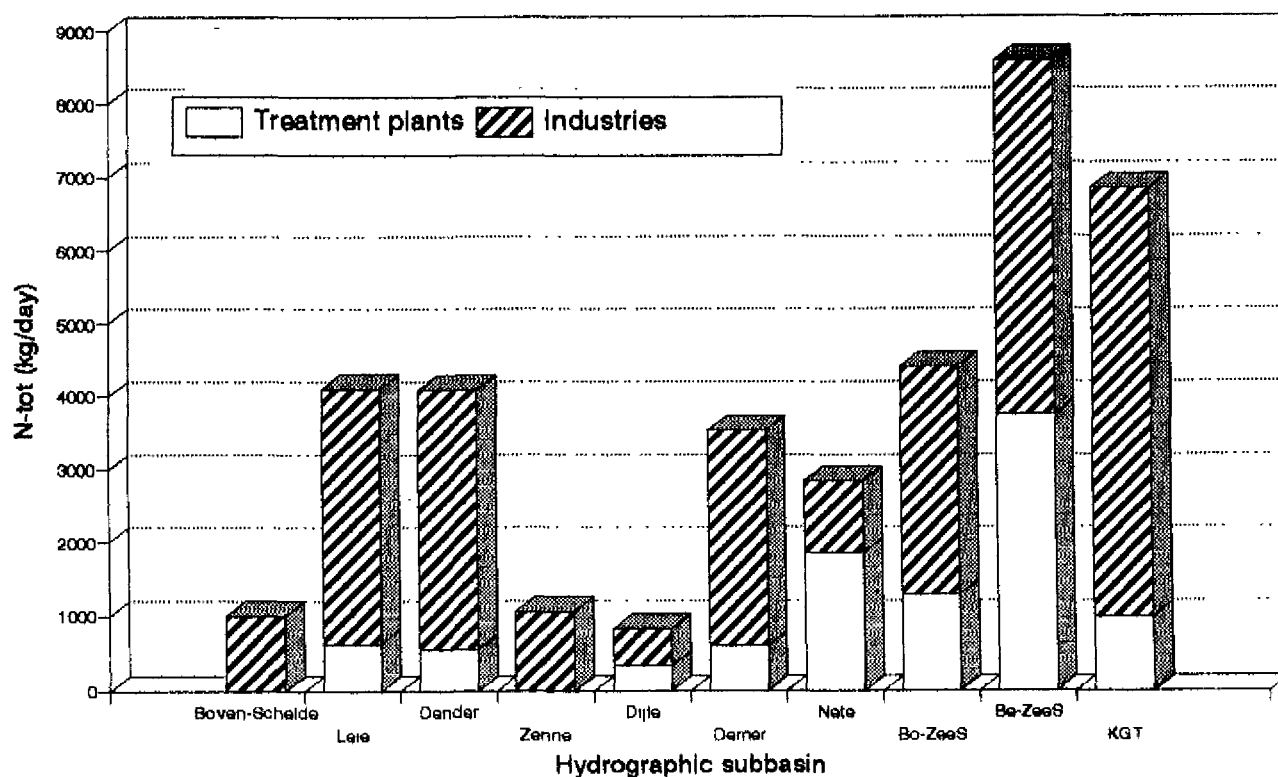
Figure 5.24 Communal and industrial discharged amounts N-total per hydrographic subbasin in Flanders (1991).
