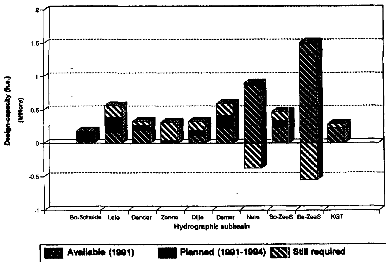
Figure 5.10 Communal waste water treatment balance in the Flemish part of the Scheldt basin. A negative still required capacity part means that there is an over-capacity.
