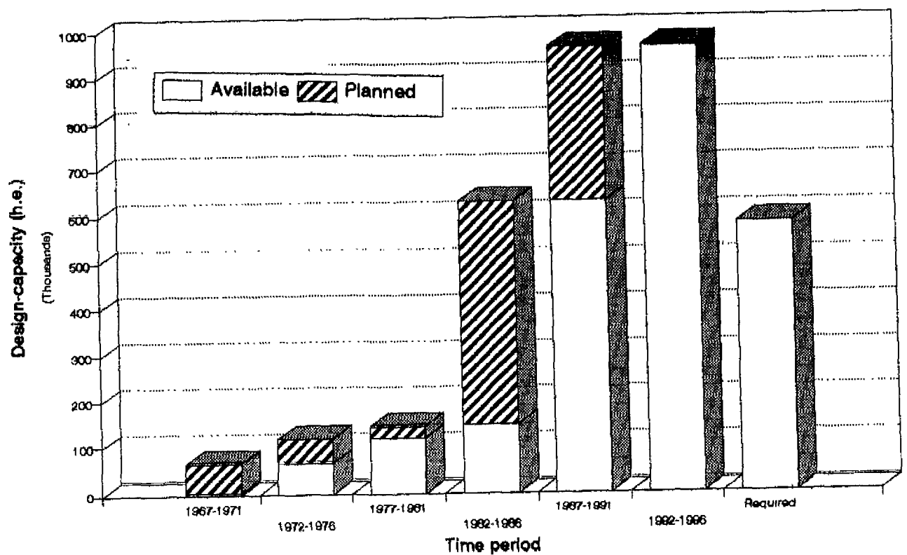
Figure 5.19 Evolution of the available and planned design-capacity in the Dutch part of the Scheldt basin (period: 1967-1996).
