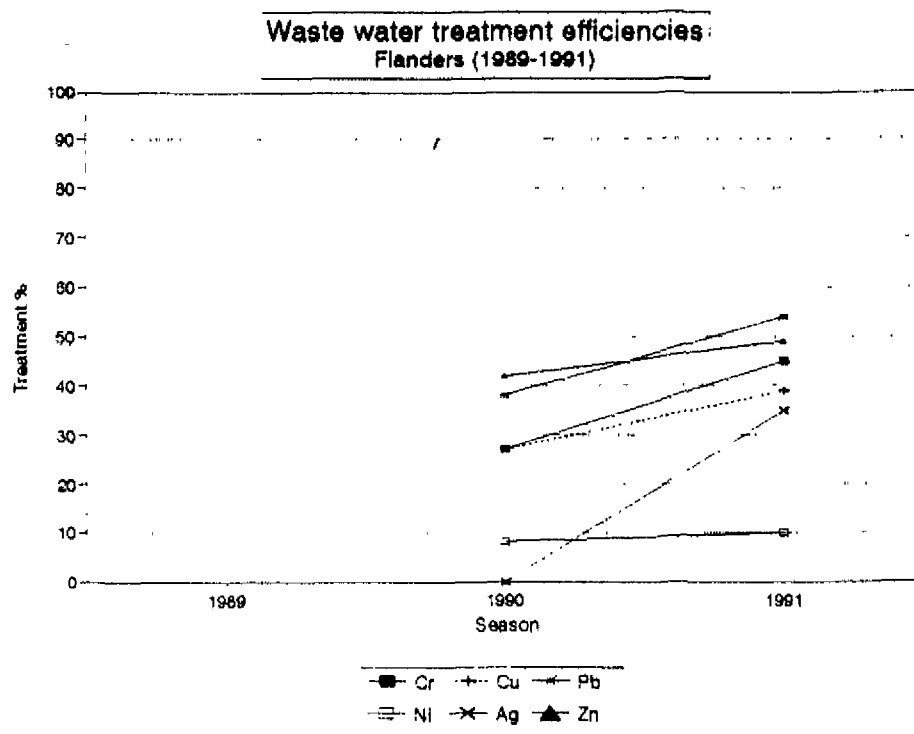
Figure 5.16 Treatment efficiencies of waste water treatment plants in Flanders (period 1990-1991). Parameters: Cr, Cu, Pb, Ni, Ag and Zn.
