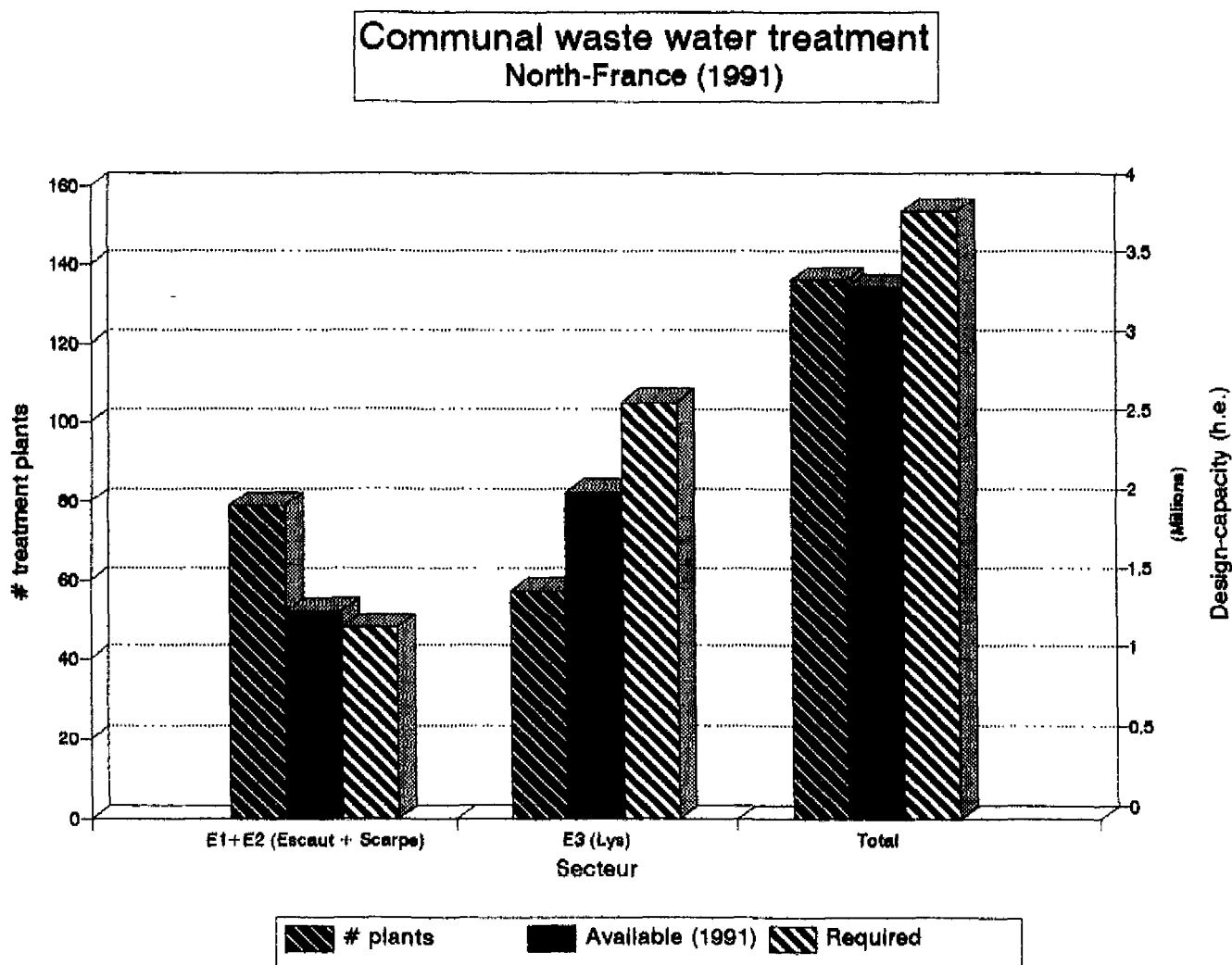
Figure 5.3 Communal waste water treatment balance of the French part of the Scheldt basin (situation 1991).
