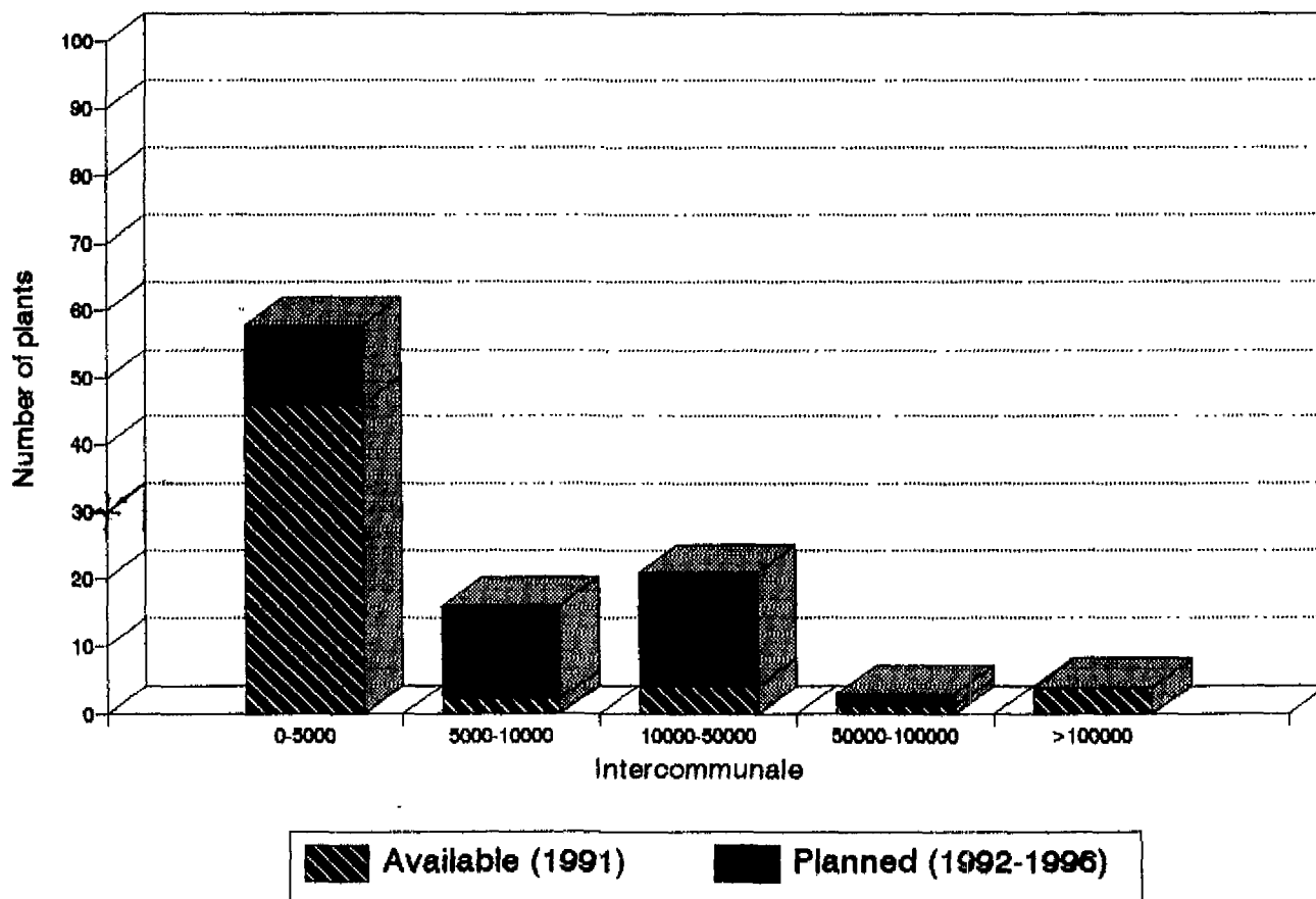
Figure 5.8 Waste water treatment plant size distribution in the Wallonian part of the Scheldt basin (situation 1991).
