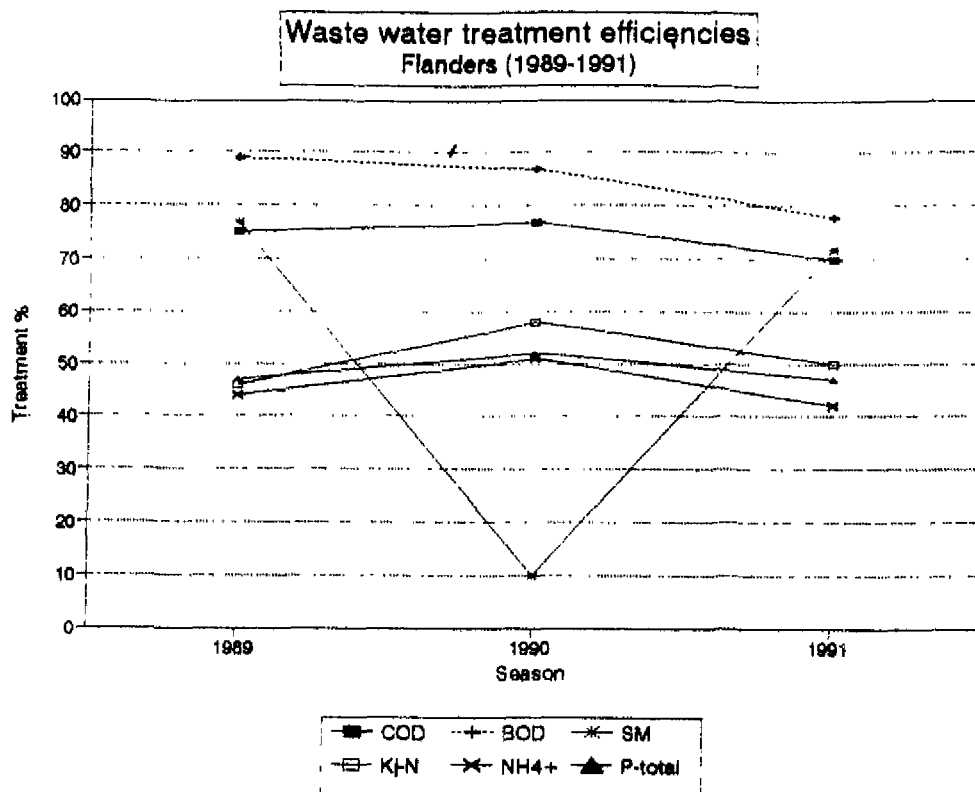
Figure 5.15 Treatment efficiencies of waste water treatment plants in Flanders (period 1989-1991). Parameters: BOD, COD, SM, Kj-N, NH4 and P-total.
