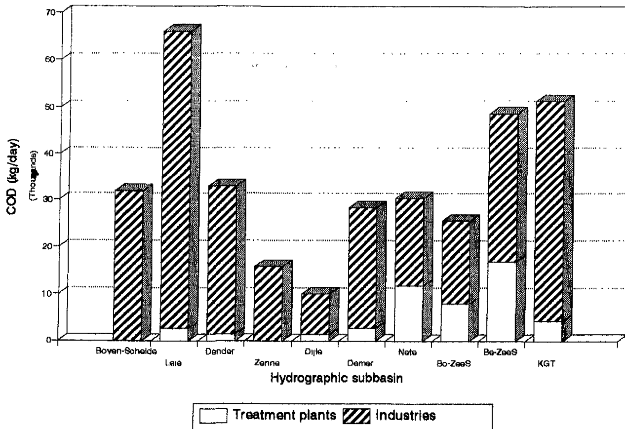
Figure 5.23 Communal and industrial discharged amounts COD per hydrographic subbasin in Flanders (1991).
