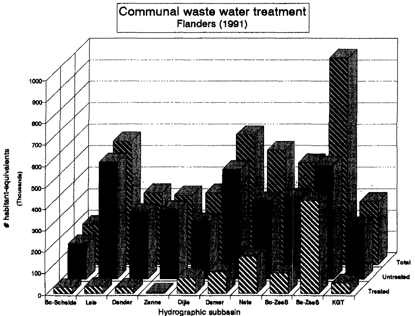
Figure 5.12 Required design-capacity and the number of habitant-equivalents that are treated per hydrographic subbasin in the Flemish part of the Scheldt basin.
