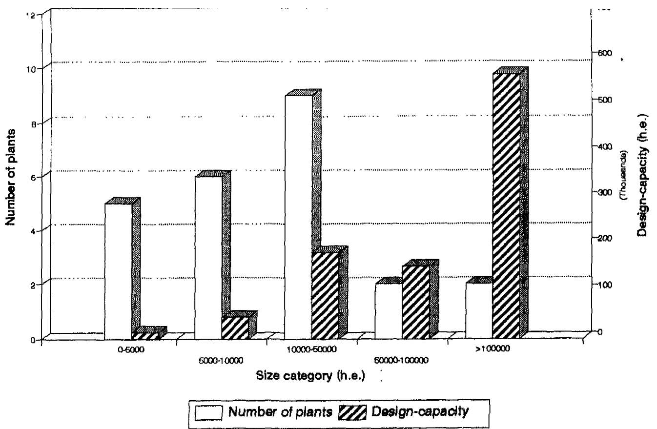
Figure 5.18 Waste water treatment plant size distribution in the Dutch part of the Scheldt basin (situation 1991).
