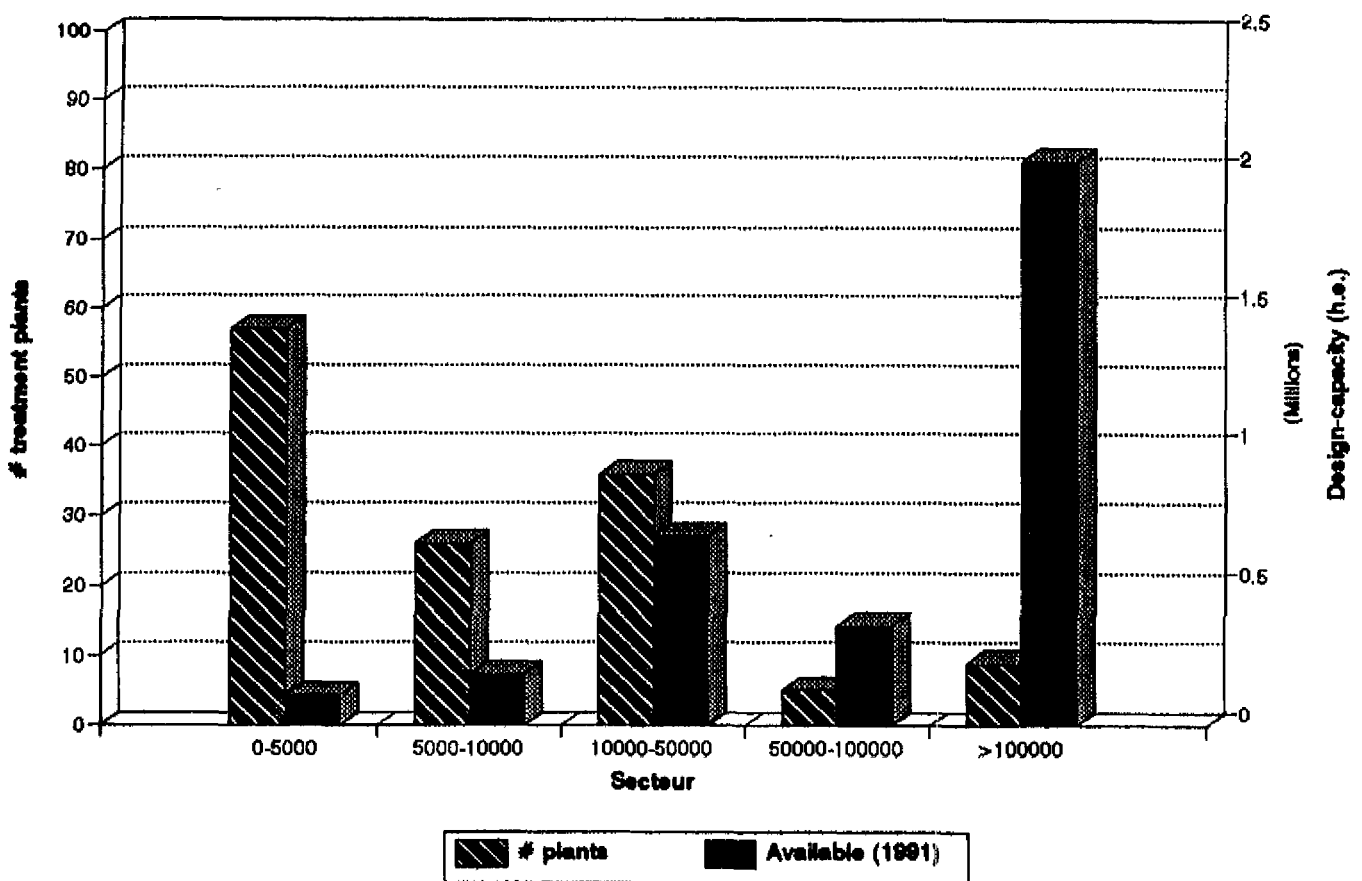
Figure 5.4 Waste water treatment plant size distribution in the French part of the Scheldt basin (situation 1991).
