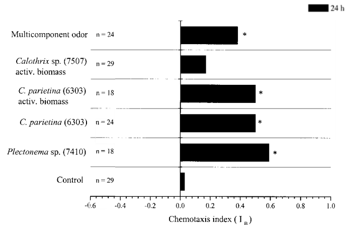
Fig. 5. Single-worm assays of B. monhystra . Chemotaxis responses after 24 h to axenic cultures of cyanobacteria and to the multicomponent odor ( n = number of assays). Values significantly different from control experiments: * p < 0.05.
