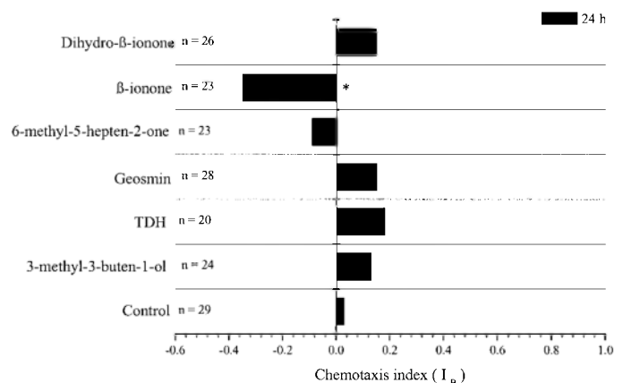
Fig. 6. Single-worm assays of B. monhystra . Response to odors of the isoprenoid pathway after 24 h ( n = number of assays). Values significantly different from control experiments: * p < 0.05.
