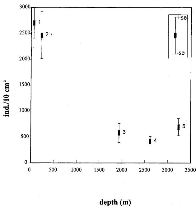
Fig. 2 Mean meiobenthic densities per station \pm standard error
