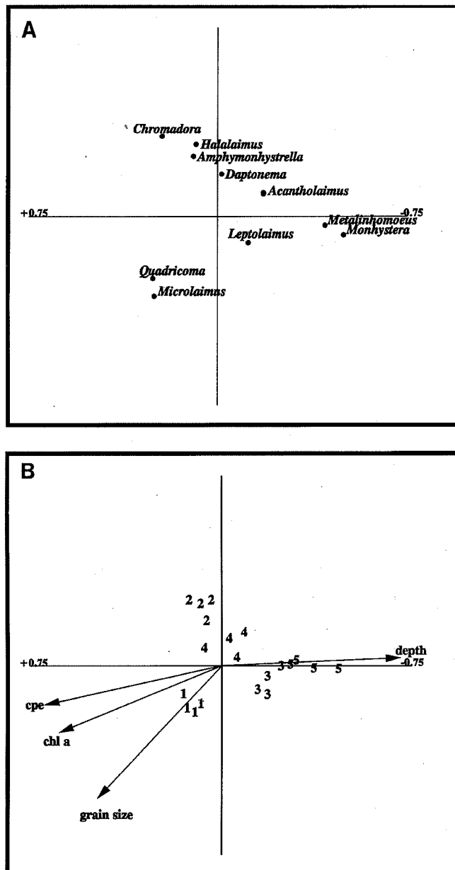
Fig. 5 A,B CCA plot based on nematode total generic abundances. Same numbers indicate different replicates from the corresponding station. A Species plot; B Stations plot
