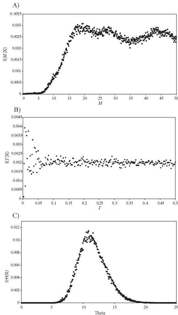
Figure 4. Typical outcomes of MDIV analyses between adjacent pairs of islands. (A) M ( 2N_e m ) and (B) T ( t/2N_e ) posterior probabilities did not distinguish with confidence between ongoing migration and recent divergence. (C) In all cases analyses showed clear maximum probability for estimates of \Theta ( 2N_e \mu ).
