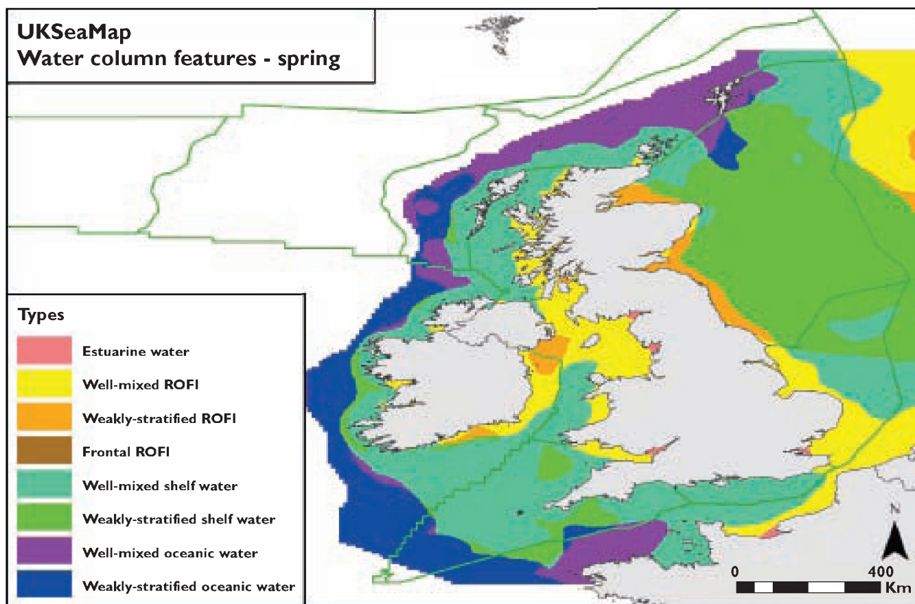
Figure 36. Spring water column features.
