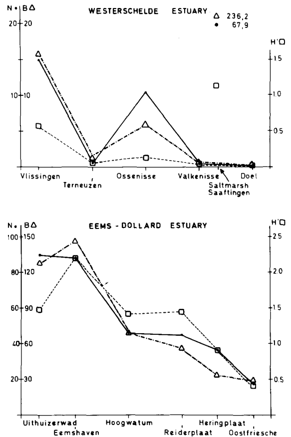
Fig. 2. Longitudinal profile of average annual density N (ind. 10\text{ cm}^{-2} ) average annual biomass B ( \mu\text{g dwt } 10\text{ cm}^{-2} ) and average annual diversity H (bits ind. -1 ; Brillouin index) of the epibenthic harpacticoids in the Westerschelde and Eems-Dollard estuaries (see also Table 5).
