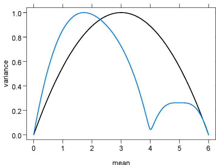
Figure 12.1. The mean-variance relationship under the assumption of quasi-binomial errors (black) and based on the individual VDSI data (blue). The two relationships are scaled to have a common maximum of unity.
