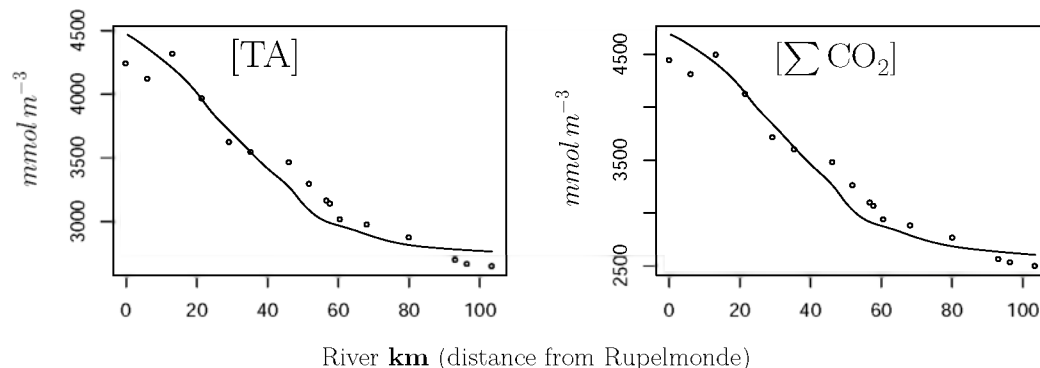
Fig. 4. Yearly averaged [TA] and [ΣCO 2 ] (model output, 2003) vs. field data provided by Frederic Gazeau (pers. comm. and Gazeau et al., 2005). [TA] data are measurements, [ΣCO 2 ] data are consistently calculated using conditions of the model.
