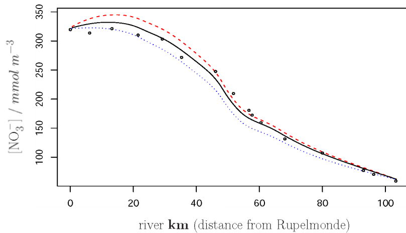
Fig. 13. [\text{NO}_3^-] fit with different denitrification parametrisations.
