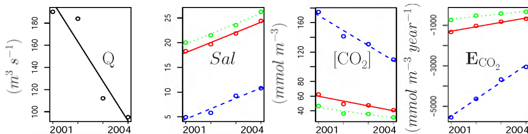
Fig. 12. Trends in key quantities from 2001 to 2004 ( Q signifies the freshwater flow at the upstream boundary; Sal , [CO_2] , E_{CO_2} : volume averaged, solid line: total estuary, dashed line: upper part (to box 50), dotted line: lower part).
