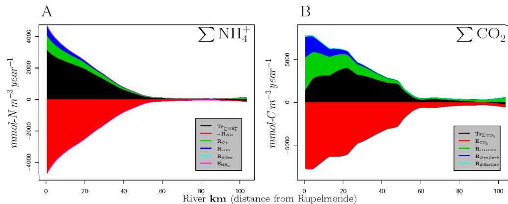
Fig. 6. Budgets for [\Sigma \text{NH}_4^+] ( A ) and [\Sigma \text{CO}_2] ( B ) along the estuary, averaged over 2001–2004 (cumulatively plotted); Values are in \text{mmol-N m}^{-3} \text{year}^{-1} .
