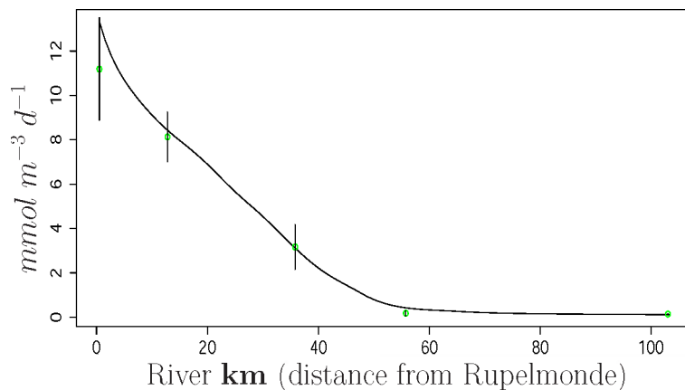
Fig. 5. Yearly averaged R_{\text{Nit}} (model output, 2003) vs. field data (Andersson et al., 2006).
