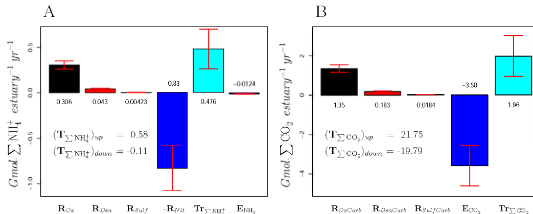
Fig. 10. Total annual budgets for \sum NH_4^+ ( A ) and \sum CO_2 ( B ) for the whole estuary, averaged over 2001–2004. (Tr_x)_{up} and (Tr_x)_{down} signify advective-dispersive import or export at the upstream and downstream boundary. The error bars give the standard deviation \sigma , obtained from the four model years.
