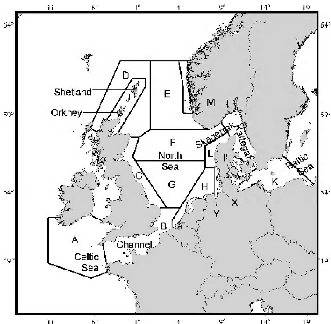
Fig. 1. Area covered during the SCANS survey in 1994. Blocks A–I were surveyed by ship. Blocks I' (a subset of block I), J–M, X and Y were surveyed by aircraft.
