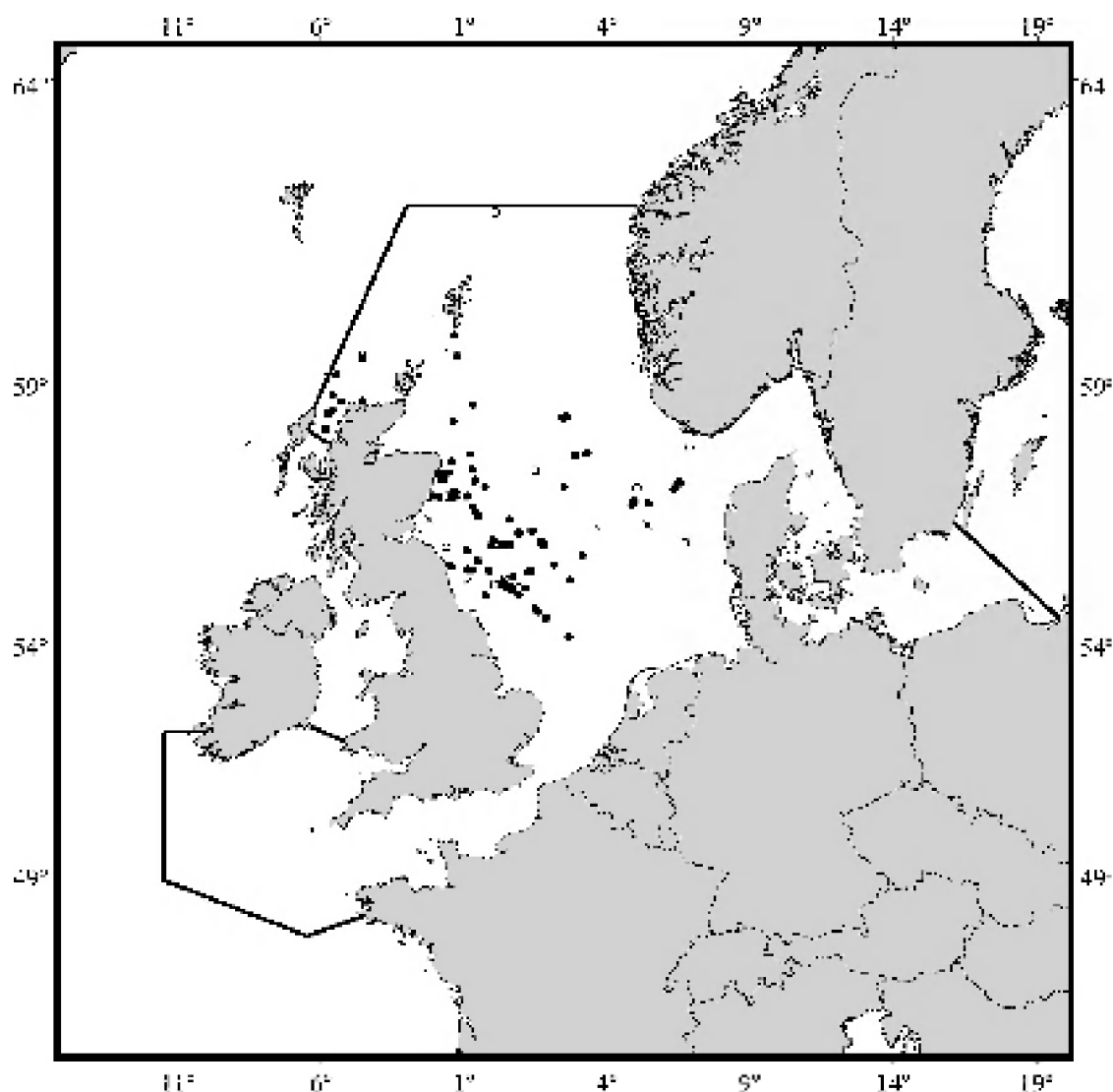
Fig. 4. Sightings of unidentified Lagenorhynchus spp. (open circles), L. albirostris (filled circles) and L. acutus (crosses) made on effort during shipboard and aerial survey.
