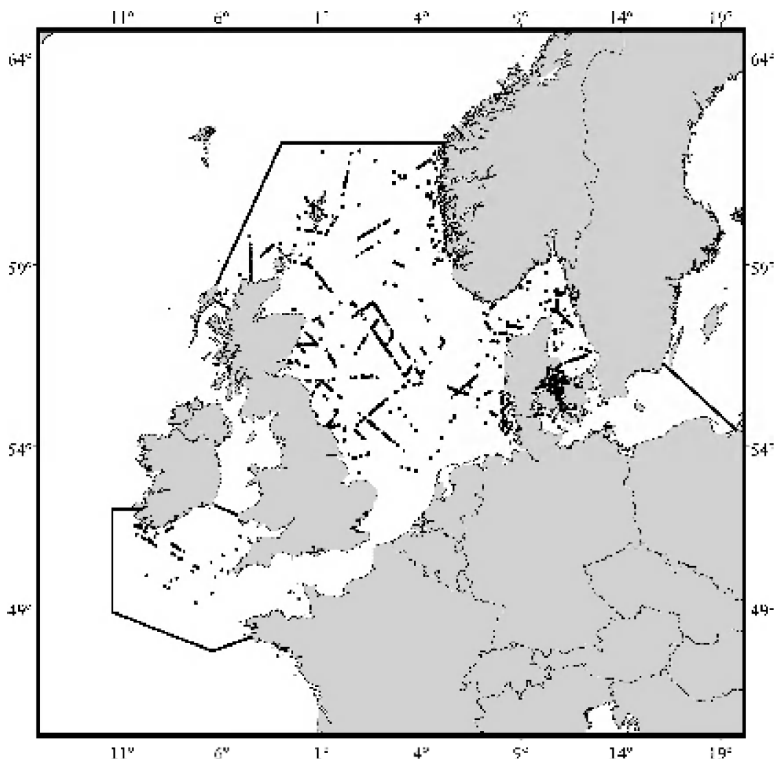
Fig. 3. Sightings of Phocoena phocoena made on effort during shipboard and aerial survey.
