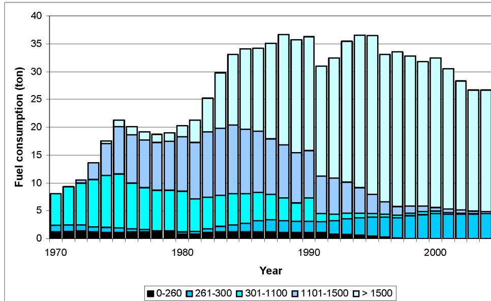
FIG. 4 - TOTAL FUEL CONSUMPTION OF THE BEAM TRAWLER FLEET BY ENGINE POWER CLASS (SMIT AND BUISMA, 2006).
