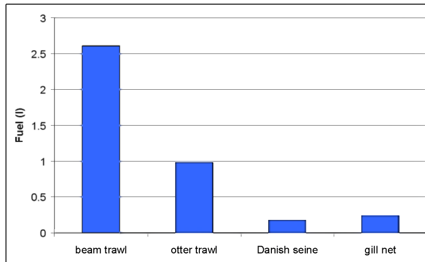
FIG. 5 - FUEL CONSUMPTION IN LITERS FOR 1 KG OF FISH (THRANE, 2004)
