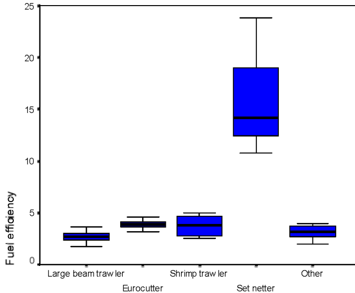
FIG. 6 – FUEL EFFICIENCY FOR SELECTED BELGIAN VESSEL TYPES (UNPUBLISHED DATA, EU-PROJECT DEGREE). FUEL EFFICIENCY = REVENUES / TOTAL FUEL COST.
