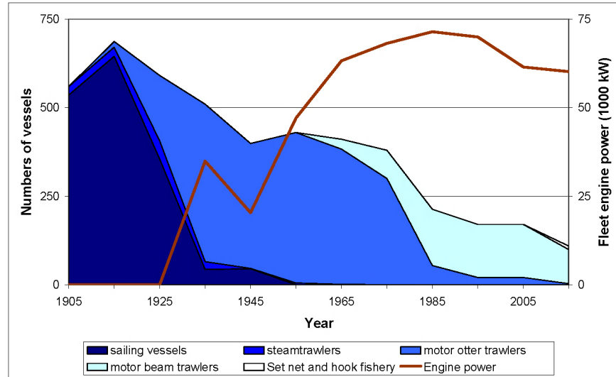
FIG. 2 – HISTORIC EVOLUTION OF THE BELGIAN FISHING FLEET IN NO.’S OF VESSELS BY VESSEL TYPE AND BY TOTAL FLEET ENGINE POWER (POLET ET AL., 1998)
