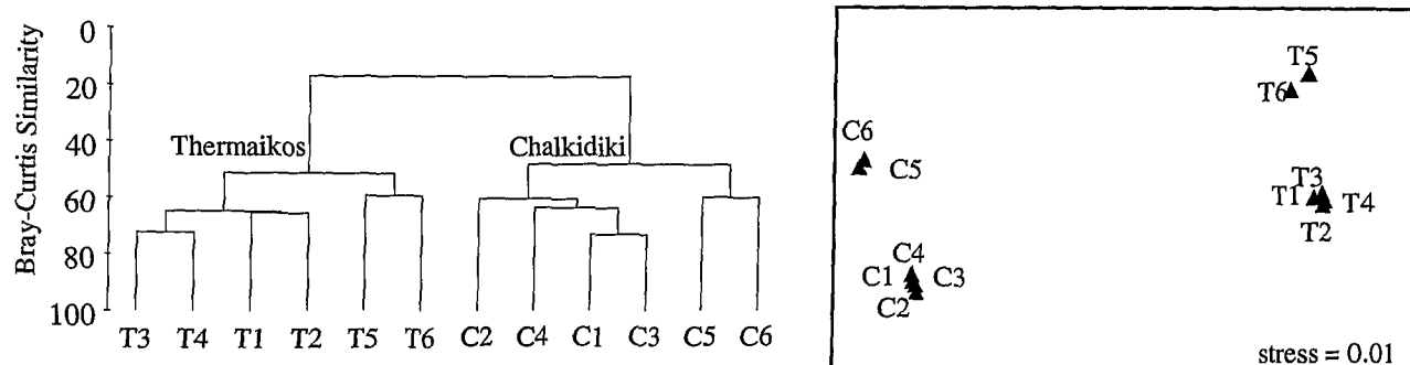
FIGURE 5 Non-metric multidimensional scaling, based on Bray-Curtis similarity index, calculated from root transformed numerical abundance data.
