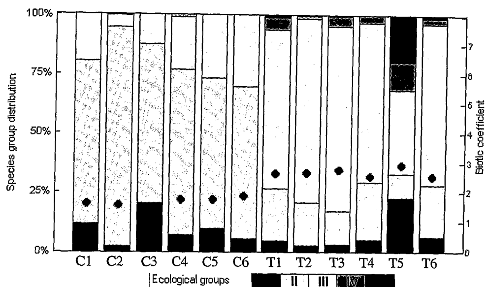
FIGURE 4 Biotic coefficient value (BC) and percentage of the ecological groups per sampling station.
