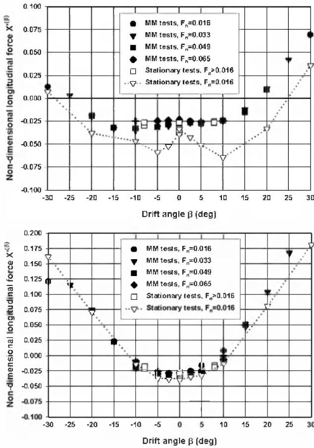
Fig. 4. Model E, comparison of non-dimensional longitudinal force X^{(\beta)} = X^{(\beta)} / (\frac{1}{2}\rho U^2 L_{VP} T) for different F_n based on test types 1 and 2. UKC: 50% (top), 20% (bottom).
