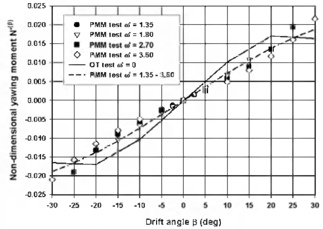
Fig. 5. Model C, comparison of non-dimensional yawing moment N^{(\beta)} = N^{(\beta)} / (\frac{1}{2}\rho U^2 L_{VP}^3) for stationary oblique towing (OT) tests and harmonic PMM tests (10% UKC)
