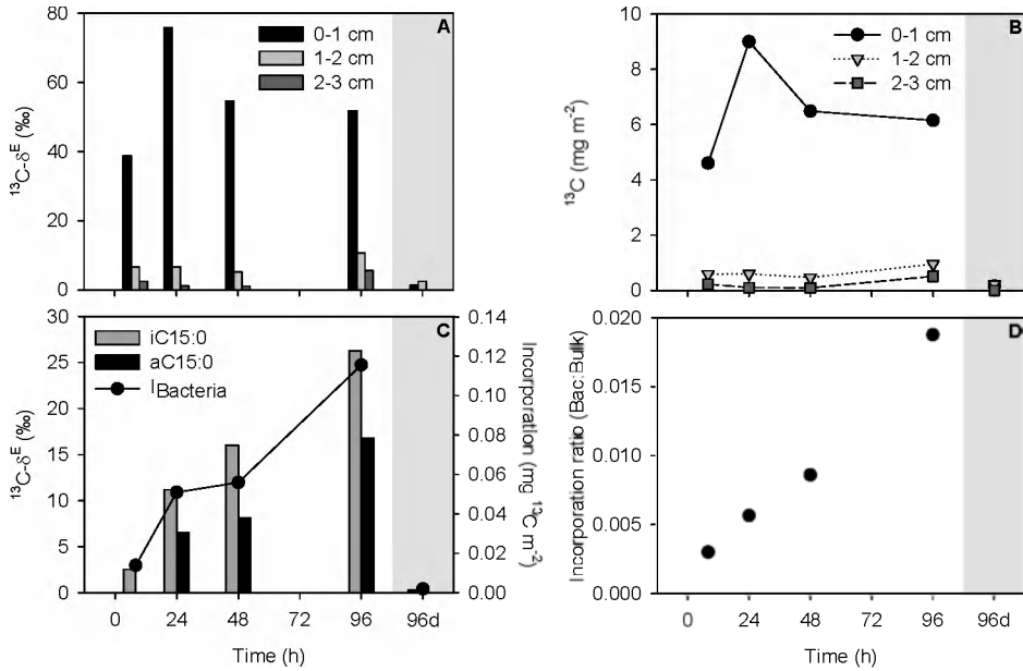
Figure 5.5. MPB addition experiment. Enrichment ( \delta^{\text{E}} ) (A) and incorporation (mg ^{13}\text{C} m -2 ) (B) for the different layers of the bulk sediment. Bacterial-specific PLFA enrichment and bacterial incorporation ( I_{\text{Bacteria}} ) for the top centimetre layer (C). Bacterial to bulk sediment incorporation ratio reflecting the gradual transfer of label to bacteria (D).
