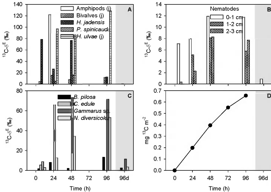
Figure 5.6. MPB addition experiment. Meiifauna (A), nematodes (B) and macrofauna (C) enrichment ( \delta^{13}\text{C} ) in the top centimetre layer. Total ^{13}\text{C} respired by the heterotrophic benthic community (D).
