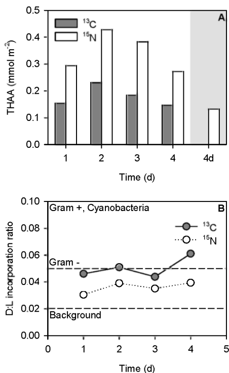
Figure 3.4. (A) ^{13}\text{C} and ^{15}\text{N} incorporation over time in THAA in the 0-1 cm layer. (B) D:L-Ala ratio of incorporation of ^{13}\text{C} and ^{15}\text{N} in the 0-1 cm layer.
