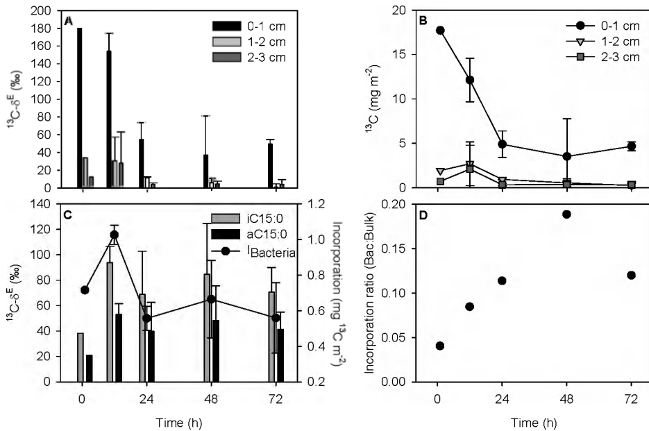
Figure 5.3. Phytodetritus addition experiment. (A) Enrichment ( \delta^{\text{E}} ) and (B) incorporation (mg ^{13}\text{C} m ^{-2} ) for the different layers of the bulk sediment. Bacterial-specific PLFA enrichment and bacterial incorporation (I Bacteria ) for the top centimetre layer (C). All but t = 1h data points are mean \pm SD with n = 2. Bacterial to bulk sediment incorporation ratio reflecting the gradual transfer of label to bacteria (D).
