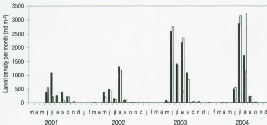
Fig. 5: Monthly comparison of larval abundance of M. leucophaea in the simulated natural and heated conditions. (■ = natural environment; □ = heated system).
