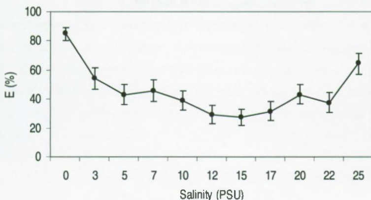
Fig. 5: Mean mortality (E %) \pm SEs at tested salinities.
