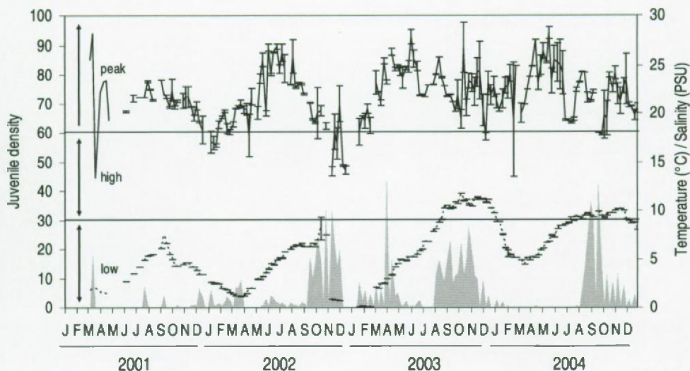
Fig. 7: Seasonal variation in presence of M. leucophaea settlement in the simulated warm cooling water system at BASF, Antwerpen N.V. with indication of the density classes (full line: temperature (°C), dashed line: salinity (PSU), grey shaded: juvenile density).
