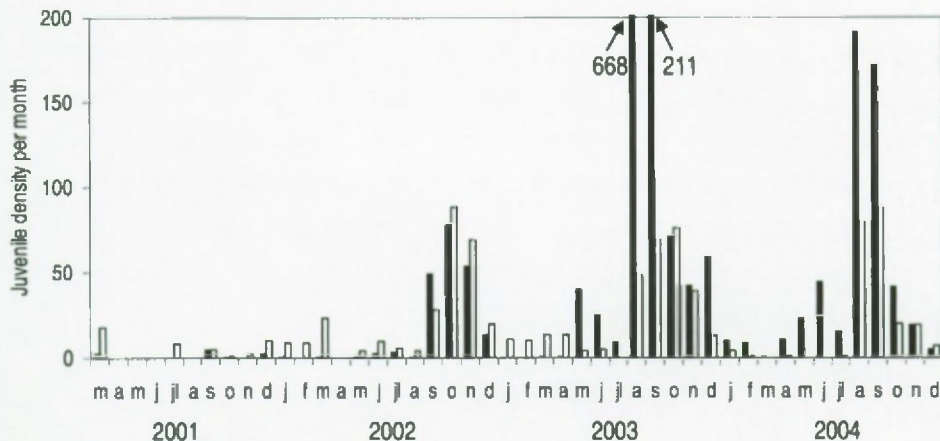
Fig. 8: Monthly comparison of abundance of M. leucophaea settlers in the simulated natural and heated conditions. (■ = natural environment; □ = heated system).
