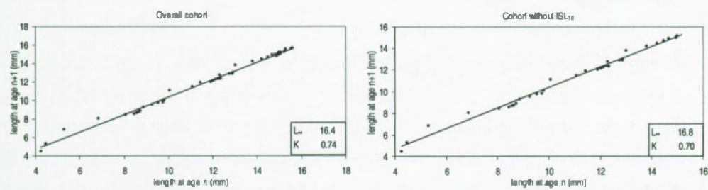
Fig. 6: Graphical presentation of the Ford-Walford method for the estimation of L_{\infty} and K. L_{\infty} = intercept / (1 – slope); K = (-1/dt)*ln (slope).
