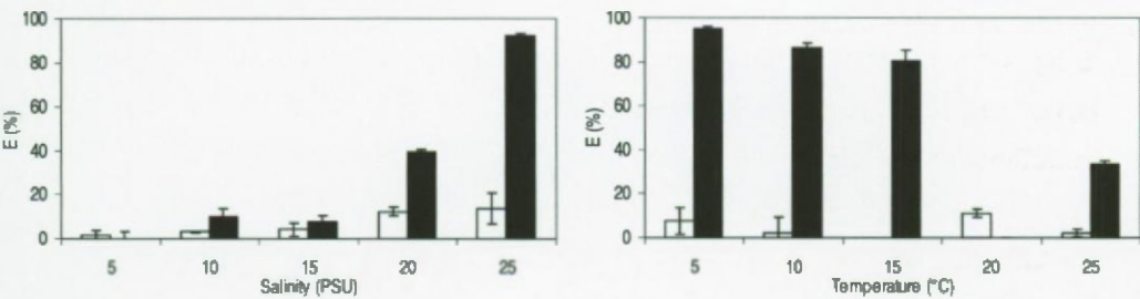
Fig. 2: Mortality rates (%) ± SE of Mytilopsis leucophaeata 4-h embryos (■) and 2-d larvae (□) at 20°C with different salinities and at 8 PSU with different temperatures.
