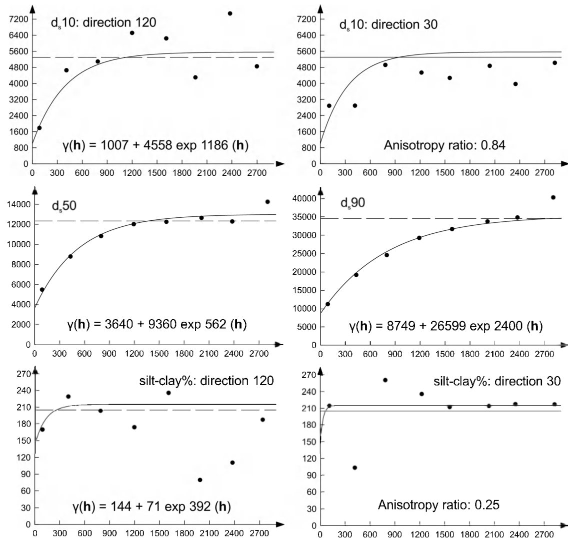
Figure 3.4: Experimental and fitted variograms for Ordinary Kriging (OK): X-axis represents lag distance (m) and the Y-axis is the semivariance (units are \mu m^2 for d_s10 , d_s50 , d_s90 and \%^2 for silt-clay%). Variogram models are expressed as \gamma(h) = C_0 + C_1 \exp a(h) , with C_0 = nugget effect, C_1 = sill, exp = exponential model and a(h) = practical range. Practical ranges are equal to the distance at which 95% of the sill has been reached. Directions are expressed as trigonometric angles (zero degrees = east increasing counter clock wise).
