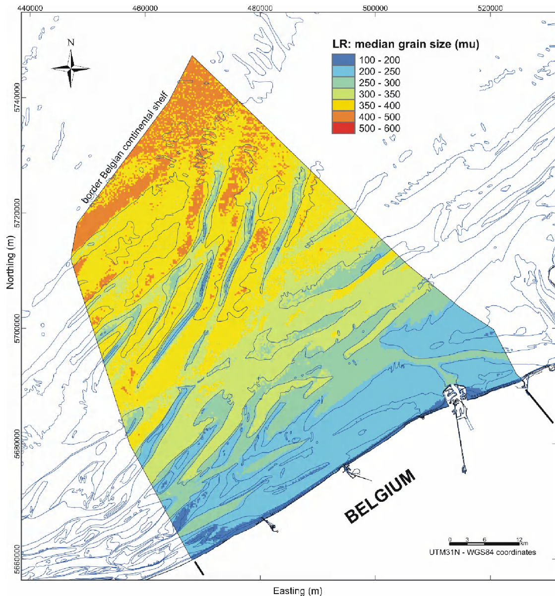
Figure 2.4: Map of median grain-size, on the basis of linear regression.
