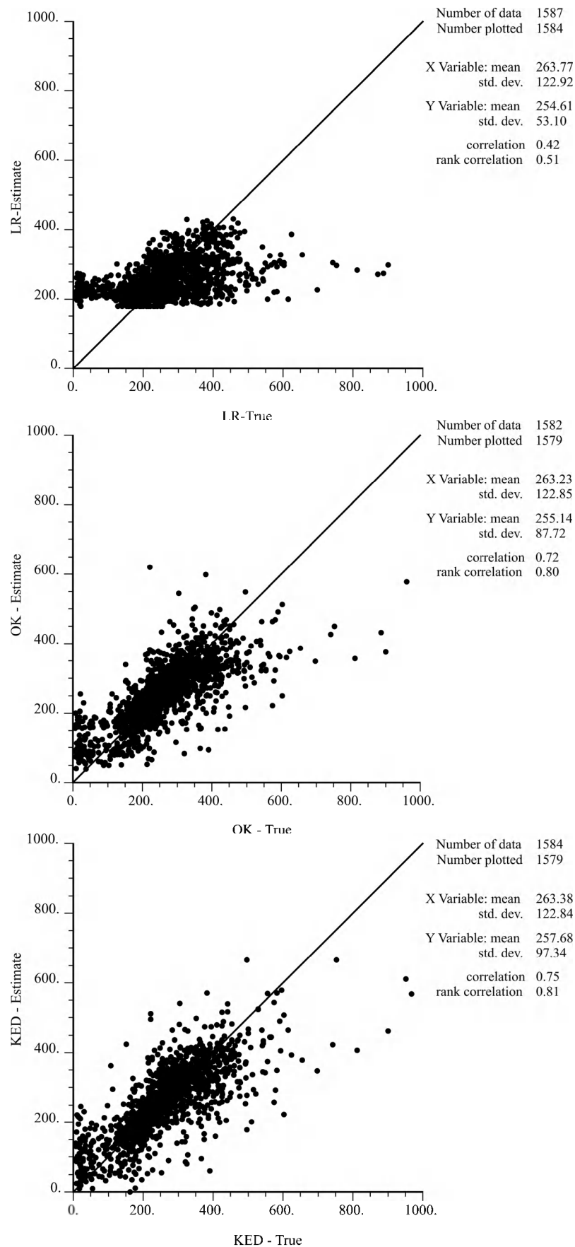
Figure 2.11: Independent validation: scatter plot of true compared to estimated value using linear regression (top), OK (middle) and KED (bottom).
