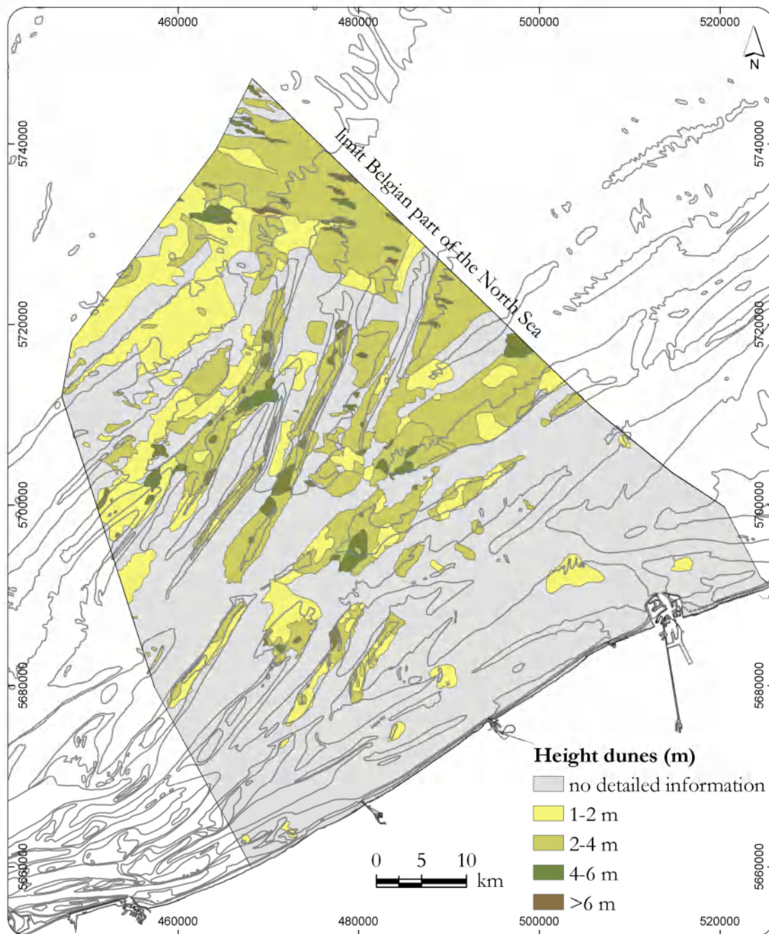
Figure 1.9: Bedforms and the height of the large to very large dunes in the Belgian part of the North Sea.
