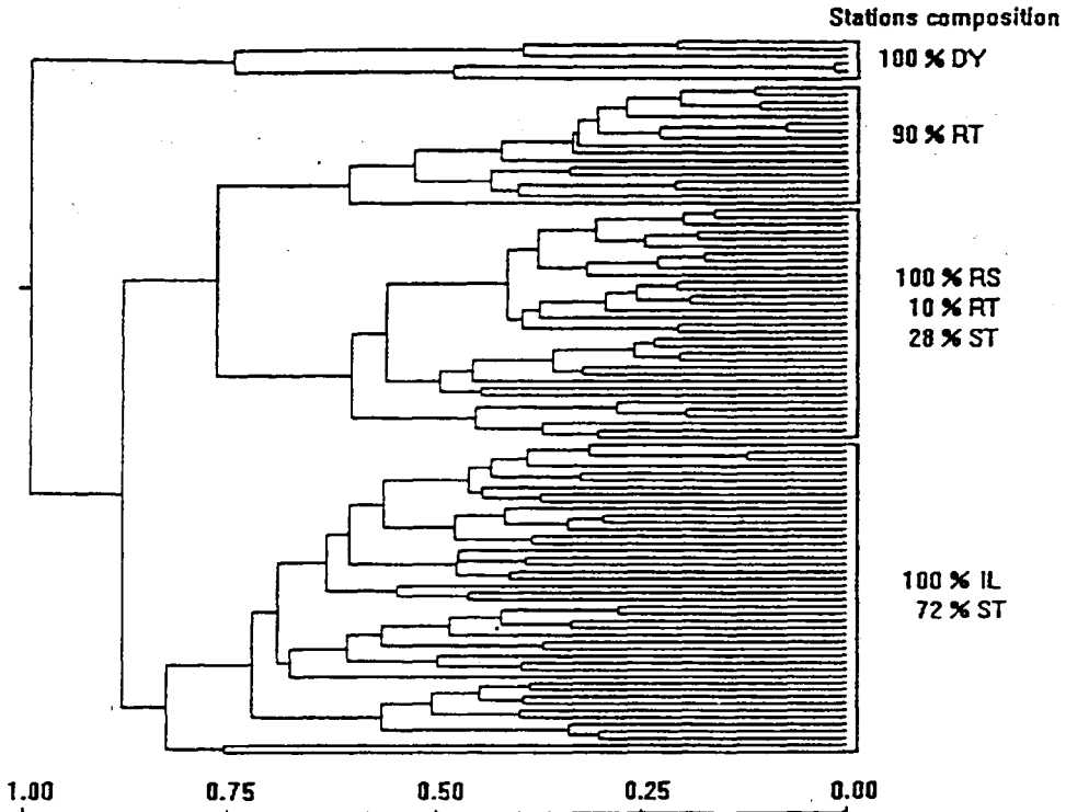
Fig. 4: Cluster analysis and ordination of stations (MDS) of the beaches. Groups identified in the dendrogram are encircled in the MDS. Scale represents dissimilarity.
