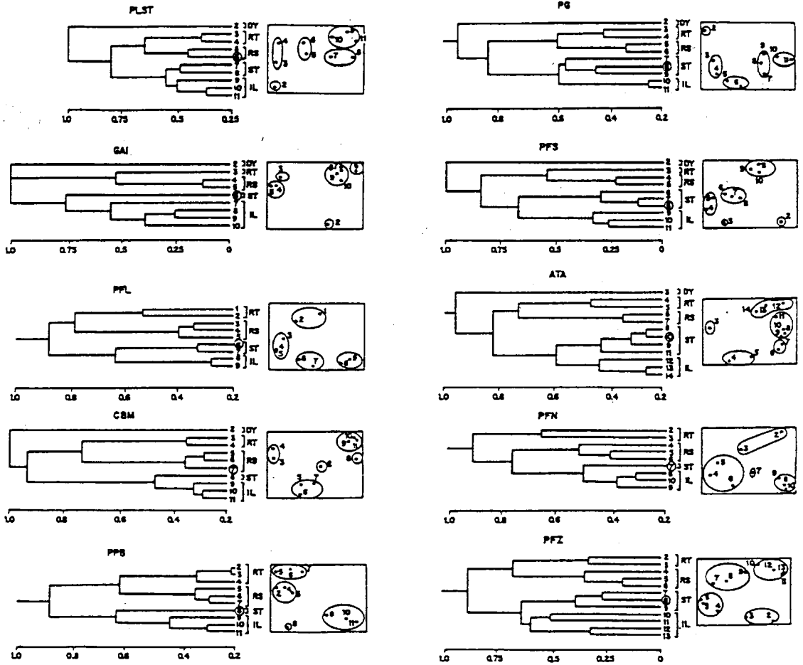
Fig. 5: Results of cluster analysis of all the stations sampled. Scale represents dissimilarity.
