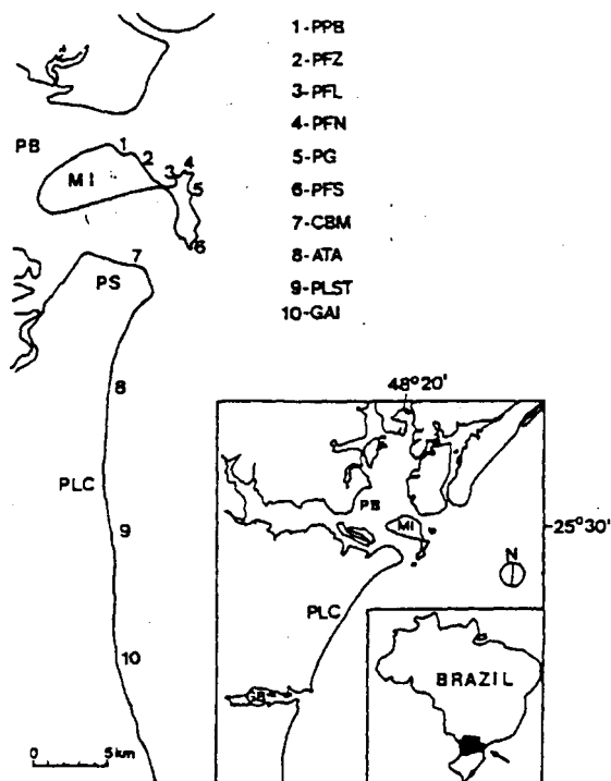
Fig. 1: Paraná coast, Brazil, showing the location of the beaches. GB: Guaratuba Bay, MI: Mel Island, PB: Paranaguá Bay. PLC: Praia de Leste Coastal Plain. PS: Ponta do Sul.
