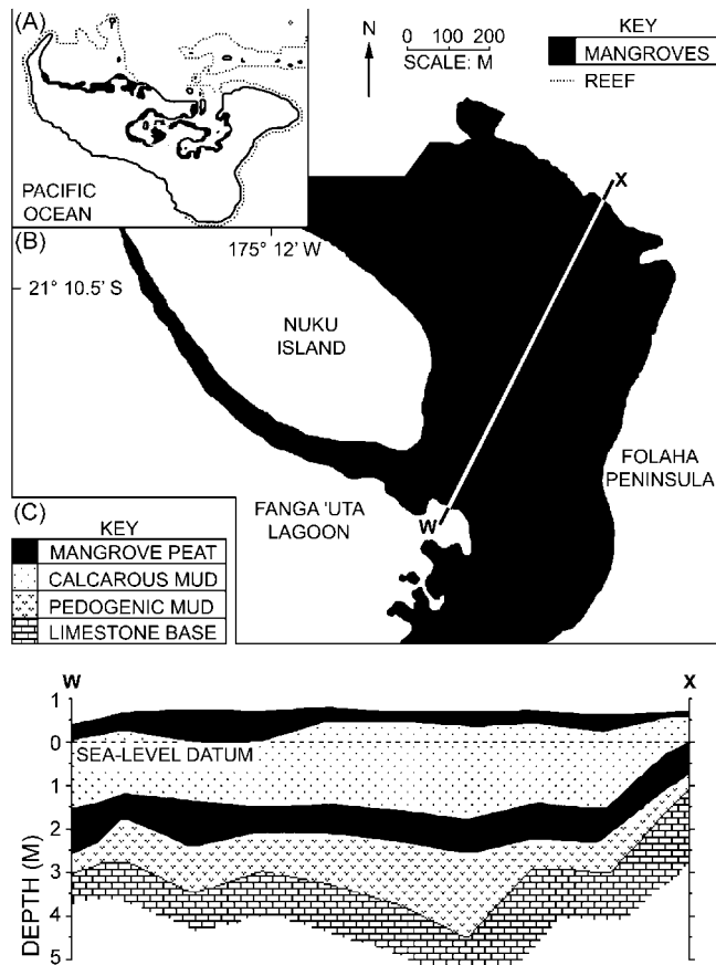
Fig. 2. (A) Mangrove distributions on Tongatapu, Tonga. (B) Mangrove swamp at Folaha, Tongatapu. (C) Holocene stratigraphy of the transect shown in B (adapted from Ellison, 1989).
