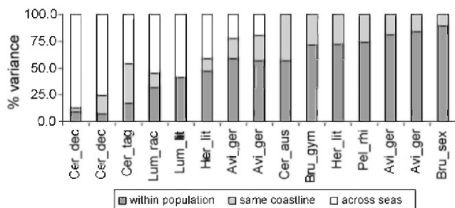
Fig. 4. Comparison of analysis of molecular variance results of ISSR and AFLP markers from 12 cases on nine species at three geographical levels—data from Dodd et al. (2002), Jian et al. (2004), Tan et al. (2005), Cerón-Souza et al. (2005), Castillo-Cárdenas et al. (2005), Su et al. (2006, 2007), Nettel and Dodd (2007) and Huang et al. (2007).
