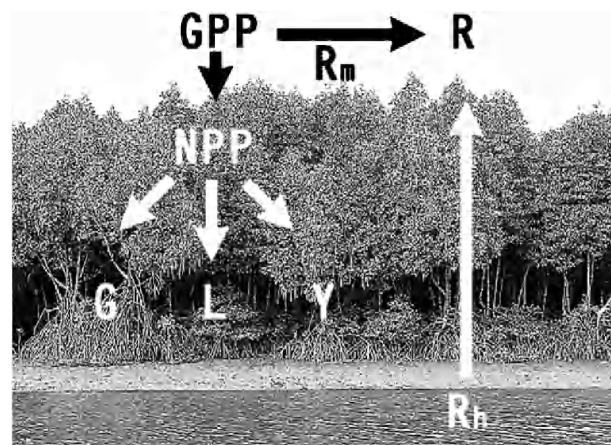
Fig. 4. The summation method used to calculate the net primary production (NPP) and the net ecosystem production (NEP) of forests. See main text for abbreviations.
