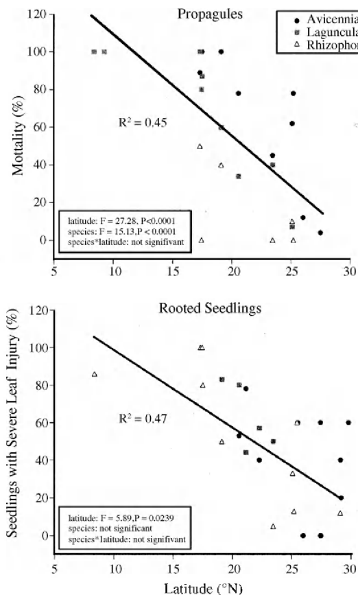
Fig. 3. Effects of mangrove species and geographic source on propagule mortality (upper panel) and percentage of rooted seedlings with severe leaf injury (lower panel) after exposure to chilling temperatures (2–4 °C for 5–6 days). Data from Markley et al. (1982), McMillan and Sherrod (1986), and Sherrod et al. (1986).
