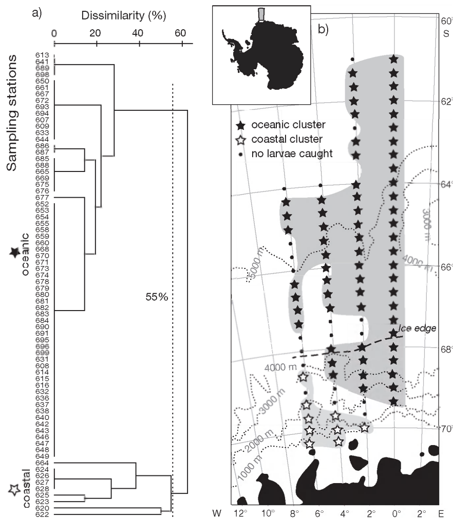
Fig. 1. (a) Cluster dendrogram of stations according to the species composition of larval fishes and (b) geographic distribution of species clusters in polar stereographic projection. Stations where fish larvae were caught were grouped in a coastal and an oceanic cluster. Geographic overview of the Antarctic continent in inset shows the survey area shaded in grey
