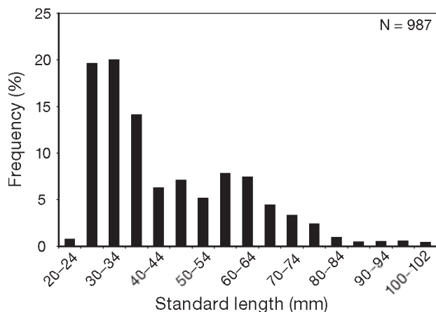
Fig. 3. Electrona antarctica . Length–frequency distribution of postlarvae. The percentage of the total number of fish is shown for each 5 mm length class
