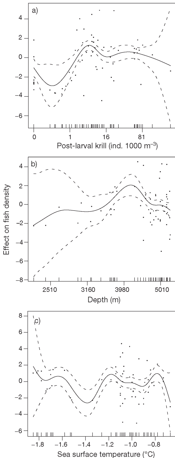
Fig. 4. Electrona antarctica . Generalized additive model of the numerical density of postlarvae. Effect of additive smoothing functions of (a) postlarval Euphausia superba abundance, (b) ocean depth and (c) surface sea temperature on the fitted density of fish. Dashed lines show 95% confidence intervals of smoothers
