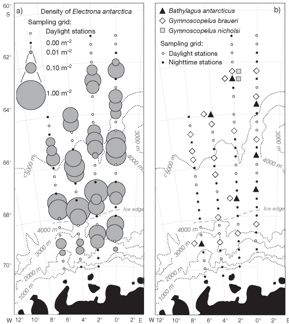
Fig. 2. Spatial distribution of postlarval fishes (polar stereographic projection). (a) Individual density of Electrona antarctica (daylight stations excluded from analysis) and (b) stations where Bathylagus antarcticus , Gymnoscopelus braueri and Gymnoscopelus nicholsi were caught (all stations included)
