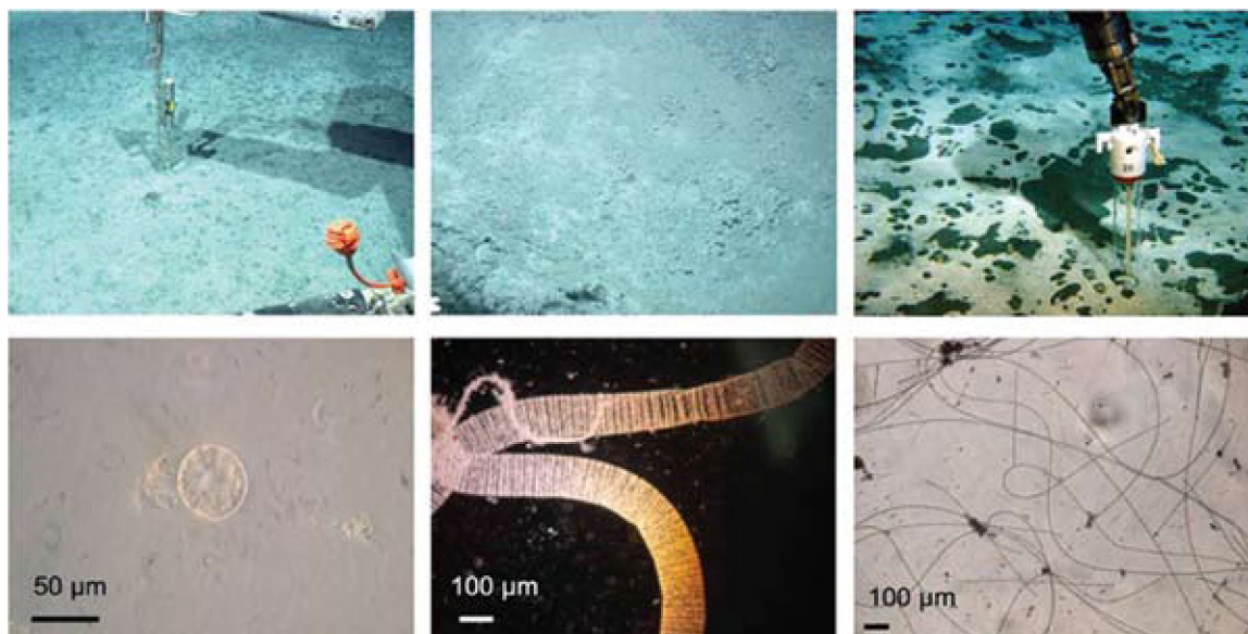
Figure 9. Macroscopic and microscopic images of microbial mats at cold seep ecosystems. (Upper panel, left) Thiomargarita mat in a fault surrounding the Amon mud volcano. ©MARUM/MPI. (Middle) Thin filamentous mats at the center of the Amon mud volcano. ©MARUM/MPI (Right) Thick filamentous mats surrounding the center of the Håkon Mosby mud volcano. ©Ifremer/AWI. The micrographs in the lower panel show the respective mat-forming thiotrophic bacteria. (Left) Sphere-like vacuolate Thiomargarita cell. (Middle) Giant filamentous vacuolate gammaproteobacteria. (Right) Thin filamentous vacuolate Beggiatoa cells. ©Stefanie Grünke, MPI/AWI
