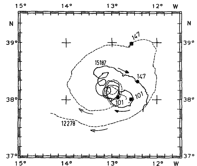
FIG. 7. Trajectories of two surface drifters, 12278 (dashed line, year days denoted by small boxes) and 15187 (solid line, year days denoted by dots) launched on the first cruise leg to relocate meddy.
