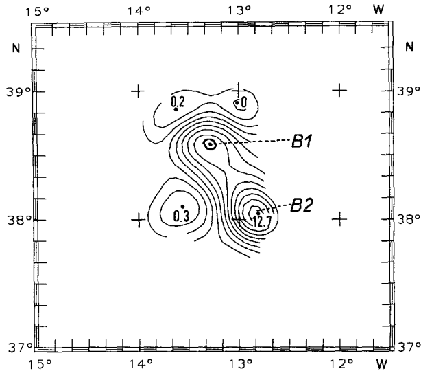
FIG. 6. Geostrophic streamfunction for the MW layer (500–1500 dbar) during the second visit to Aska. Contour interval is 1 \text{ m}^4 \text{ s}^{-1} referenced to 3000 dbar.
