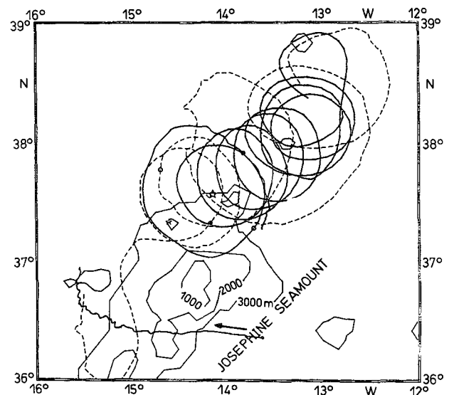
FIG. 14. Anticyclonic trajectories of R10 (solid line) and surface drifter 12275 (dotted line) overlaid on bottom contours. Open circles mark position of each on year day 225, while the open star marks the position of the meddy center on that day, the day on which R10 left the meddy. Closed circles and star mark year day 250, the day the surface drifter was expelled. The continuation after a gap within the RAFOS float trajectory is indicated by the arrow.
