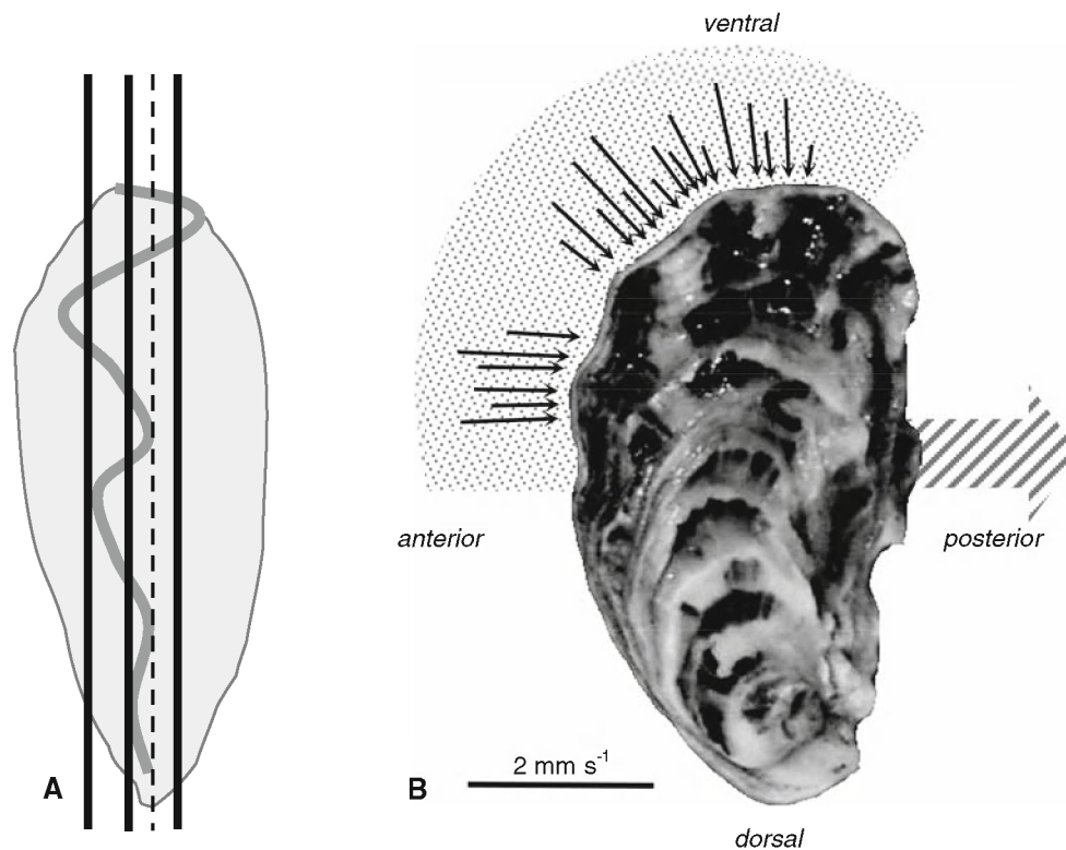
Fig. 1 Indication of the different laser sheet projections (a) used to determine the area of in- and outflow in C. gigas (b). a The frontal view of an oyster, showing both valves and undulating shell edges. The dashed line indicates the sagittal plane. Different projections of the laser-sheet, parallel to the sagittal plane, are indicated as black lines . b Areas of in- and outflow in a Pacific oyster. The dotted area is
