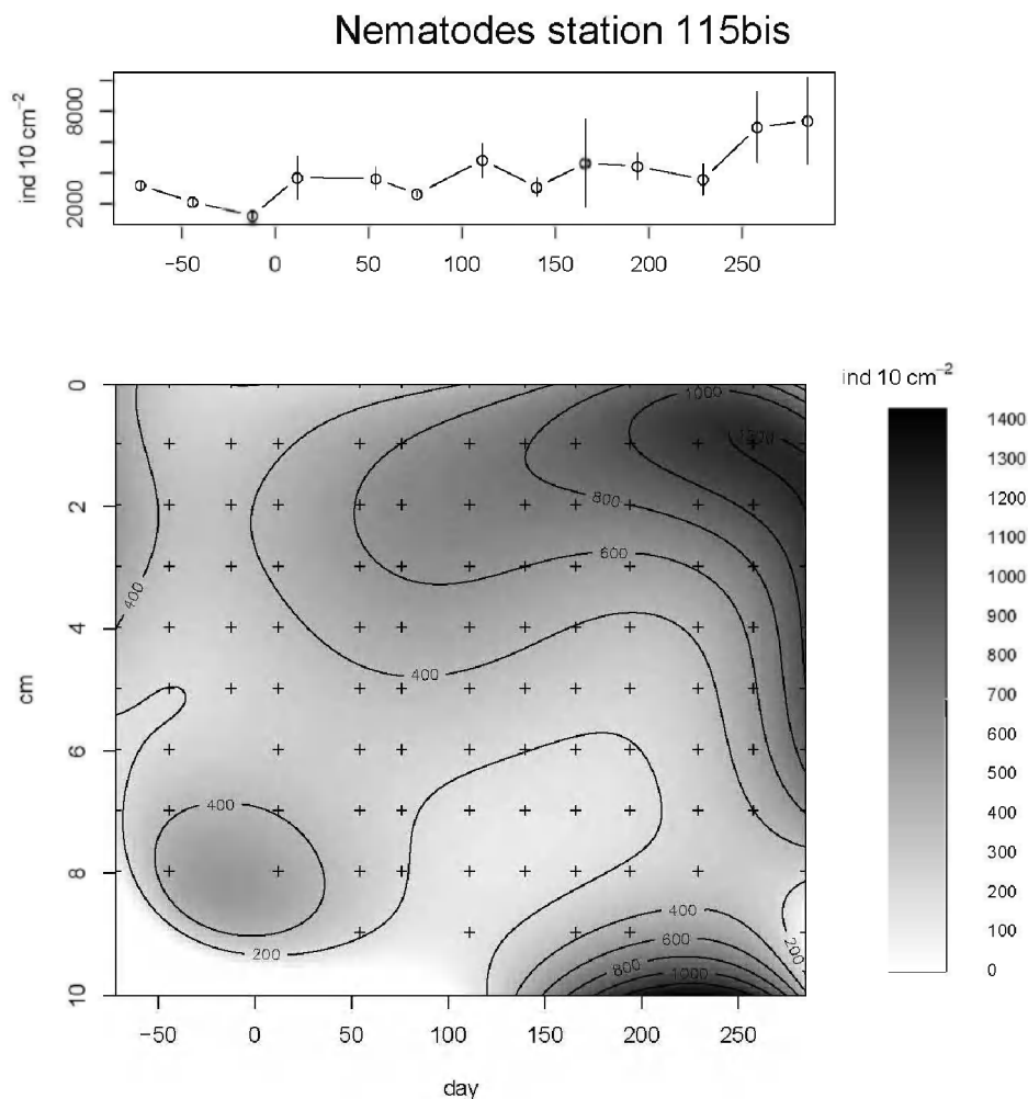
Figure 3.4: Nematode densities ( \text{ind } 10\text{cm}^{-2} ) at station 115bis for the period from October 2002 to October 2003 (day 0 = 1st January 2003) from 0 to 10cm deep. The upper graph shows the nematode densities ( \text{ind } 10\text{cm}^{-2} ) summed over the vertical profile. Vertical bars represent the standard error.
