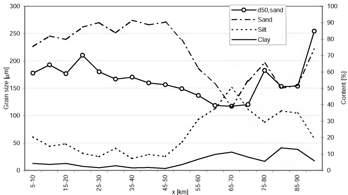
Figure 35. Sediment characteristics of the Scheldt estuary in 1992 (courtesy of van Ledden).
