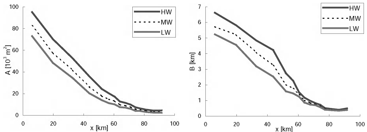
Figure 27. The macro-scale averaged cross section area A and width B , for high water (HW), mean water (MW) and low water (LW), from Vlissingen to Schelle.
