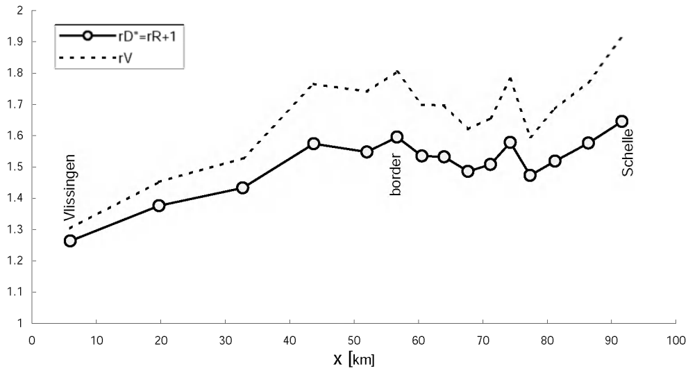
Figure 15. Ratio between tidal range and average depth at low water r_R (for sake of comparison, the related ratio r_D^* is plotted in continuous line with circles), and ratio between volumes at high water and low water r_V (dashed line), along the sections of the Scheldt estuary (from Vlissingen to Schelle).
