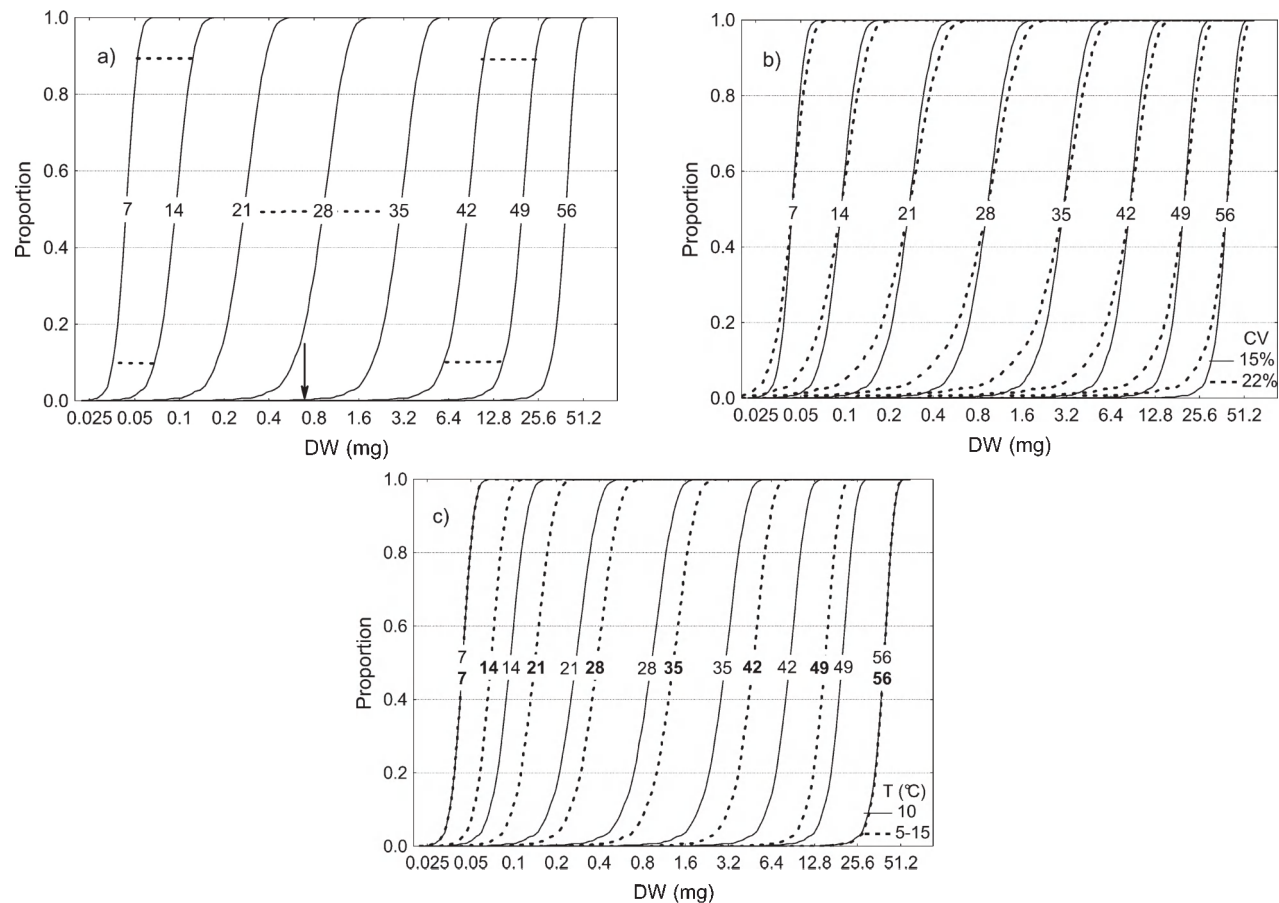
FIG. 3. – Simulated CSDs based on the STDG model by Folkvord (2005); 1000 individuals with average DW_7 = 0.045 mg and a) initial CV = 15% and temperature = 10^\circ\text{C} . Horizontal dashed lines represent approximate growth for different parts of the cohort between weekly samplings, the arrow indicates size of maximum growth potential (Folkvord 2005), b) as left with initial CV = 22% (dashed line), c) temperature linearly increasing from 5 to 15^\circ\text{C} (dashed line). CSDs in a) shown by solid line in b) and c) for comparison. Numbers on CSDs represent larval age (dph).
