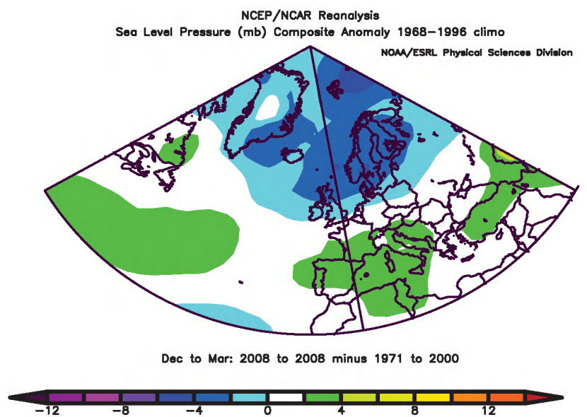
Figure 10. Winter (DJFM) sea level pressure (SLP) fields. Top panel: SLP averaged over 30 years (1971–2000). Middle panel: mean SLP in winter 2008 (December 2007, January–March 2008). Bottom panel: winter 2008 SLP anomaly – the difference between the top and middle panels. Images provided by the NOAA/ESRL Physical Sciences Division, Boulder, Colorado (available online at http://www.cdc.noaa.gov/ ).
