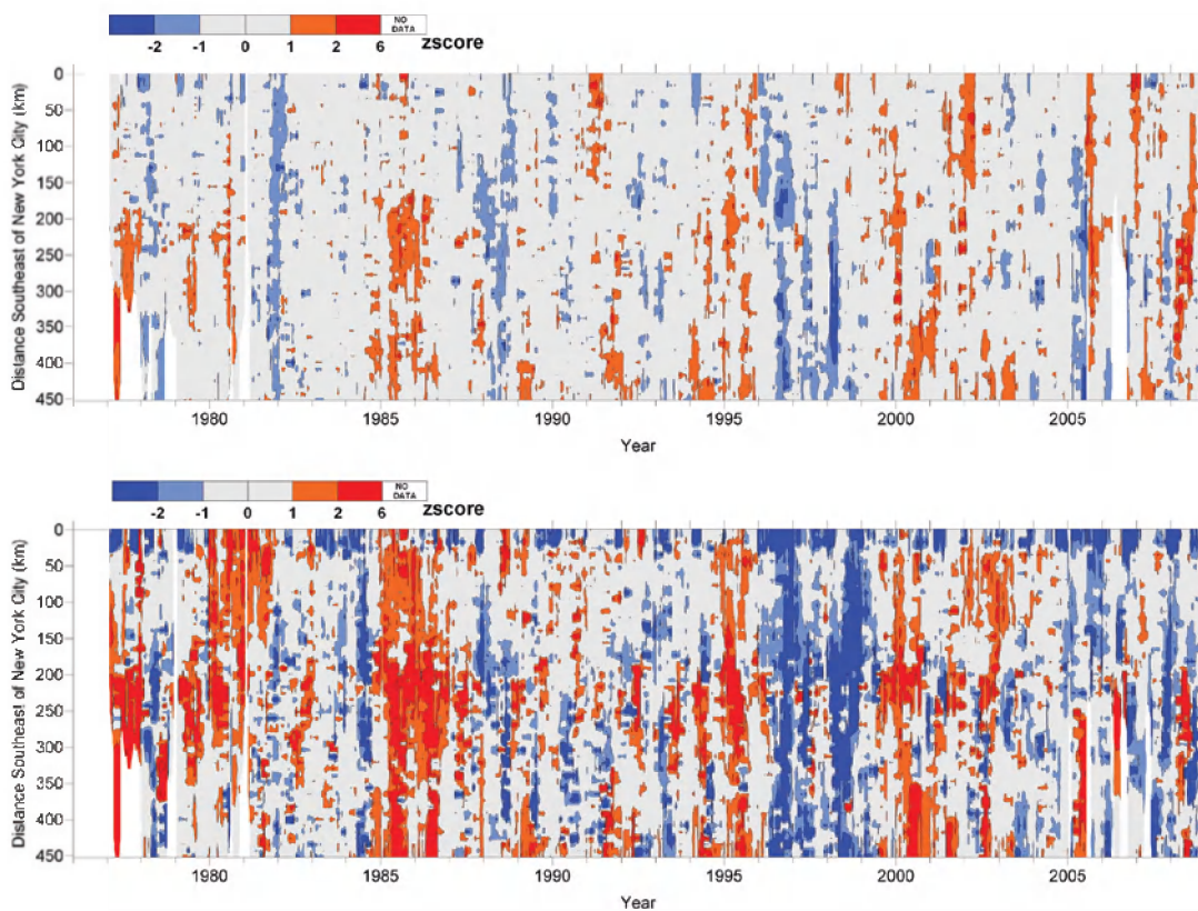
Figure 27. Area 2c – Mid-Atlantic Bight. Temperature and salinity in the central Mid-Atlantic Bight. Top panel: surface temperature anomaly (relative to the base period of 1978–2007) from XBT measurements. The origin of the line is New York City. Bottom panel: sea surface salinity anomalies from bottle measurements. Data provider: Woods Hole Oceanographic Institution, USA.
