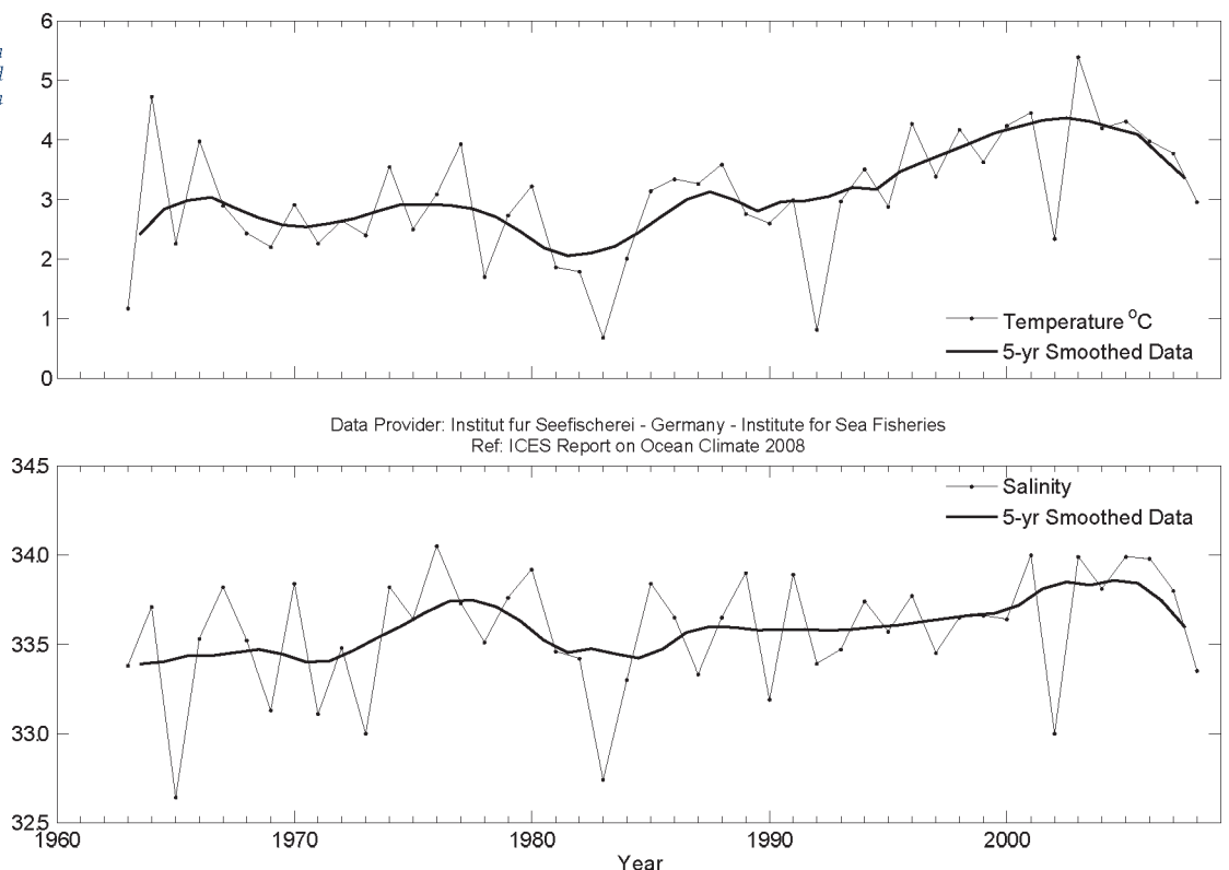
Figure 15. West Greenland. Autumn temperature (upper panel) and salinity (lower panel) at 0–200 m at Fyllas Bank Station 4.
