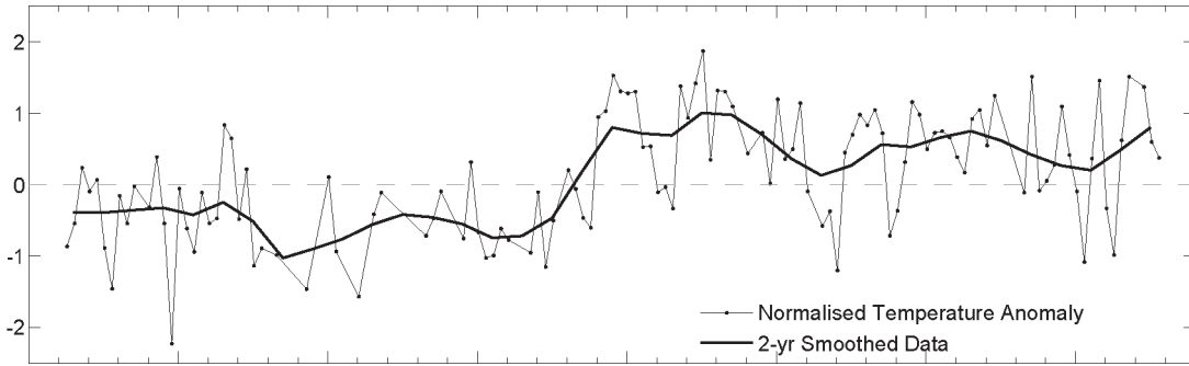
Figure 55. Area 9 – Southern North Sea. Normalized sea surface temperature anomaly (upper panel) and salinity anomaly (lower panel) relative to 1971–2000, measured along 52°N by a regular ferry at six standard stations. The time-series reveals the seasonal section average (DJF, MAM, JJA, SON) of the normalized variable..
