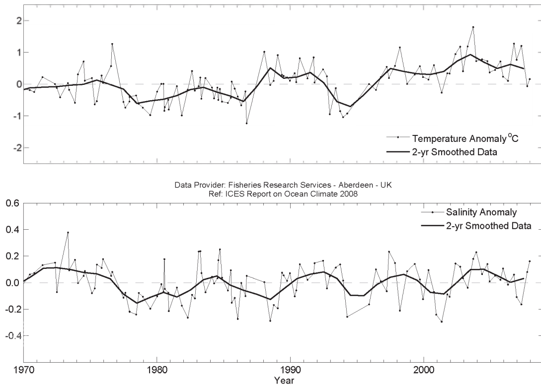
Figure 52. Area 8 – Northern North Sea. Temperature anomaly (upper panel) and salinity anomaly (lower panel) in the Fair Isle Current entering the North Sea from the North Atlantic.
