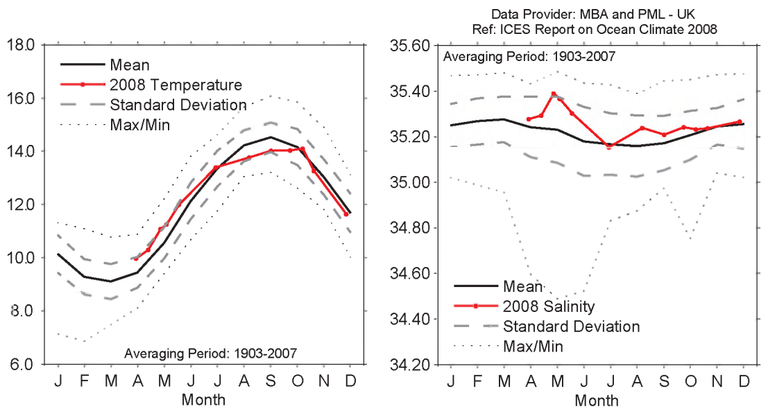
Figure 40. Area 4b – Northwest European continental shelf. 2008 monthly temperature (left panel) and salinity (right panel) of surface water at Station E1 in the western English Channel (50.03°N 4.37°W).
