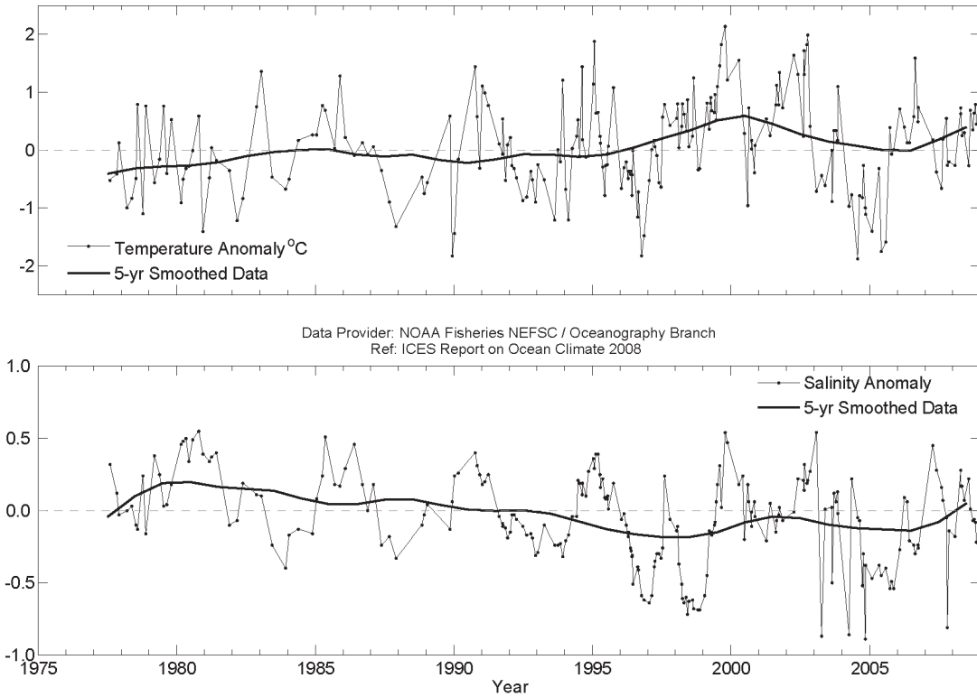
Figure 29. Area 2c – Mid-Atlantic Bight. Time-series plots of 0–30 m averaged temperature anomaly (top panel) and salinity anomaly (bottom panel) at Georges Bank.
