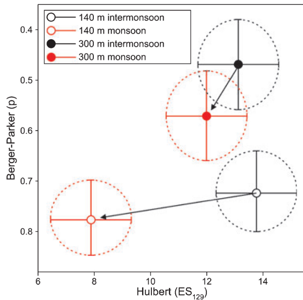
Fig. 5. Foraminifera (Rose-Bengal-stained, >300\text{-}\mu\text{m} fraction) from 140 and 300 m (monsoon and intermonsoon seasons) on the Pakistan margin. Joint plot of Berger-Parker Index (Rank 1 dominance) and rarefied species richness (Hulbert), showing 95% confidence limits. Data from Larkin & Gooday (2009).
