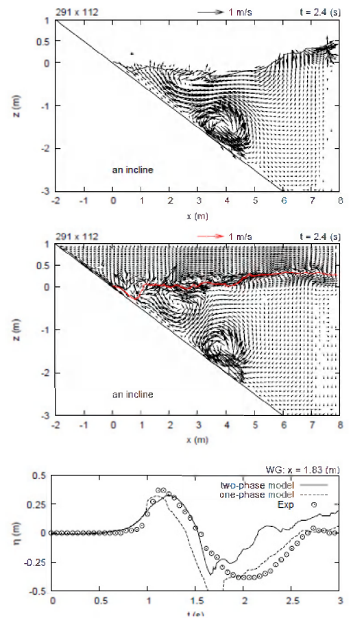
Fig. 4. Comparison of the one- and two-phase models over grid (291 × 112) for impulsive waves caused by the landslide.
