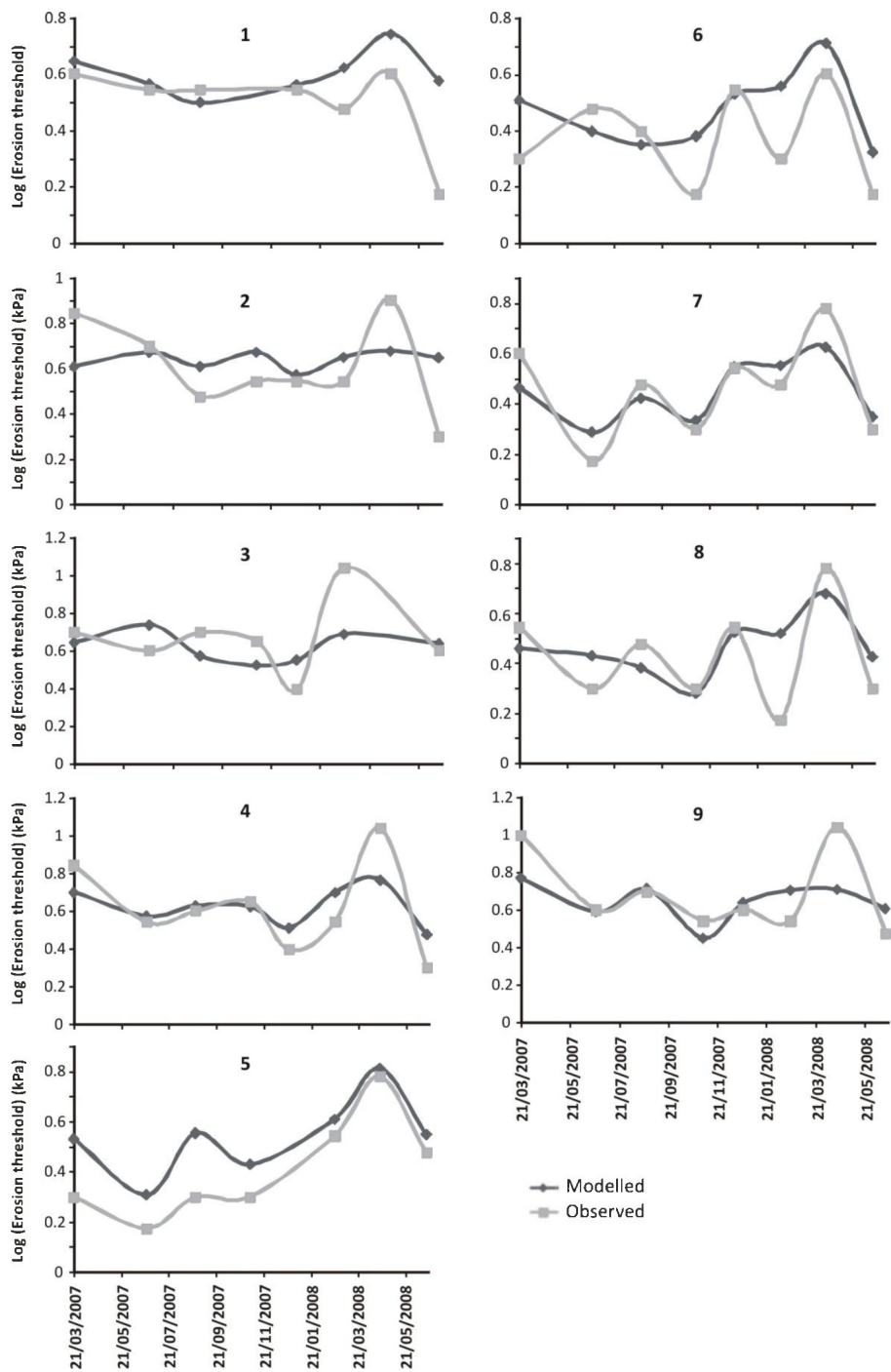
Figure 6: Modelled versus observed values for Log(erodion threshold) from March 2007 onwards.
