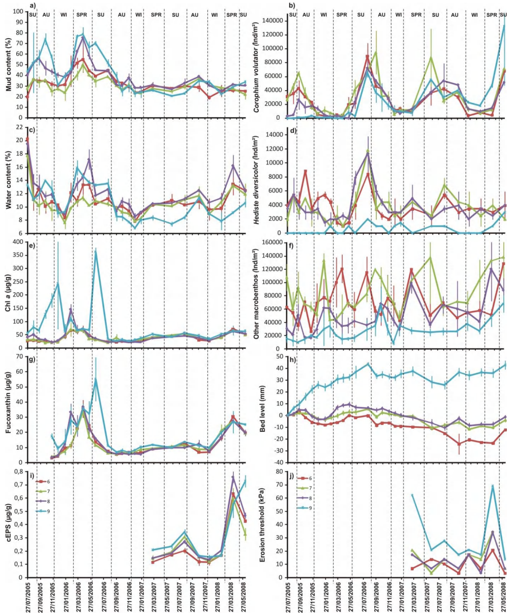
Figure 4: Temporal distribution of mean \pm SE from a) mud content (%), b) Corophium density (ind./m 2 ), c) water content (%), d) Hediste density (ind./m 2 ), e) chl a (µg/g), f) other macrobenthos density (ind./m 2 ), g) fucoxanthin (µg/g), h) bed level (mm), i) colloidal EPS (µg/g) and j) erosion threshold (kPa), for plots 6 to 9 with indication of the seasons. Note the scale differences for mud content, chl a , bed level, cEPS and erosion threshold in comparison with Fig. 3.
