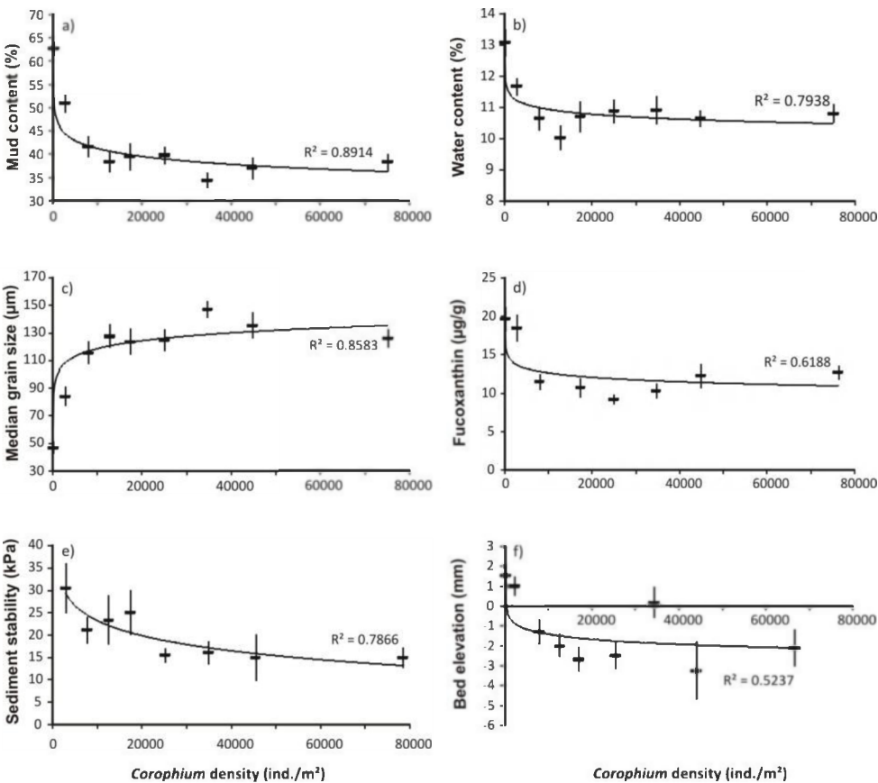
Figure 1 a - f: Relationships between density classes of Corophium volutator and biophysical parameters of the sediment, (a) mud content, (b) water content, (c) median grain size, (d) fucoxanthin concentration, (e) sediment stability and (f) erosion/accretion measured as bed level changes between successive surveys. Data points indicate averages±SE of the available data per density class collected during the field survey presented in Chapter 6.
