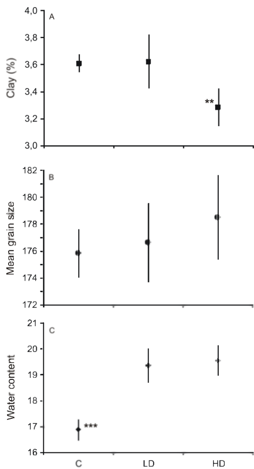
Figure 3: (A) Average percentage of clay (B) average mean grain size and (C) average water content (in %) for the different treatments ( n=5 \pm \text{S.D.} ) (C = Control, LD = Low Density, HD = High Density), * * and *** indicate significance levels of Tukey's Post Hoc
