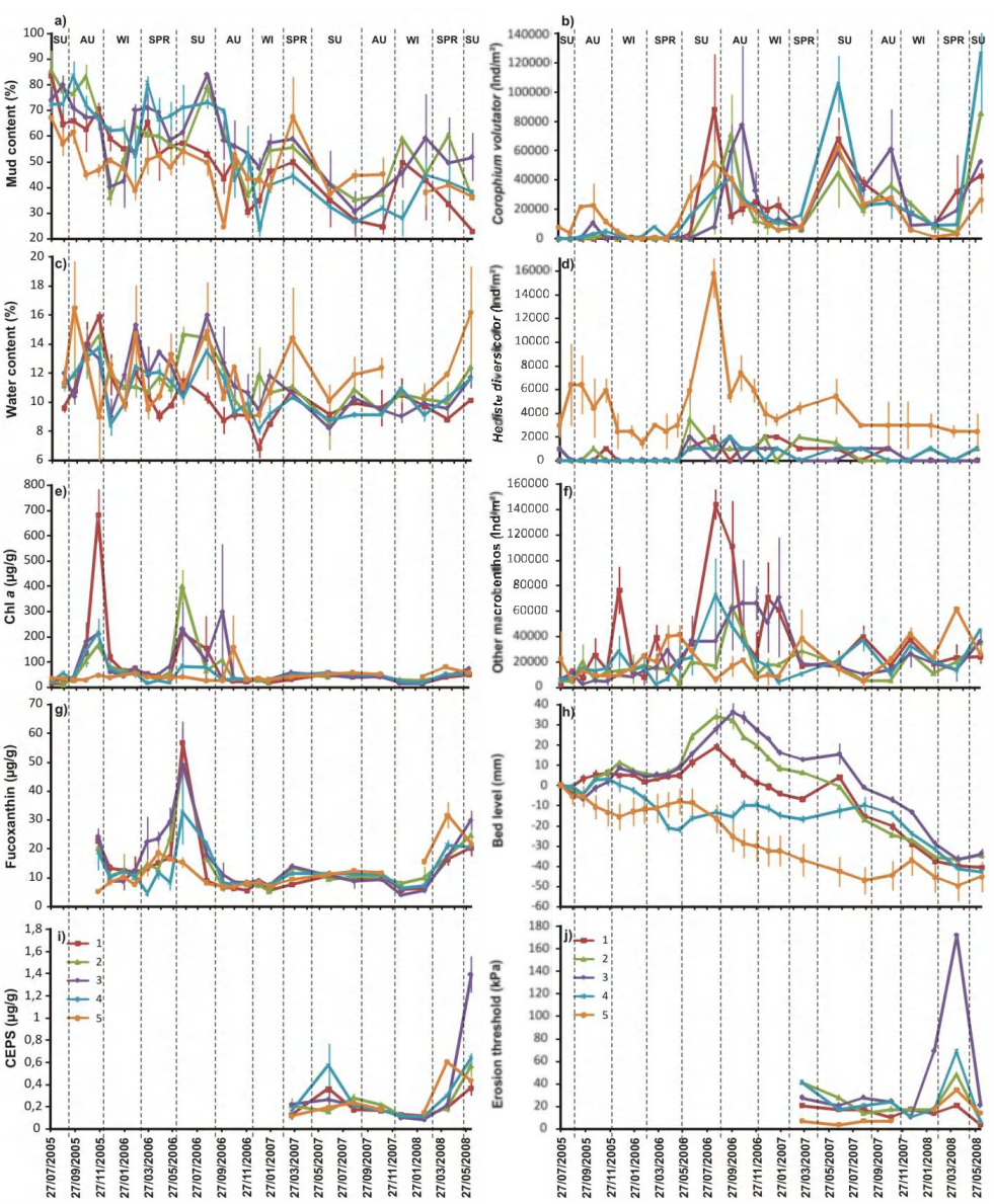
Figure 3: Temporal distribution of mean \pm SE from a) mud content (%), b) Corophium density (ind./m 2 ), c) water content (%), d) Hediste density (ind./m 2 ), e) chl a ( \mu g/g), f) other macrobenthos density (ind./m 2 ), g) fucoxanthin ( \mu g/g), h) bed level (mm), i) colloidal EPS ( \mu g/g) and j) erosion threshold (kPa), for plots 1 to 5 with indication of the seasons. Note the scale differences for mud content, chl a, bed level, cEPS and erosion threshold in comparison with Fig. 4.
