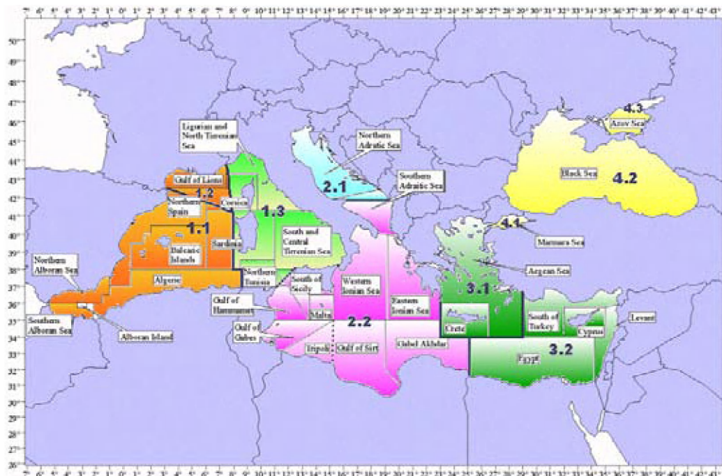
Figure 7: GFCM Geographical Areas
