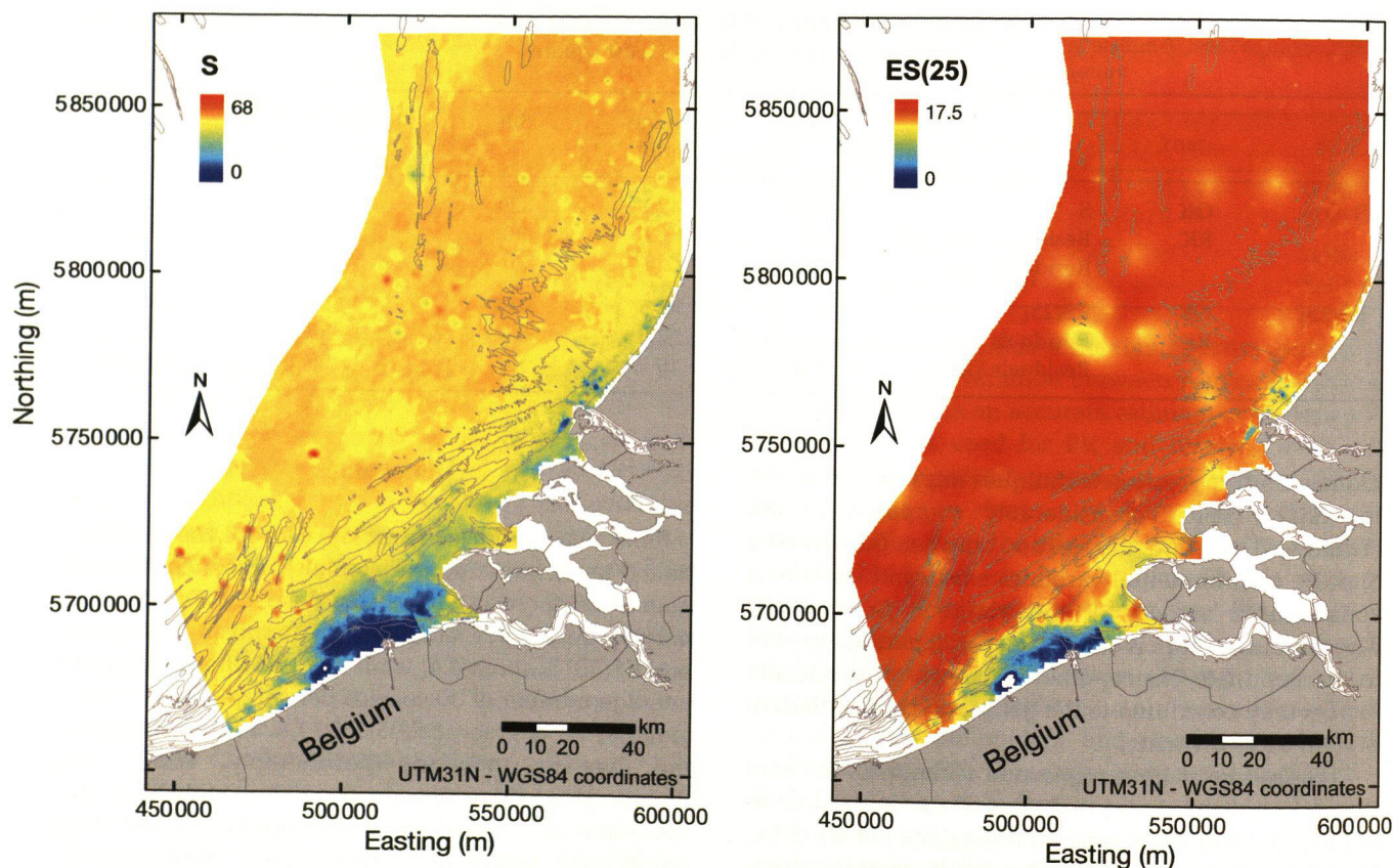
Fig. 4. Maps of the generalised least squares models, predicting the nematode diversity after kriging of diversity indices S (left) and ES(25) (right). Grey lines in water are bathymetric lines. See Table 1 for definitions
