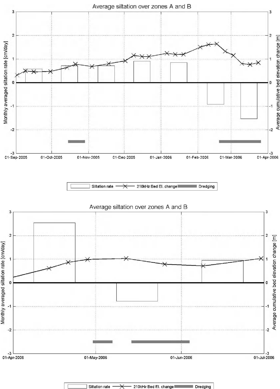
Figure 5-1: Monthly averaged siltation rate [cm/day] for first period (reference 4 August 2005) and second period (reference 24 March 2006)
