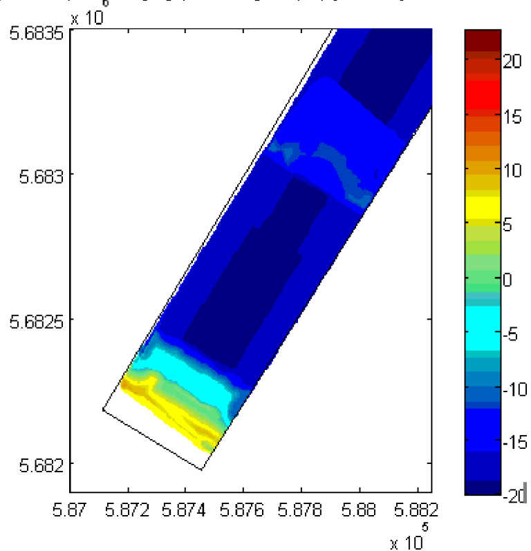
Depth of capital dredging (and design depth) [m TAW]: 08-Feb-2008
