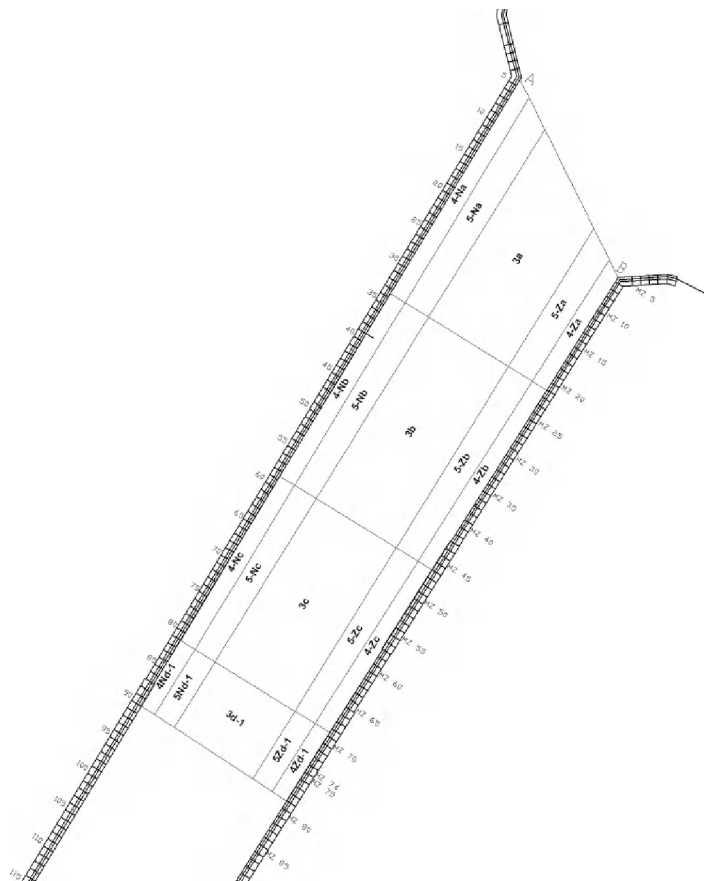
Figure 4-13: Operational part of Deurganckdok at the start of the 3 rd phase of capital dredging works (Feb. 2007)
